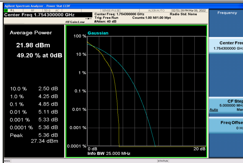
Band4-1.4MHz-64QAM-20393-1RB#0
