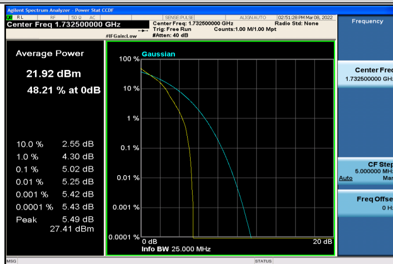
Band4-1.4MHz-64QAM-20175-1RB#0
