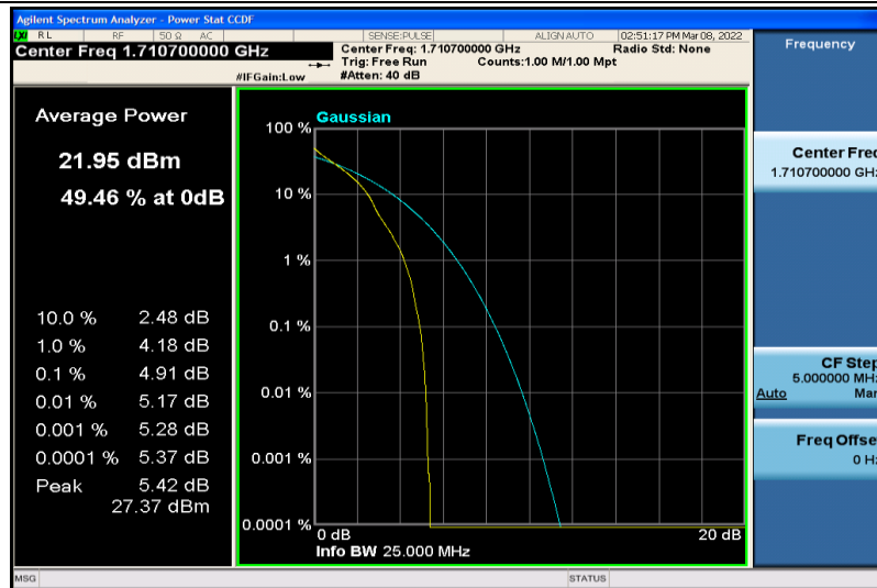
Band4-1.4MHz-64QAM-19957-1RB#0
