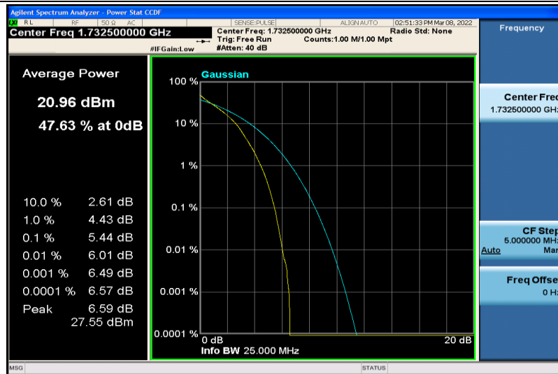
Band4-1.4MHz-64QAM-20175-6RB#0
