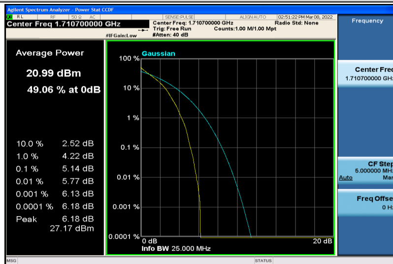
Band4-1.4MHz-64QAM-19957-6RB#0
