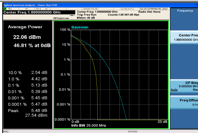
Band2-10MHz-64QAM-18900-1RB#0
