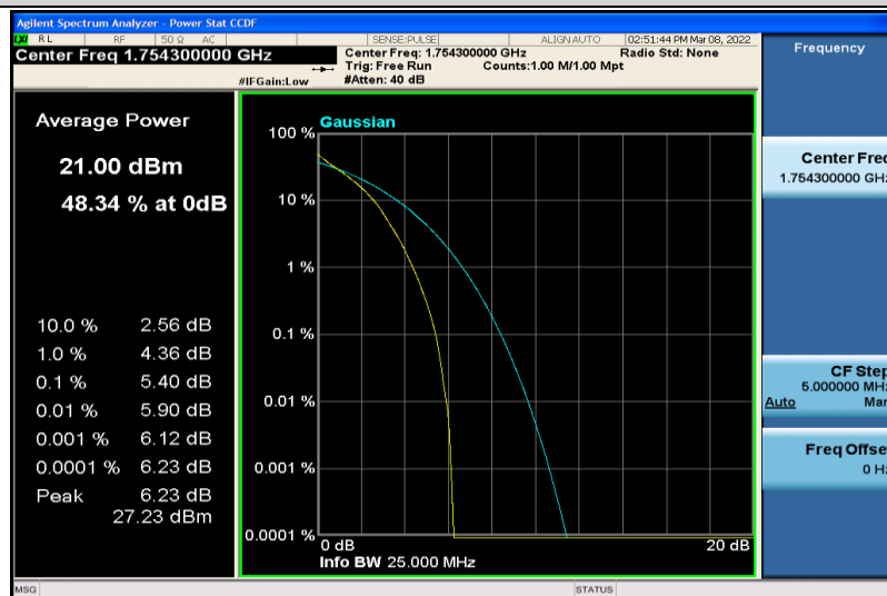
Band4-1.4MHz-64QAM-20393-6RB#0
