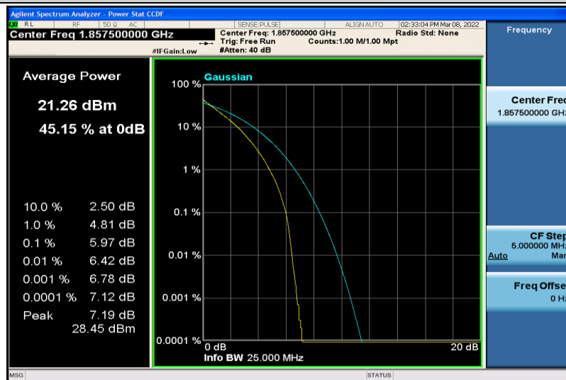
Band2-15MHz-64QAM-18675-5RB#0
