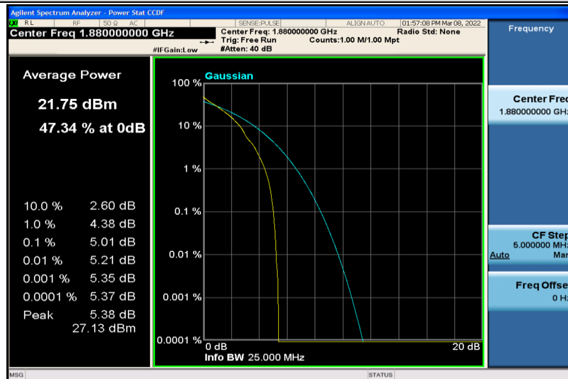
Band2-1.4MHz-64QAM-18900-1RB#0
