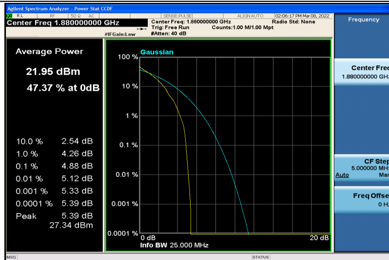
Band2-3MHz-64QAM-18900-1RB#0
