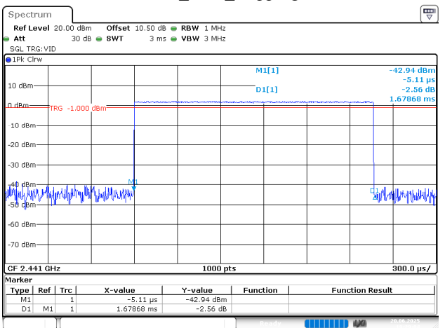
BDR_DH3_Hopping
