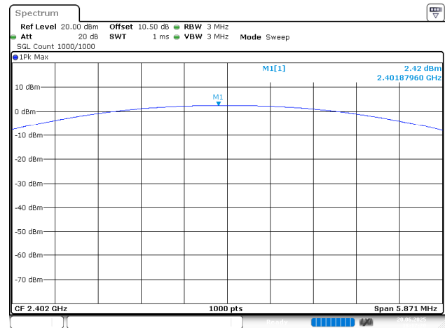
3EDR_DH1_Low
