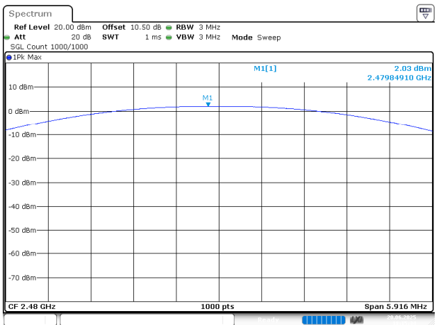
2EDR_DH1_High
