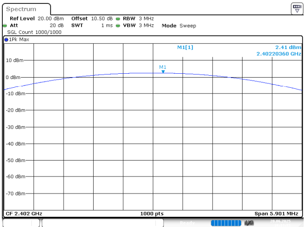
2EDR_DH1_Low
