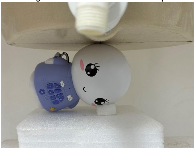
Fig-4.4 Test Position 4 with 0 cm Gap
