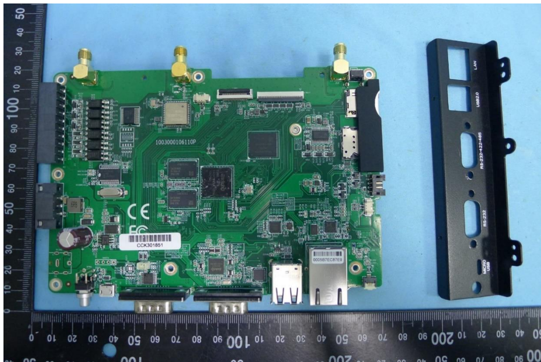
(7) EUT Photo
