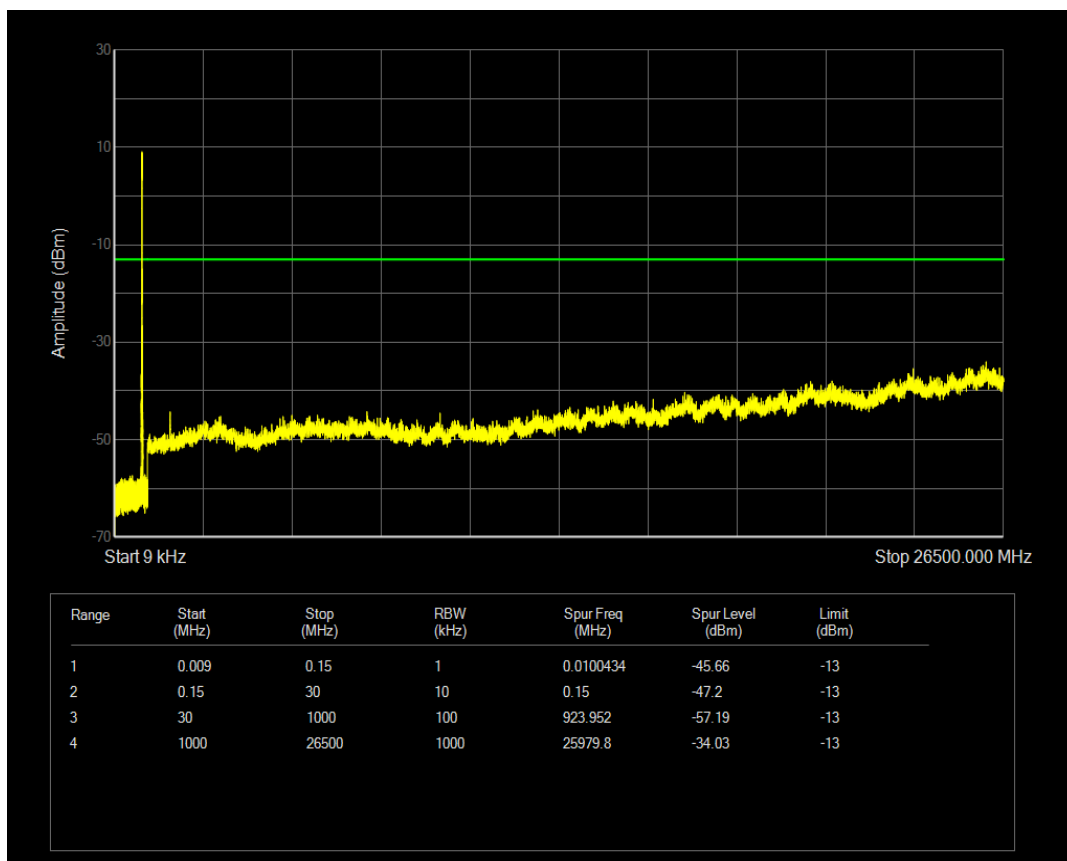
Band19 QAM16 BW=15MHz Channel=24075 RB Size=75 Position=#0
