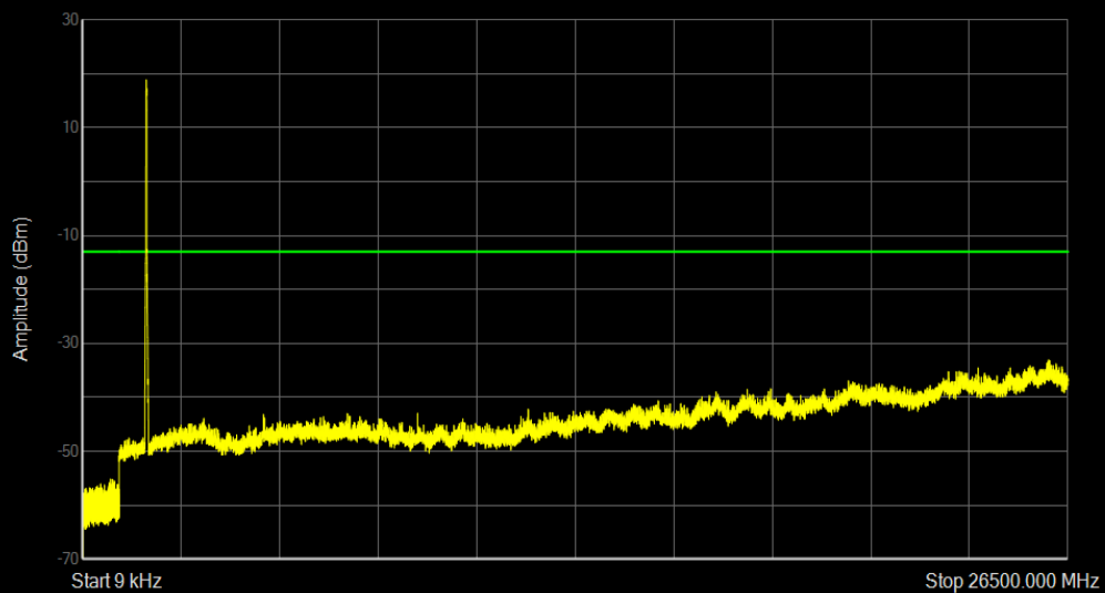
Band4 QAM16 BW=20MHz Channel=20175 RB Size=100 Position=#0
