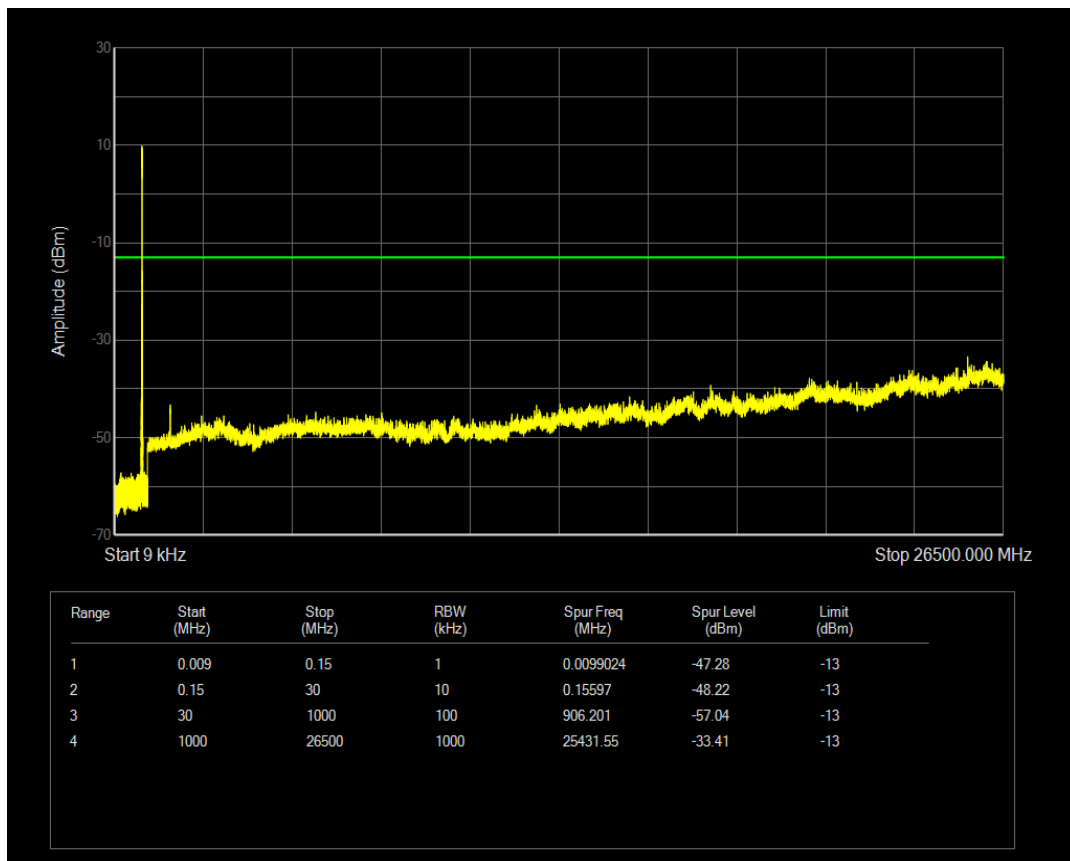
Band19 QAM16 BW=15MHz Channel=24075 RB Size=1 Position=#0
