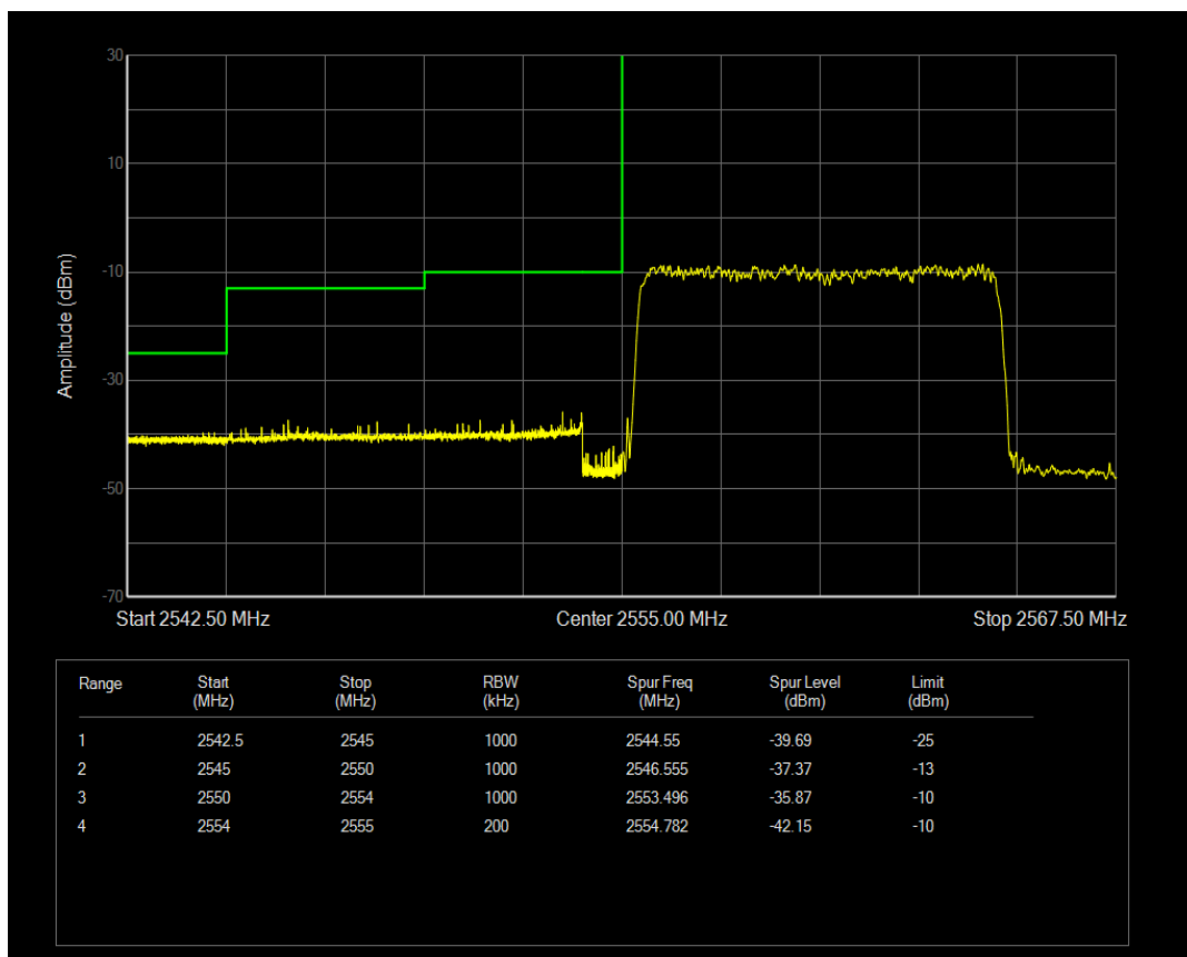
Band41 QAM16 BW=10MHz Channel=40290 RB Size=1 Position=#Max
