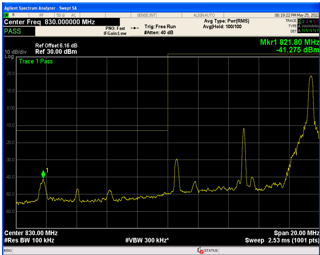
Band19 QPSK BW=10MHz Channel=24050 RB Size=50 Position=#0
