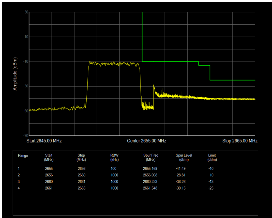
Band41 QAM16 BW=5MHz Channel=41215 RB Size=1 Position=#Max
