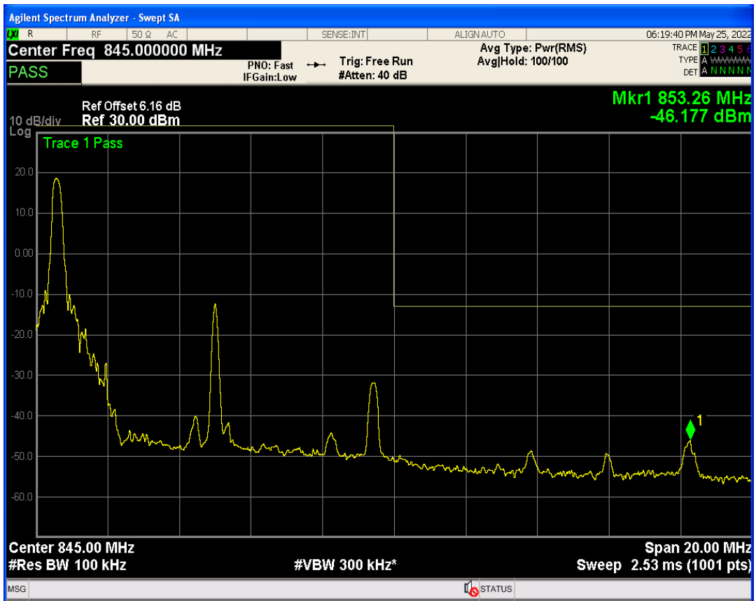
Band19 QAM16 BW=10MHz Channel=24050 RB Size=50 Position=#0
