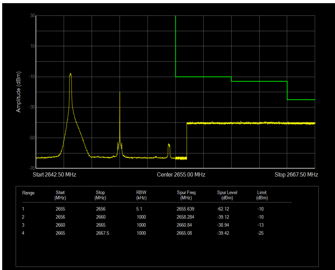
Band41 QPSK BW=10MHz Channel=41190 RB Size=1 Position=#Max
