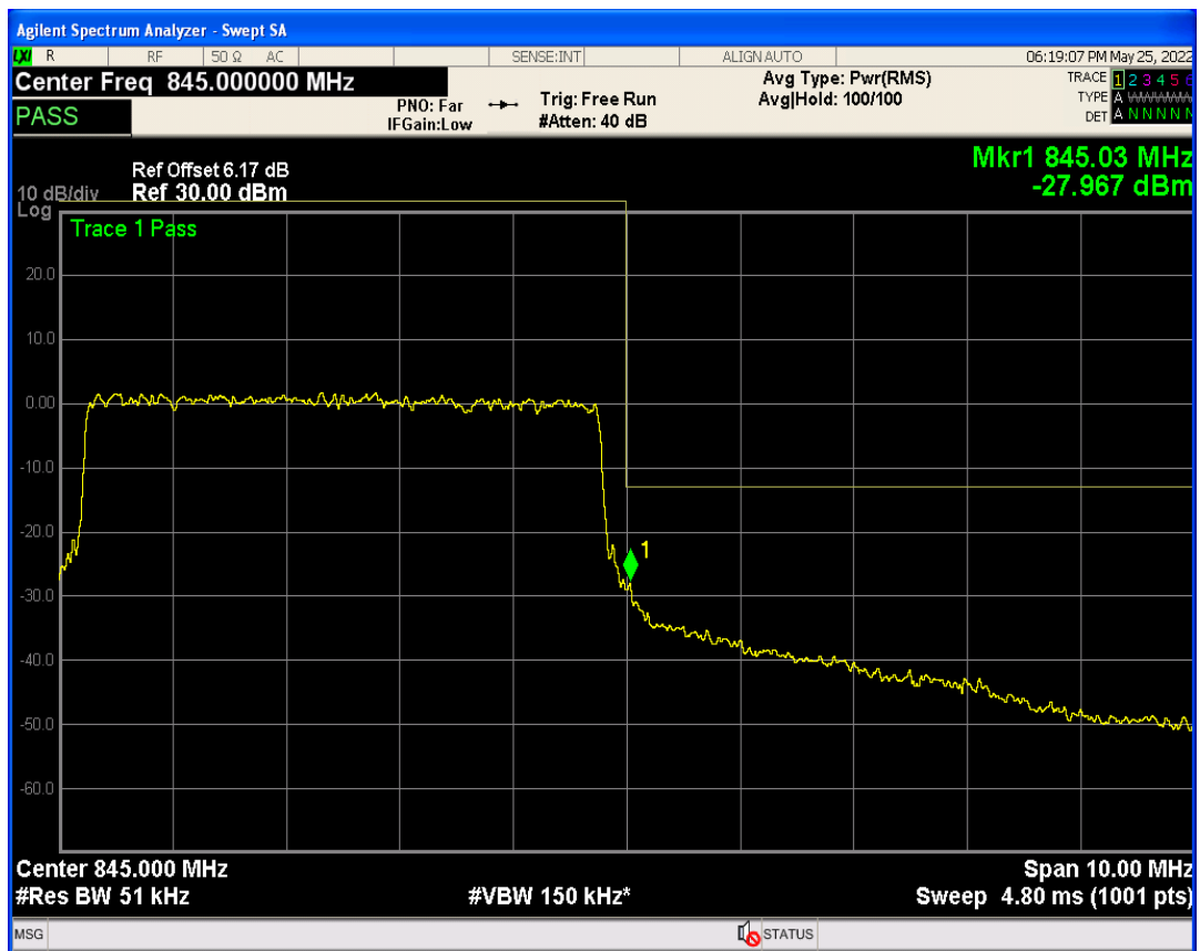
Band19 QPSK BW=10MHz Channel=24050 RB Size=1 Position=#Max
