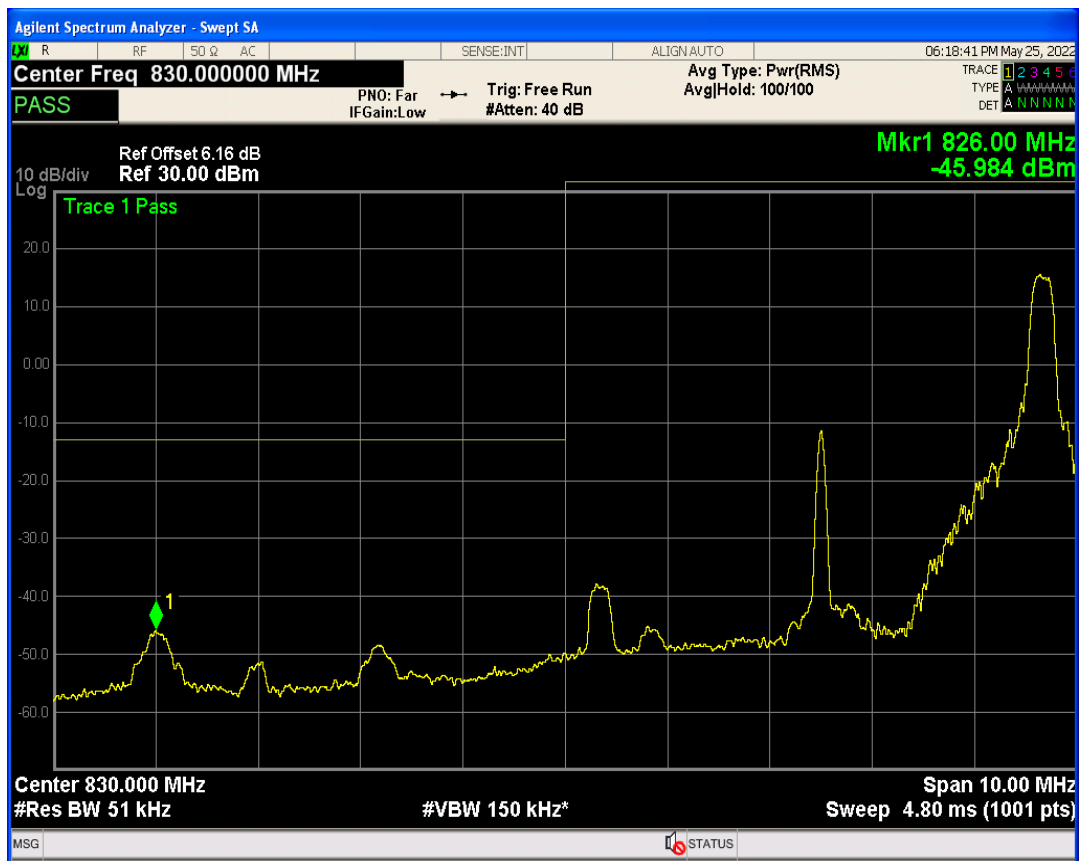
Band19 QAM16 BW=5MHz Channel=24025 RB Size=1 Position=#0
