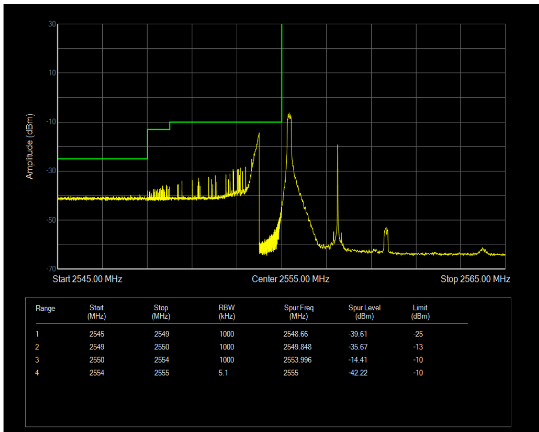
Band41 QPSK BW=5MHz Channel=40265 RB Size=1 Position=#Max
