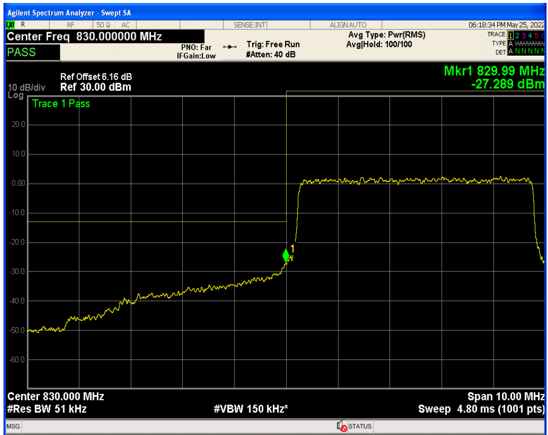
Band19 QPSK BW=5MHz Channel=24025 RB Size=1 Position=#Max
