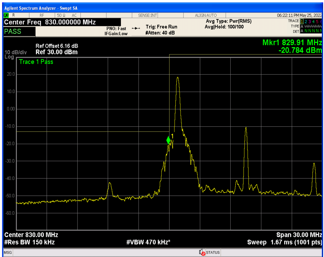
Band19 QAM16 BW=15MHz Channel=24075 RB Size=75 Position=#0
