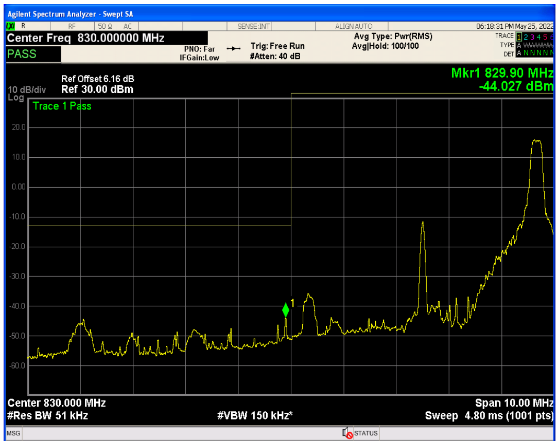
Band19 QAM16 BW=5MHz Channel=24025 RB Size=1 Position=#Max
