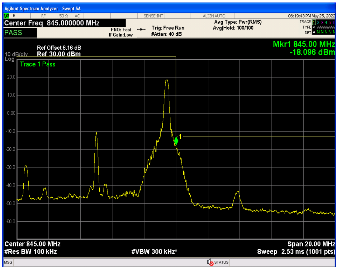
Band19 QAM16 BW=10MHz Channel=24100 RB Size=1 Position=#0
