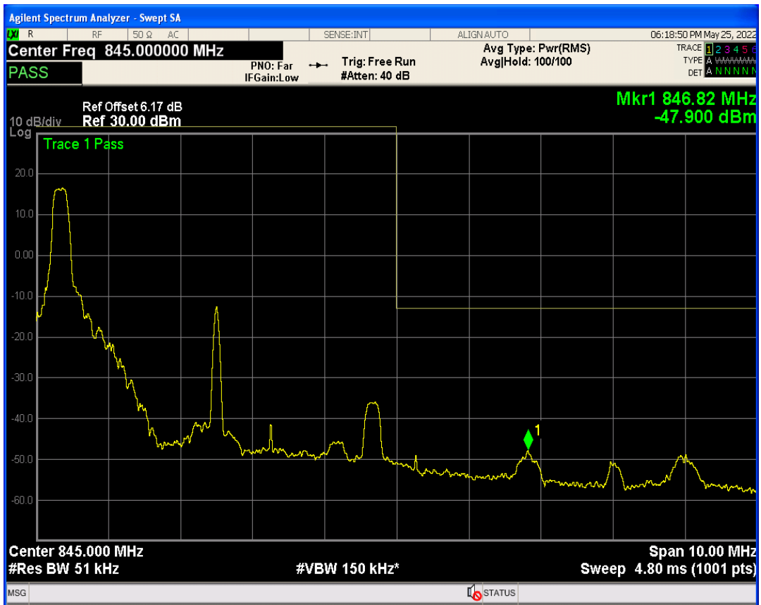
Band19 QPSK BW=5MHz Channel=24125 RB Size=25 Position=#0
