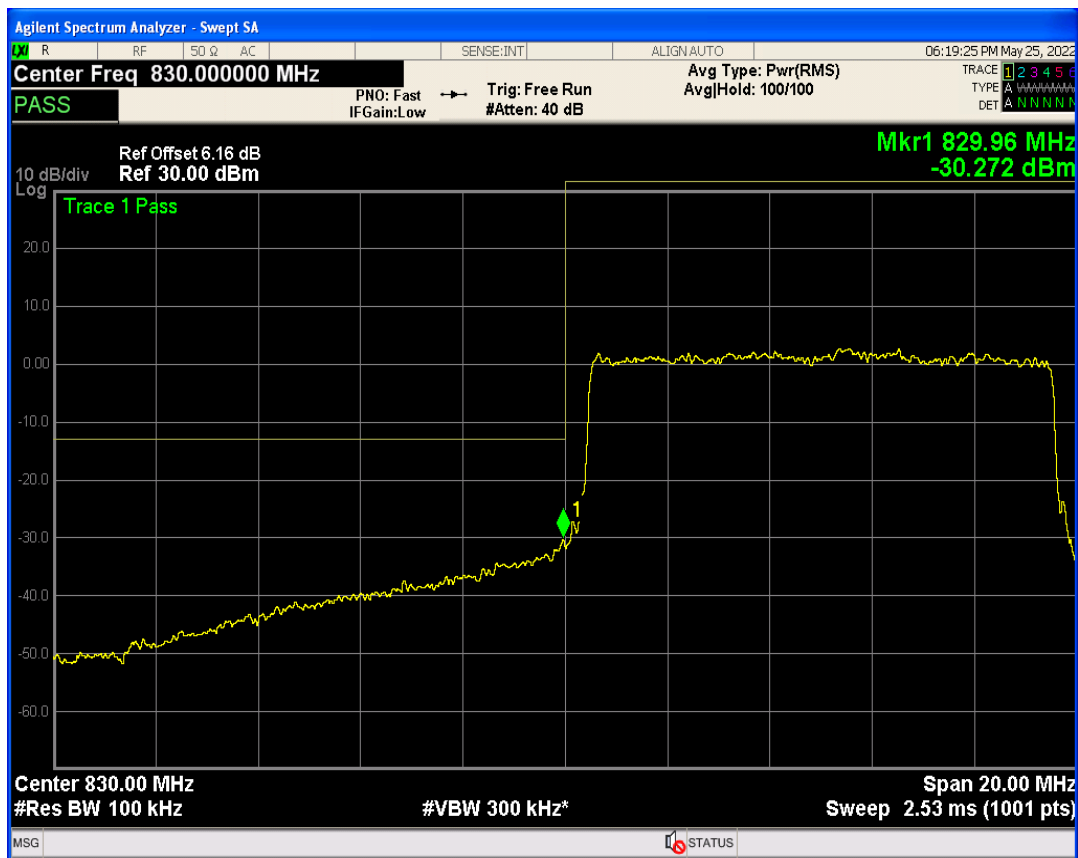
Band19 QAM16 BW=10MHz Channel=24050 RB Size=1 Position=#0
