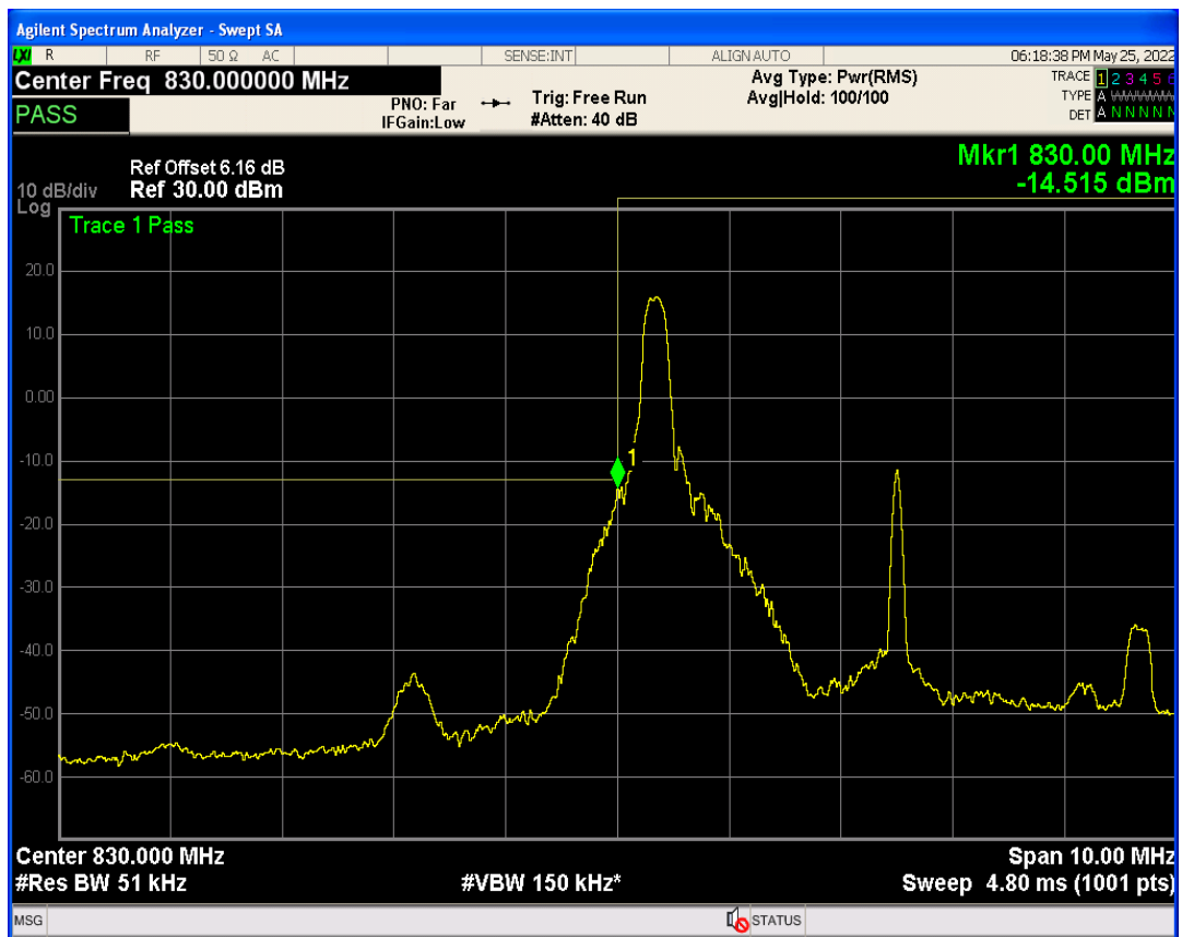
Band19 QAM16 BW=5MHz Channel=24025 RB Size=25 Position=#0
