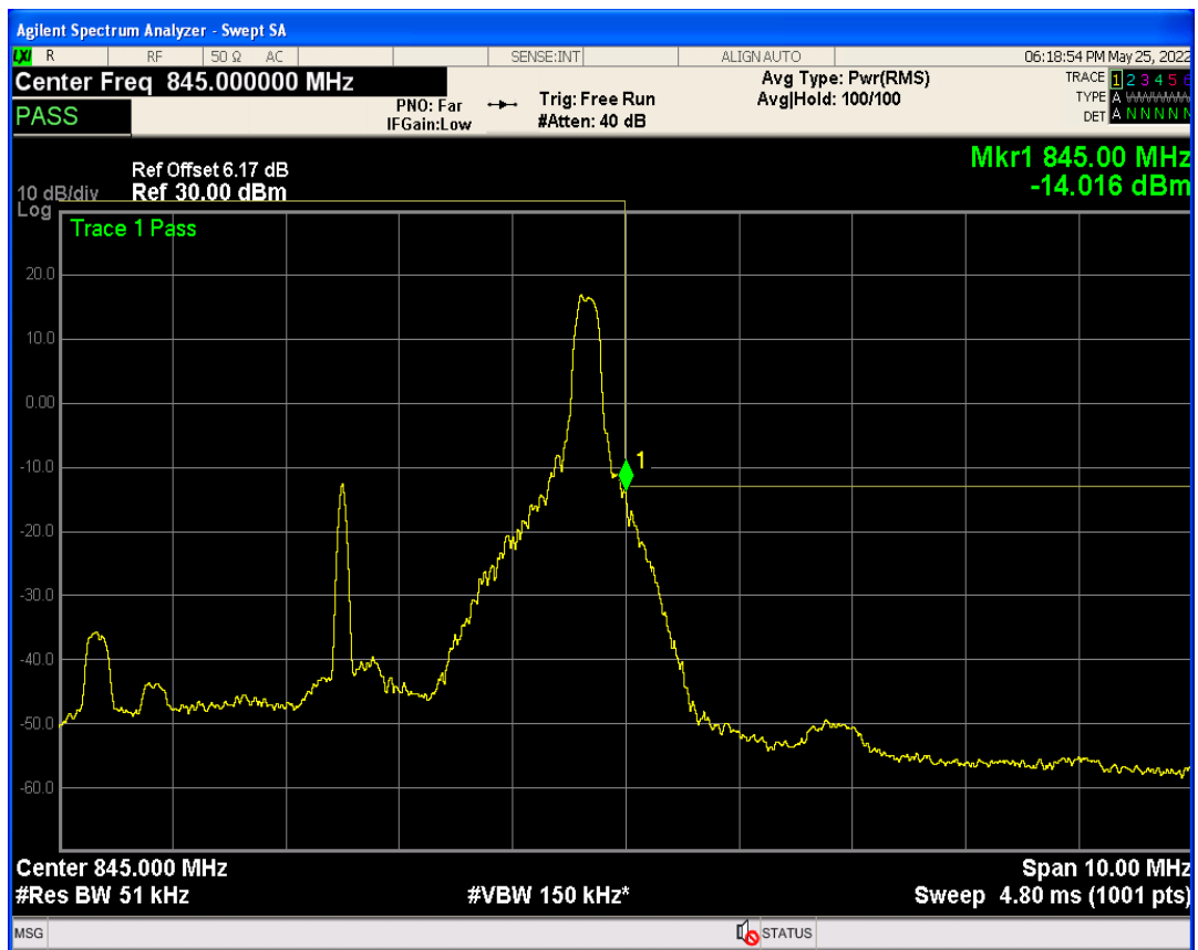
Band19 QPSK BW=5MHz Channel=24125 RB Size=1 Position=#0
