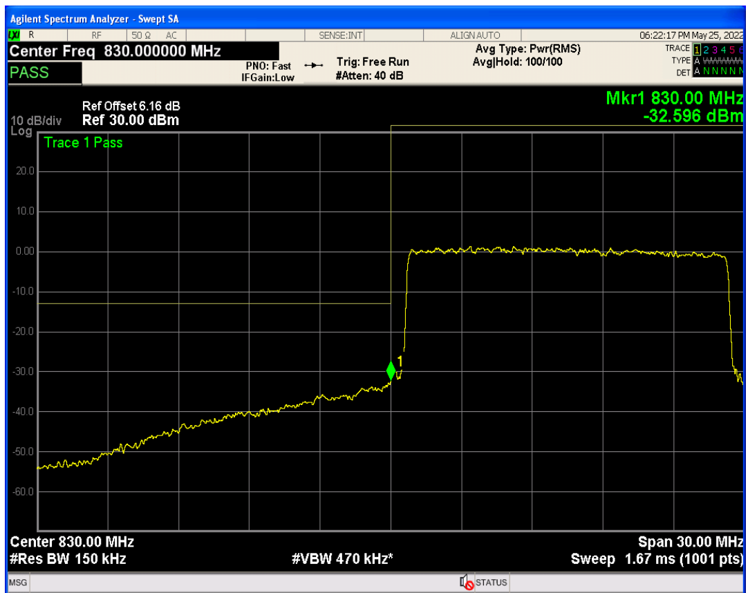
Band19 QAM16 BW=15MHz Channel=24075 RB Size=1 Position=#Max
