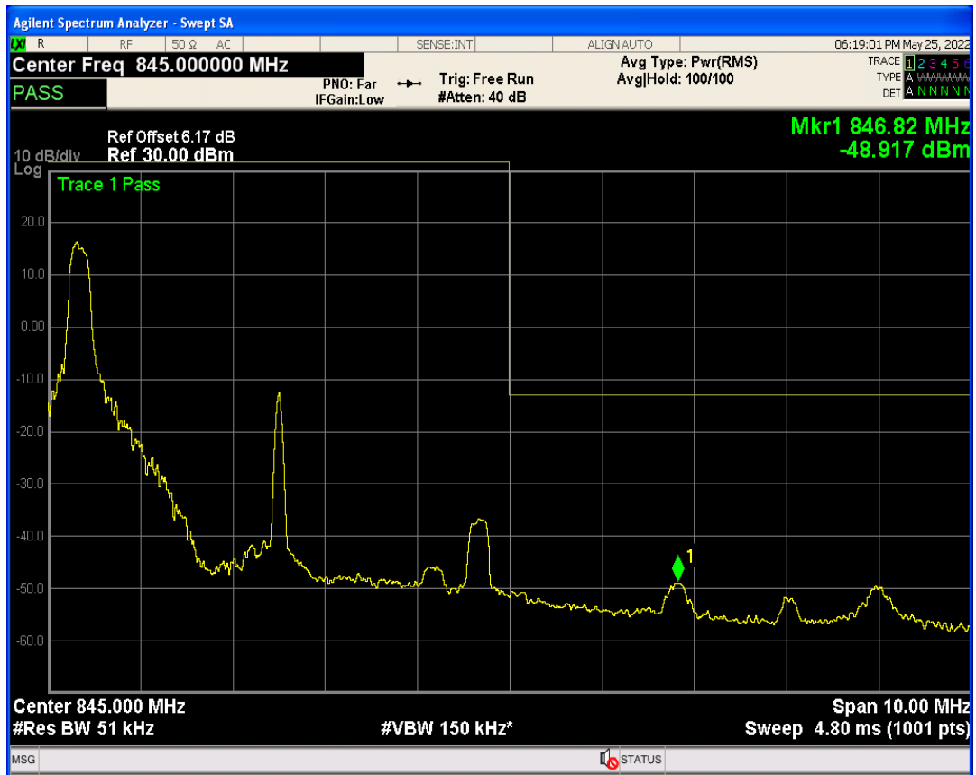
Band19 QAM16 BW=5MHz Channel=24125 RB Size=1 Position=#Max
