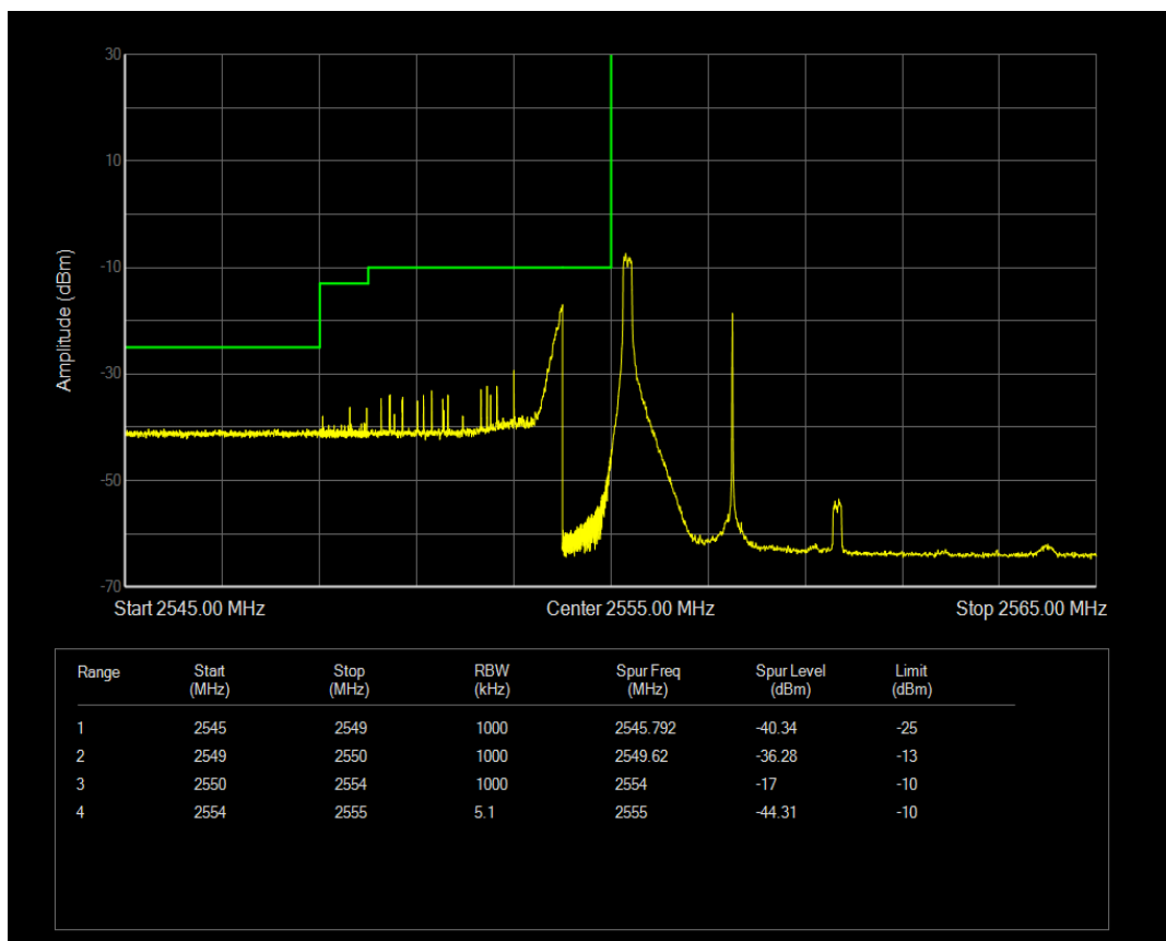
Band41 QAM16 BW=5MHz Channel=40265 RB Size=1 Position=#Max
