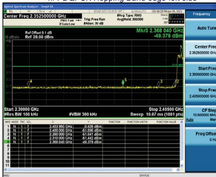
\pi/4 -DQPSK Hopping Band edge-left side
