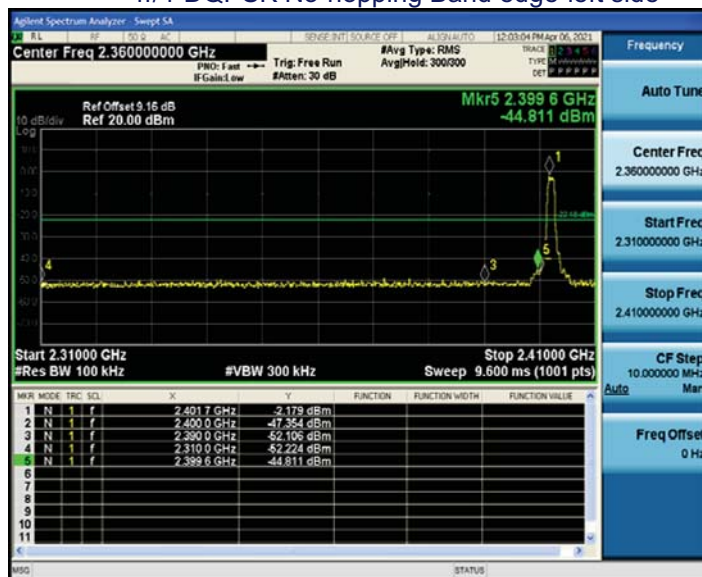
\pi/4 -DQPSK No-hopping Band edge-left side
