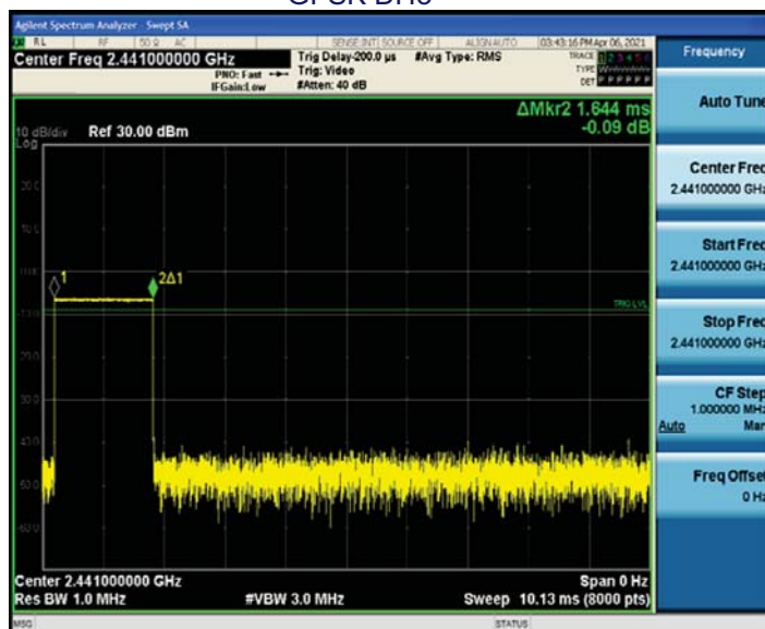
GFSK DH3
