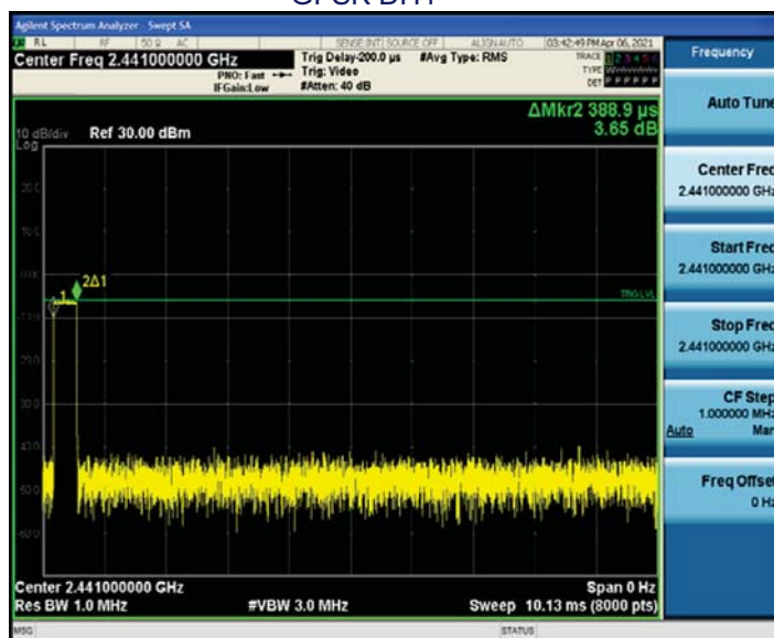
GFSK DH1
