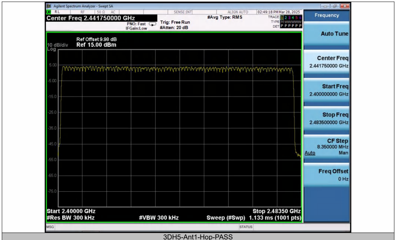
3DH5-Ant1-Hop-PASS
