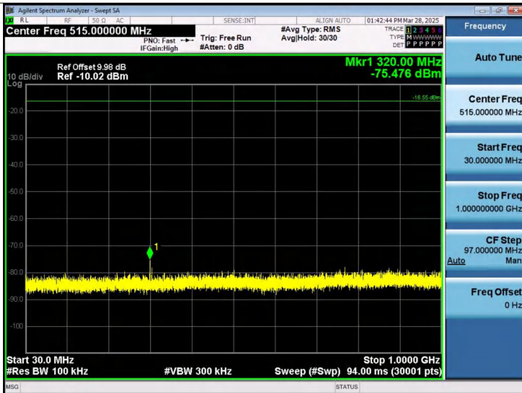
DH5-Ant1-2402-30~1000-PASS
