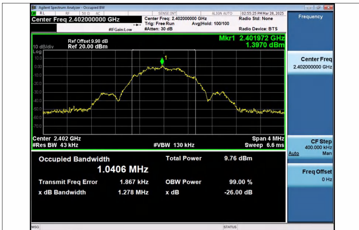
BLE_1M-Ant1-2402
