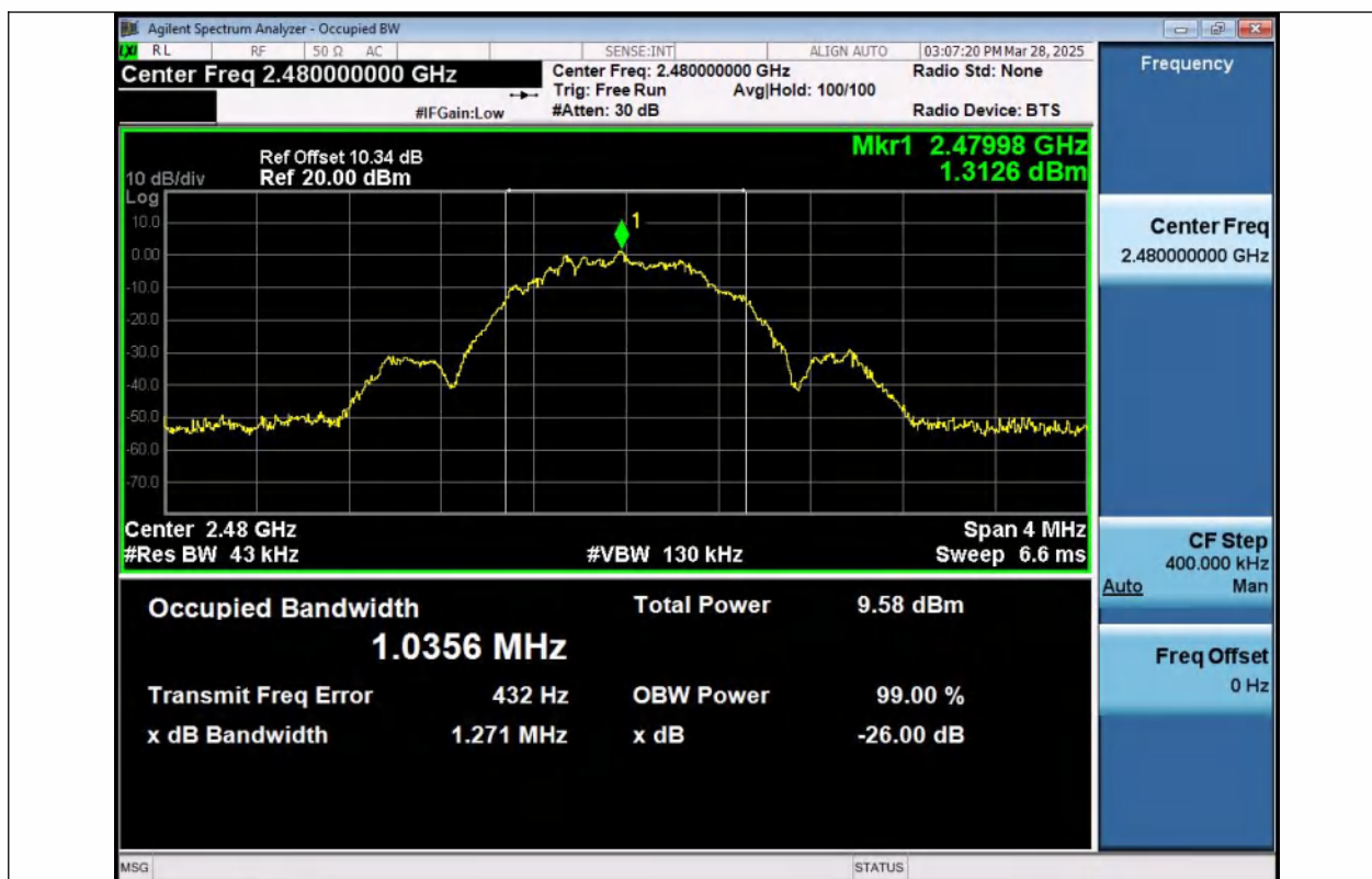
BLE_1M-Ant1-2480
