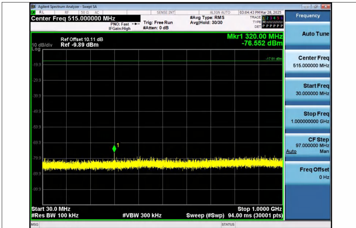
BLE_1M-Ant1-2440-30~1000-PASS
