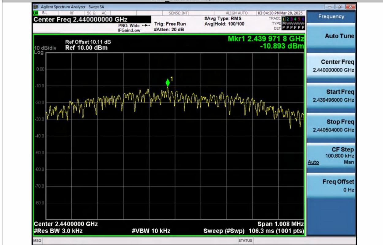
BLE_1M-Ant1-2440-PASS
