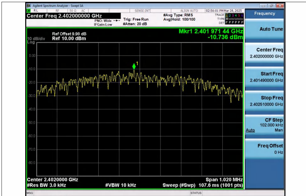
BLE_1M-Ant1-2402-PASS
