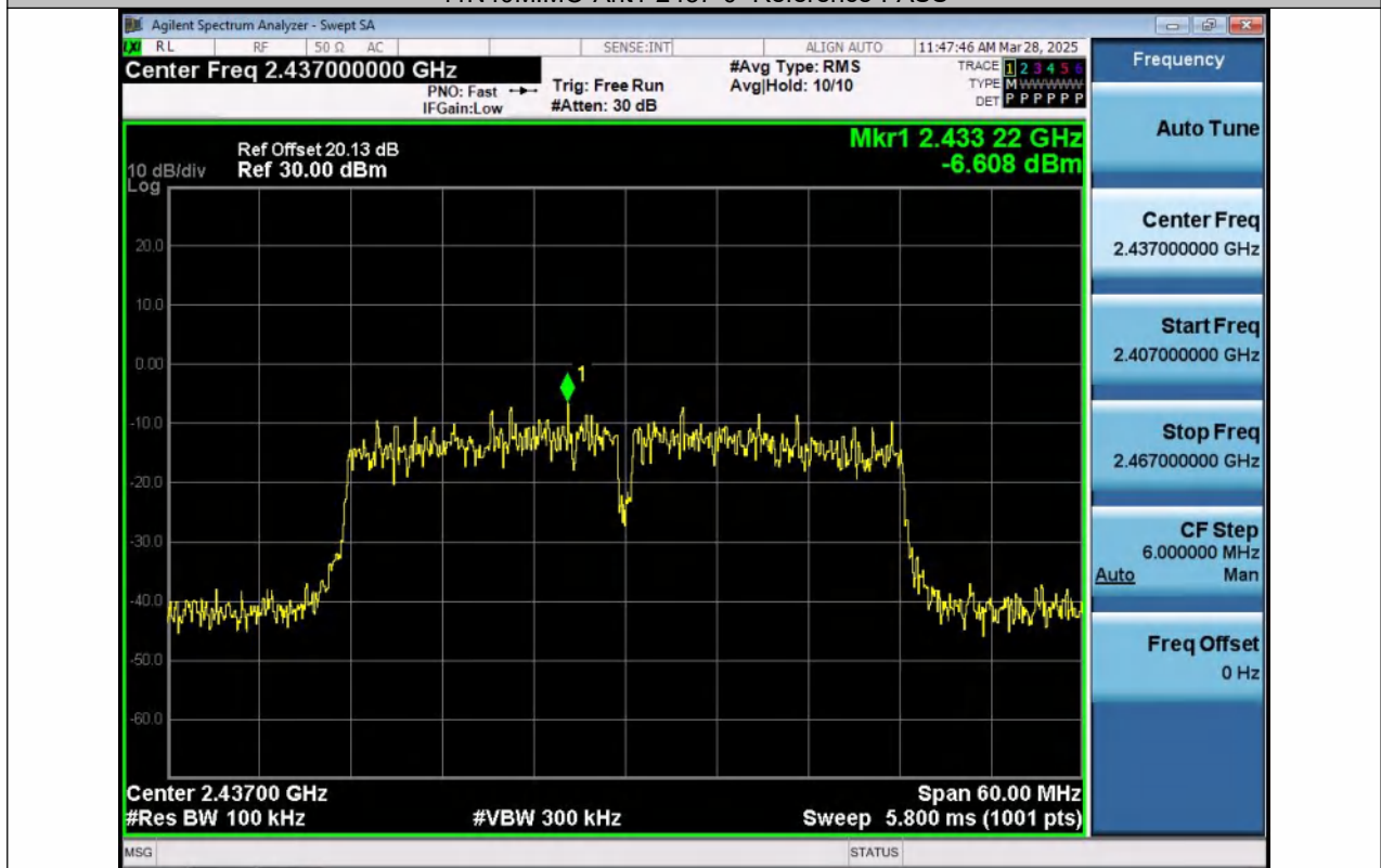
11N40MIMO-Ant2-2437-0~Reference-PASS
