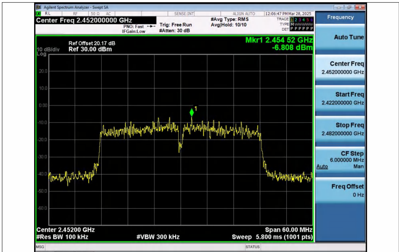
11N40MIMO-Ant1-2452-0~Reference-PASS
