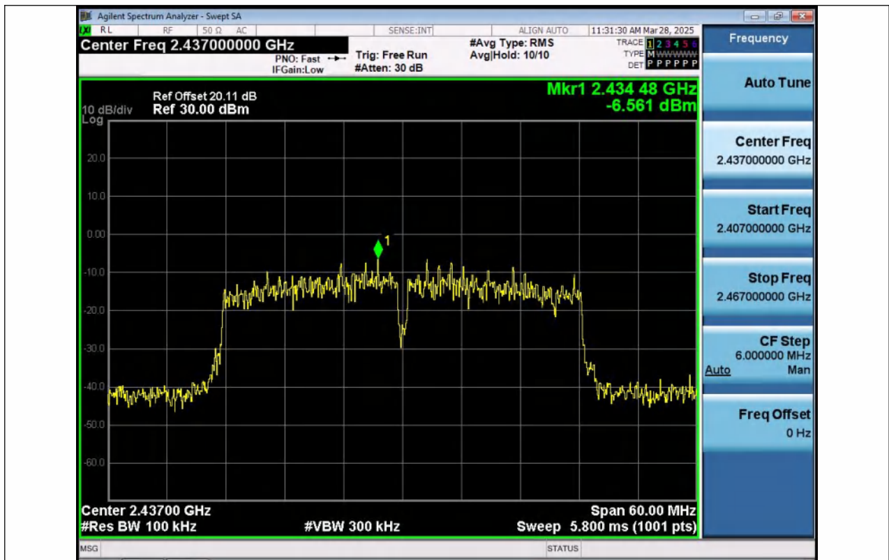
11N40MIMO-Ant1-2437-0~Reference-PASS
