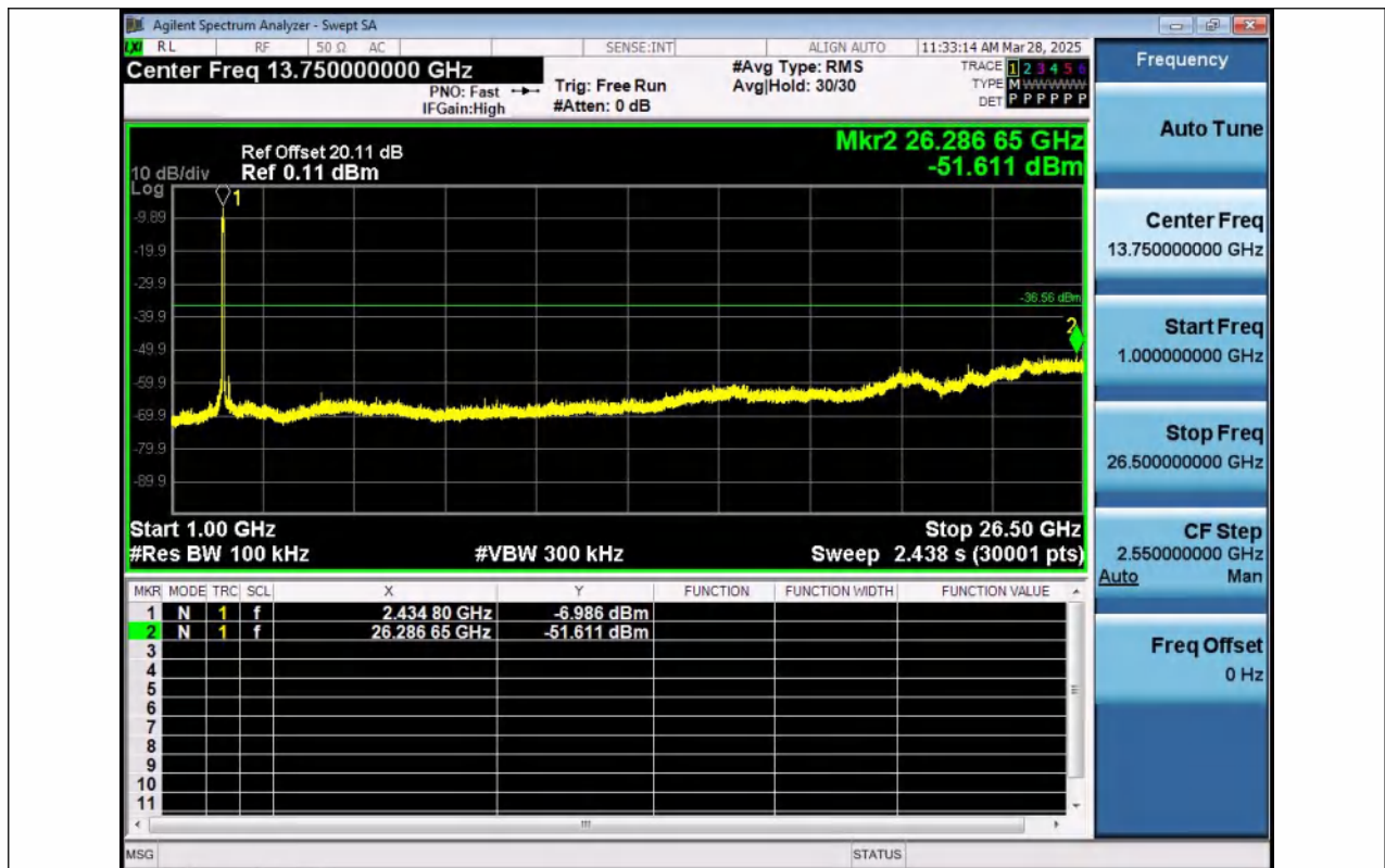
11N40MIMO-Ant1-2437-1000~26500-PASS
