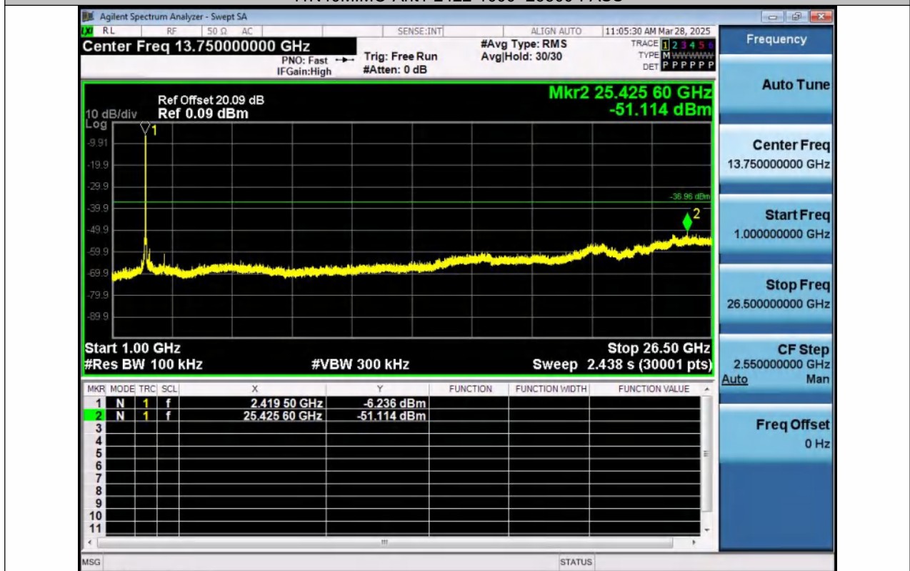
11N40MIMO-Ant2-2422-1000~26500-PASS
