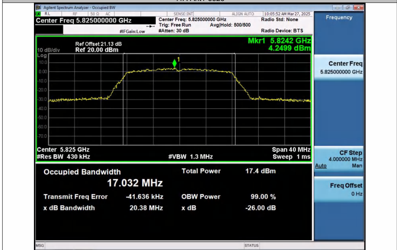
11A-Ant2-5825
