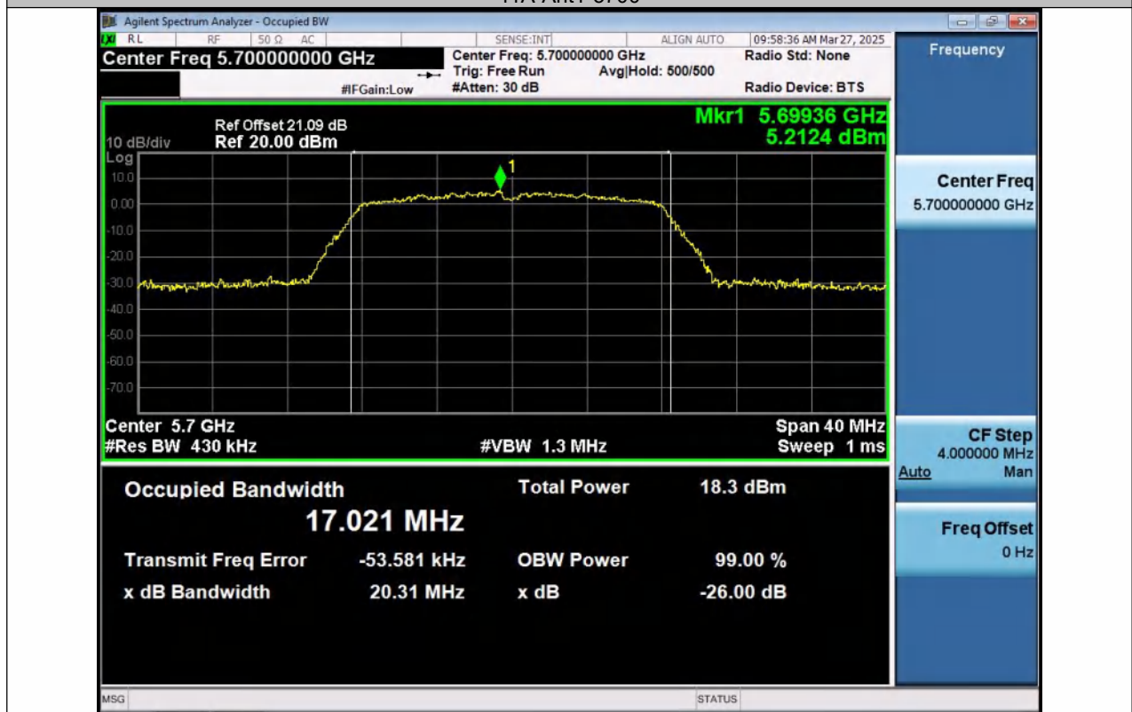
11A-Ant2-5700
