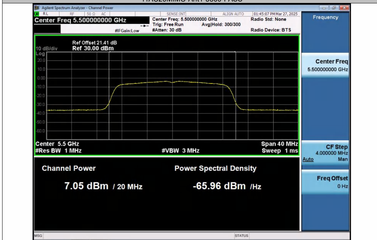
11AC20MIMO-Ant2-5500-PASS
