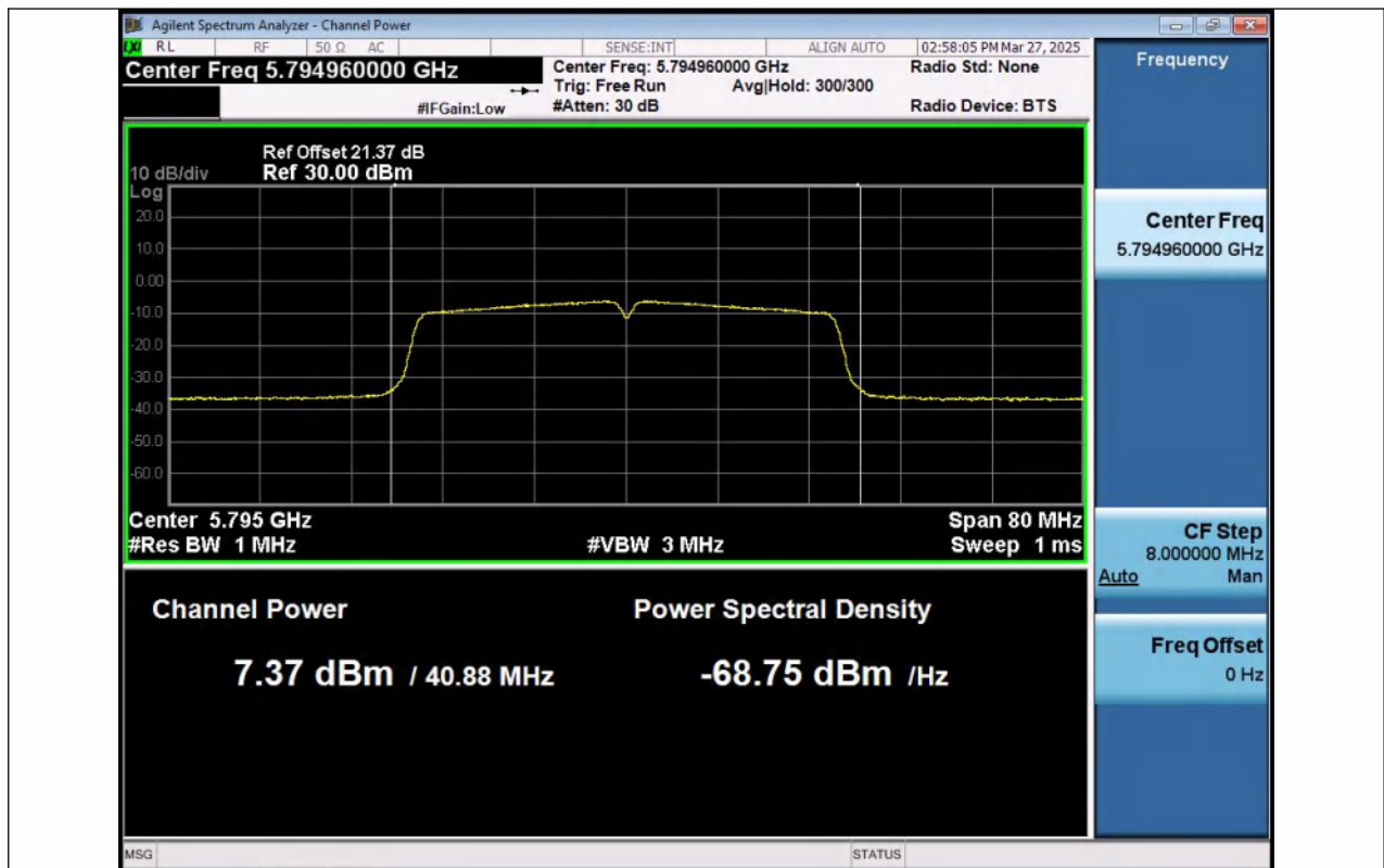
11AC40MIMO-Ant1-5795-PASS
