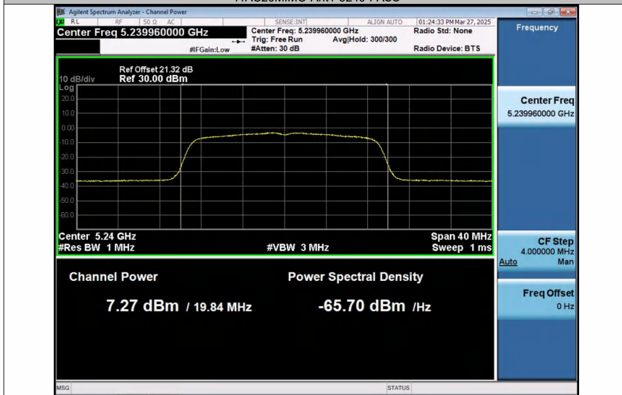
11AC20MIMO-Ant2-5240-PASS
