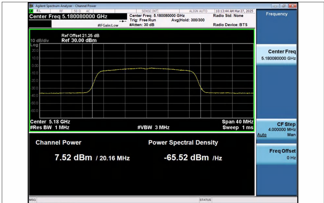
11N20MIMO-Ant1-5180-PASS
