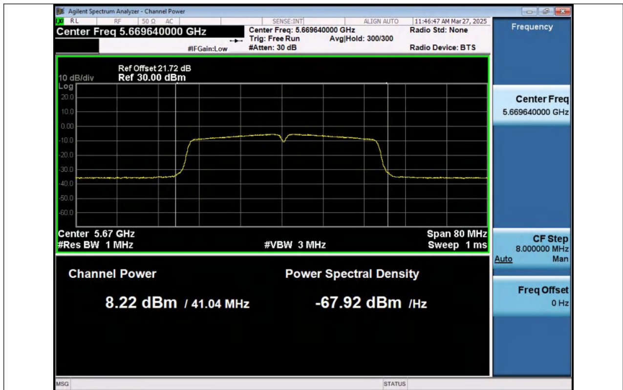
11N40MIMO-Ant1-5670-PASS
