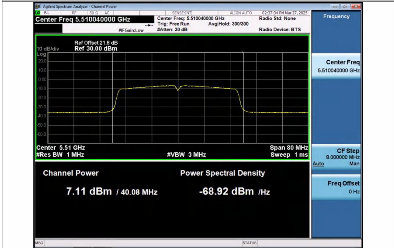
11AC40MIMO-Ant2-5510-PASS
