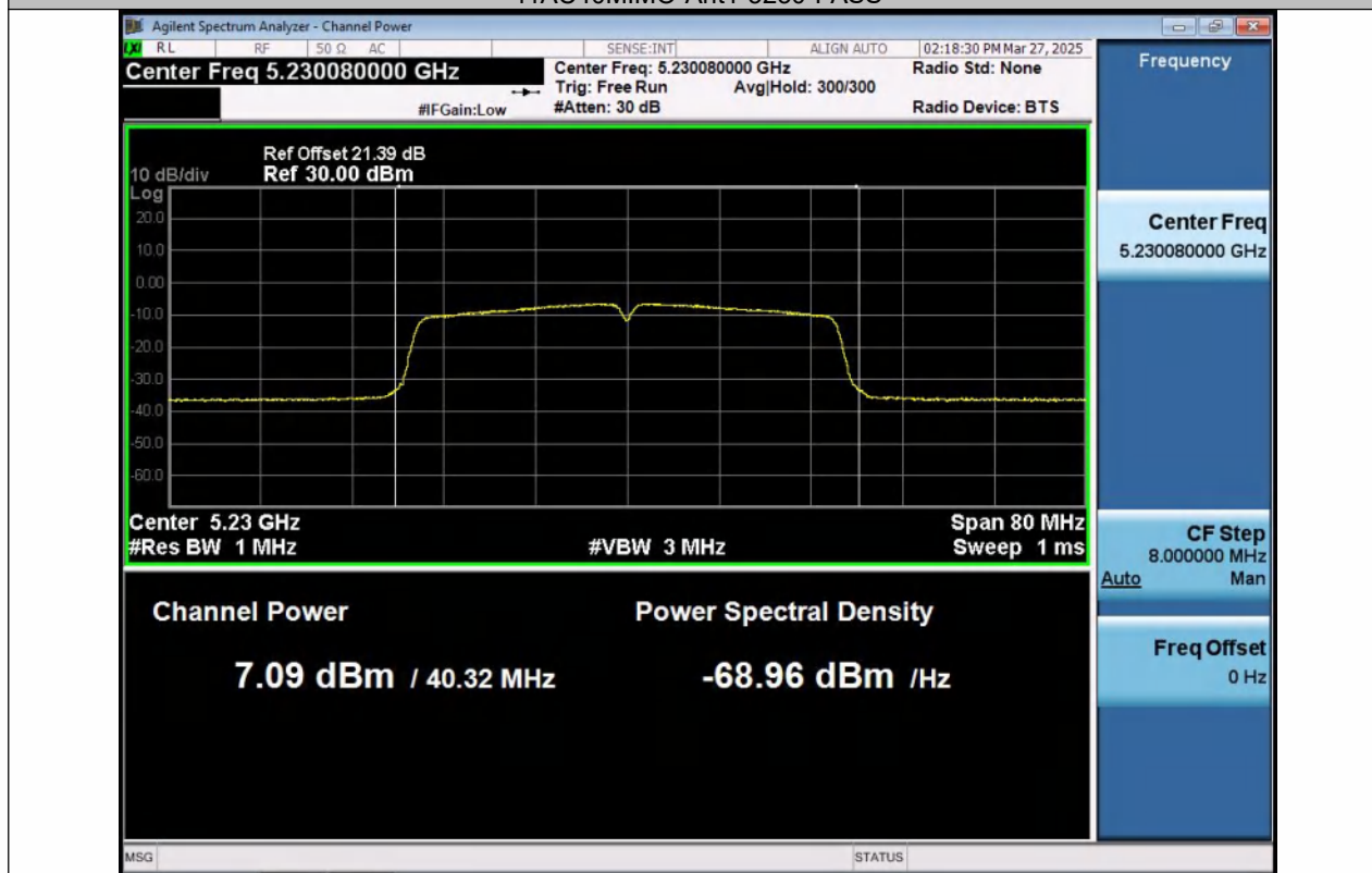
11AC40MIMO-Ant2-5230-PASS
