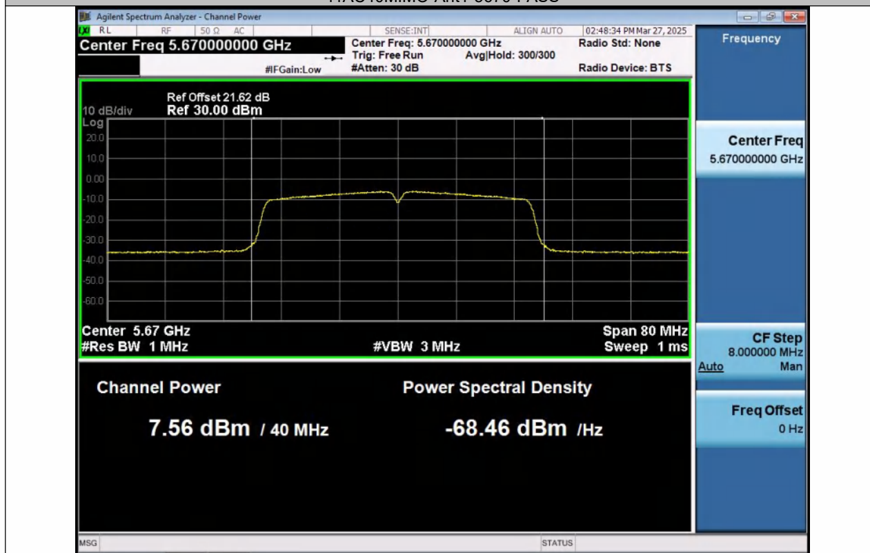
11AC40MIMO-Ant2-5670-PASS
