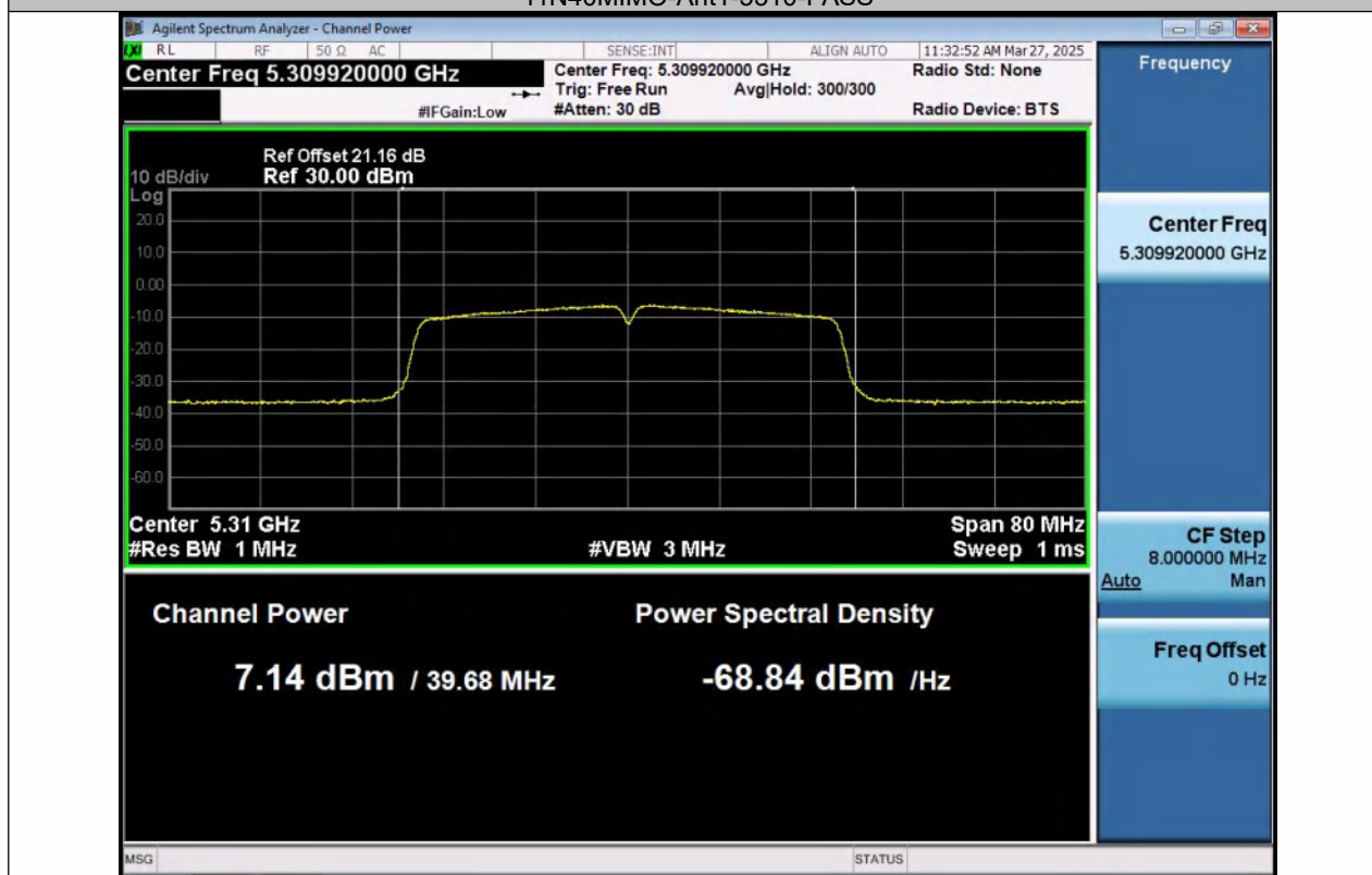
11N40MIMO-Ant2-5310-PASS
