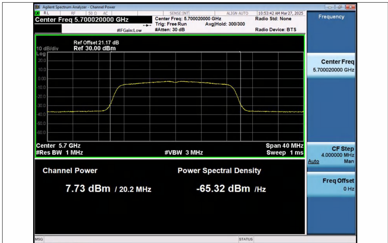
11N20MIMO-Ant1-5700-PASS
