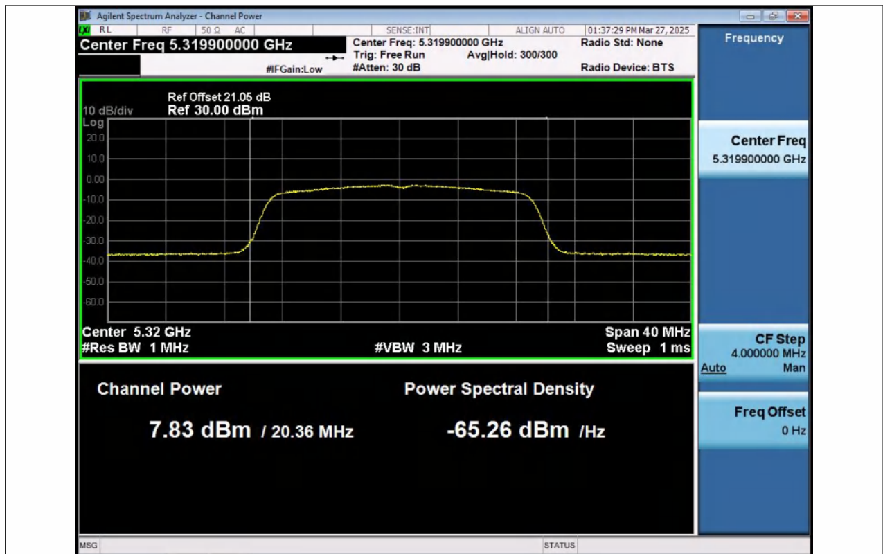
11AC20MIMO-Ant1-5320-PASS
