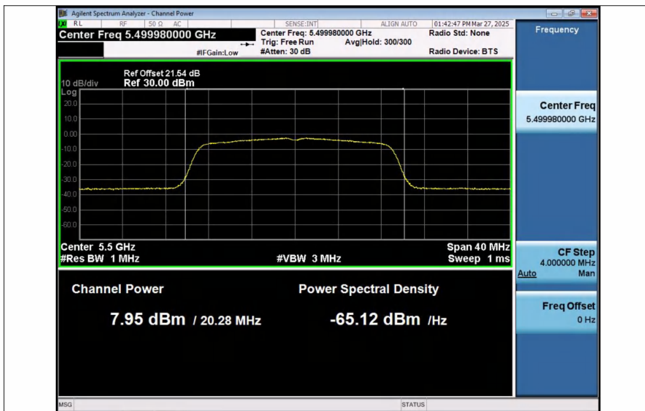
11AC20MIMO-Ant1-5500-PASS
