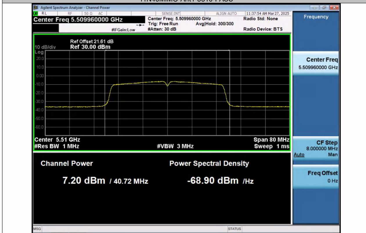
11N40MIMO-Ant2-5510-PASS
