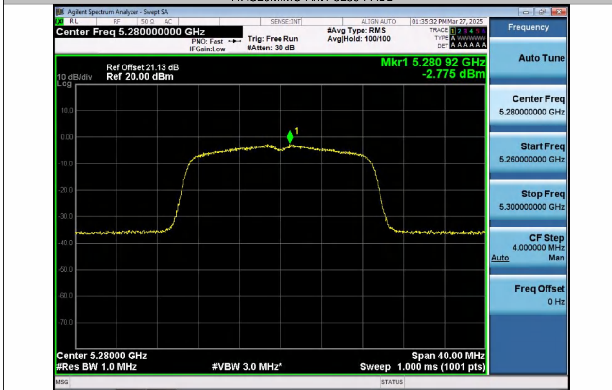
11AC20MIMO-Ant2-5280-PASS
