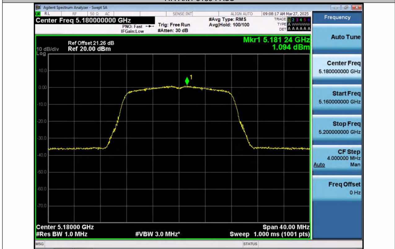
11A-Ant2-5180-PASS
