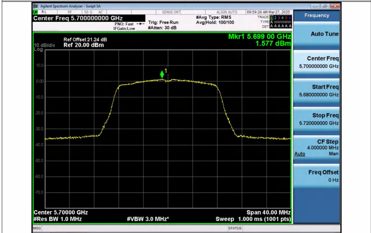
11A-Ant2-5700-PASS
