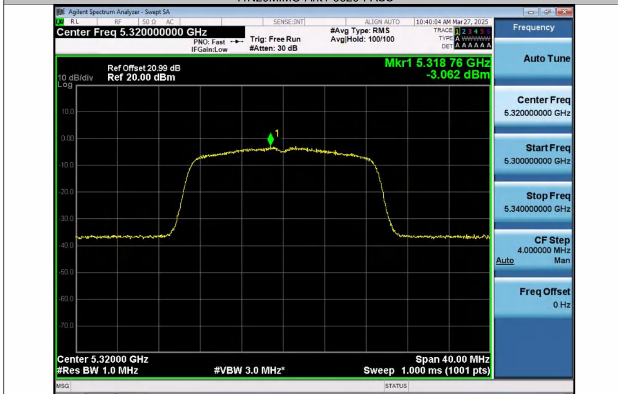
11N20MIMO-Ant2-5320-PASS
