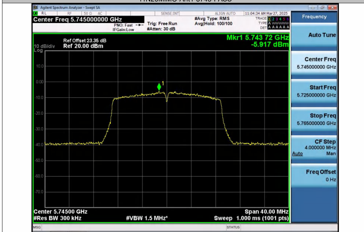
11N20MIMO-Ant2-5745-PASS
