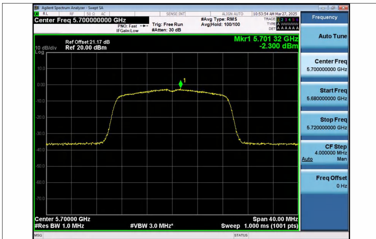
11N20MIMO-Ant1-5700-PASS
