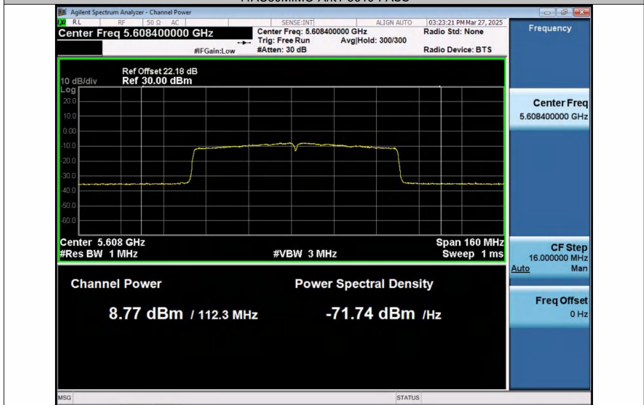
11AC80MIMO-Ant2-5610-PASS
