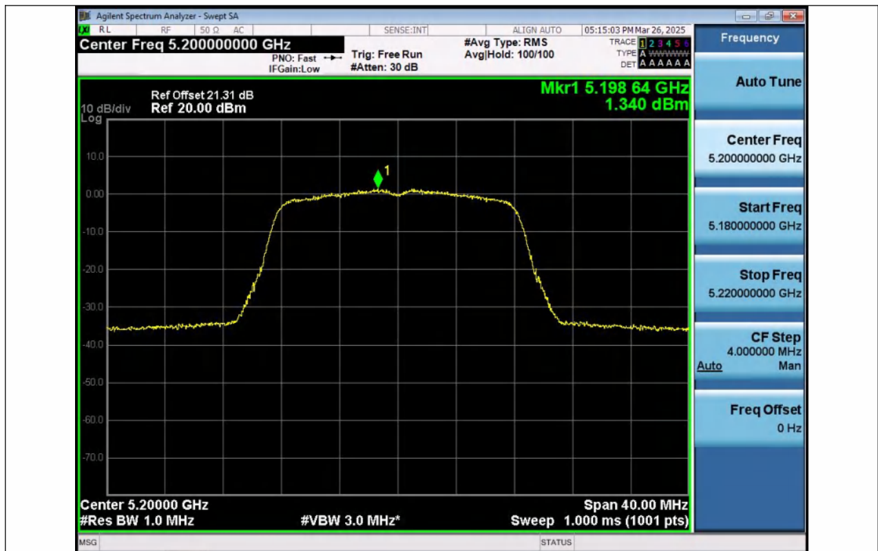
11A-Ant1-5200-PASS
