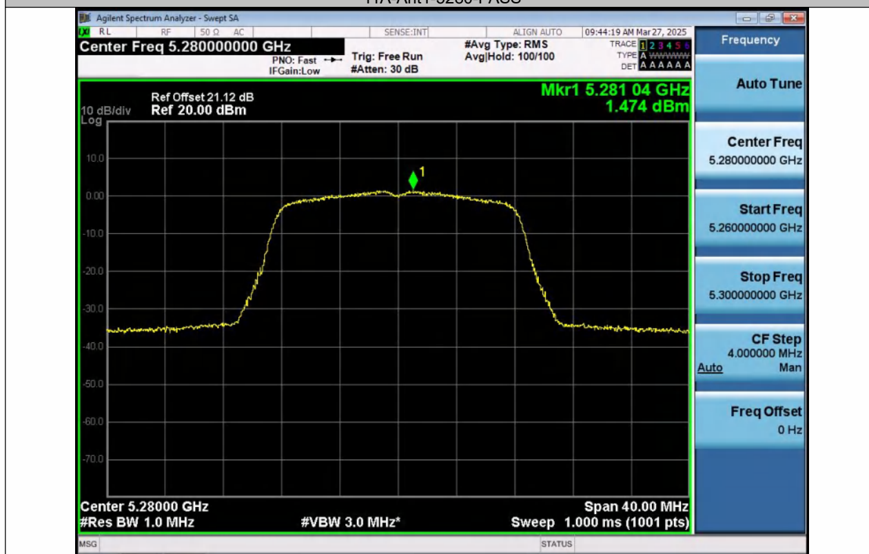
11A-Ant2-5280-PASS
