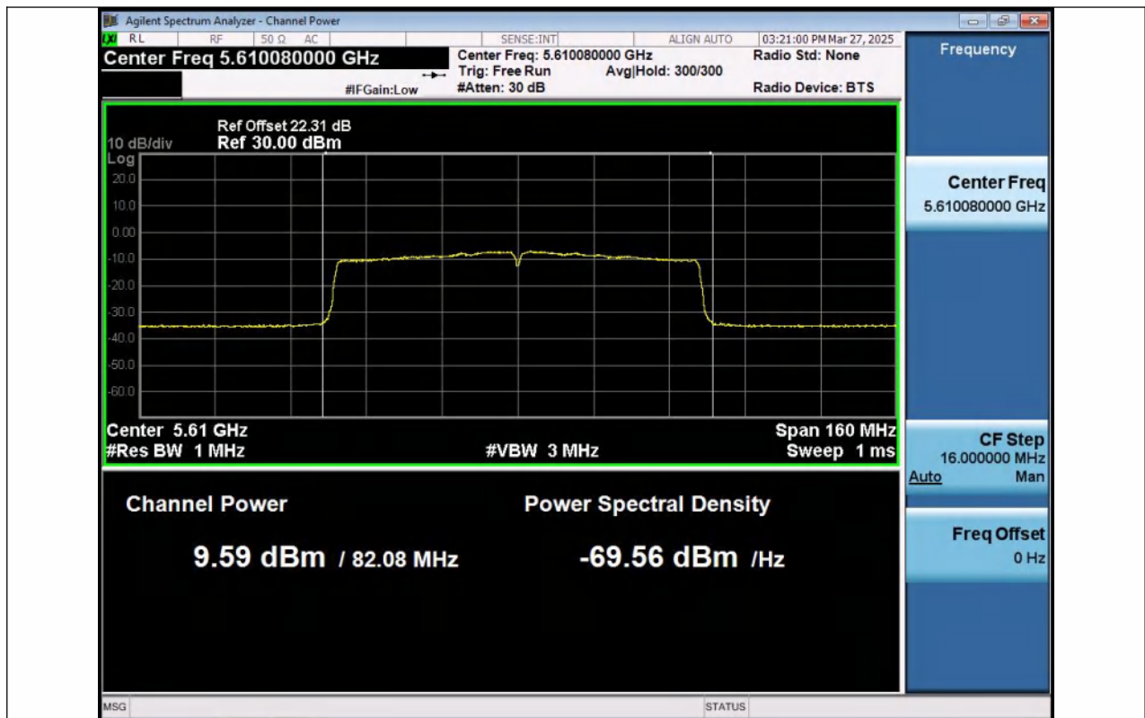
11AC80MIMO-Ant1-5610-PASS
