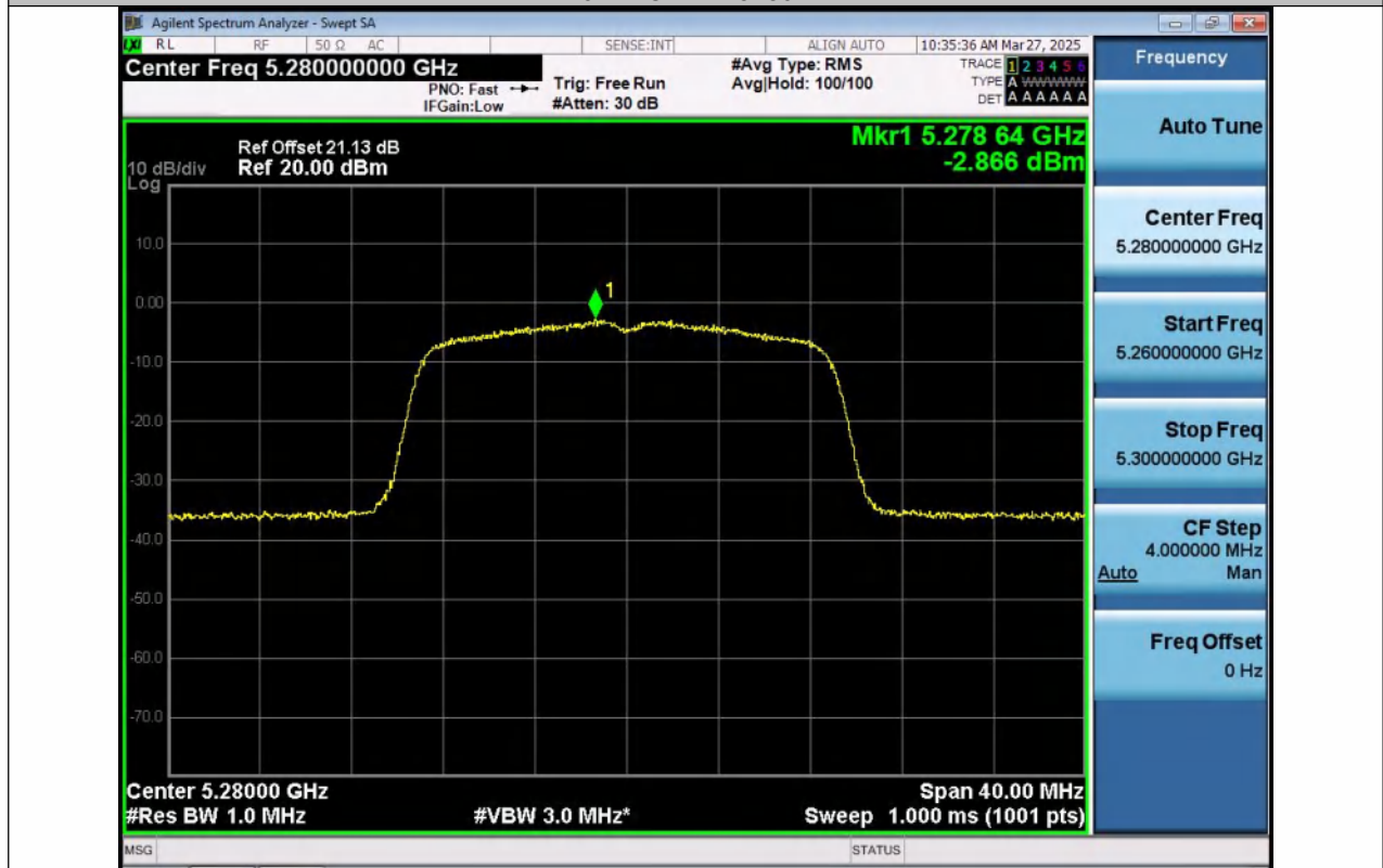
11N20MIMO-Ant2-5280-PASS
