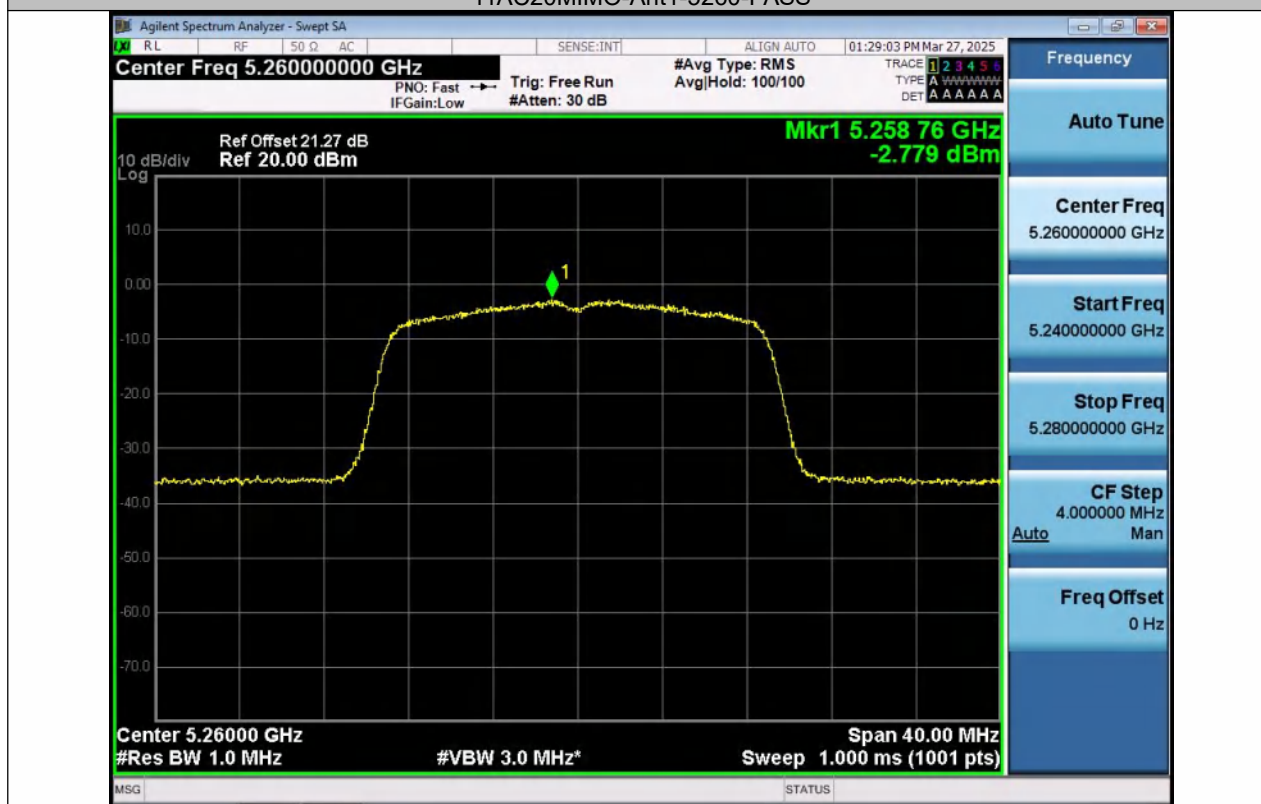
11AC20MIMO-Ant2-5260-PASS
