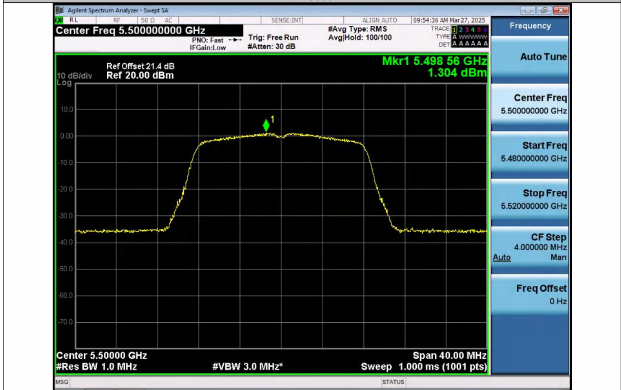
11A-Ant2-5500-PASS
