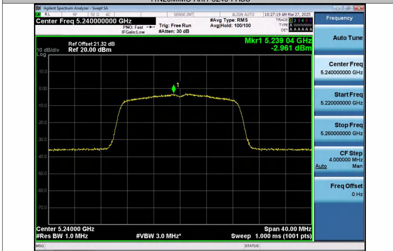
11N20MIMO-Ant2-5240-PASS
