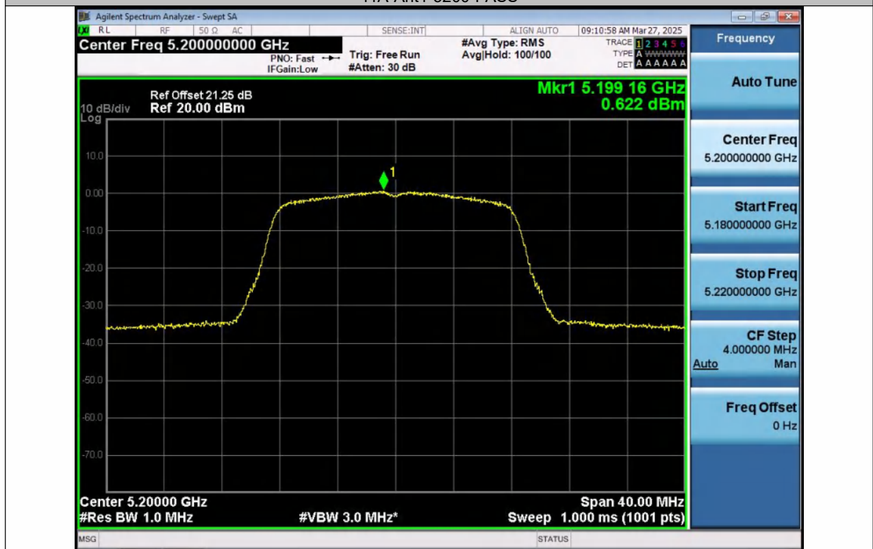
11A-Ant2-5200-PASS
