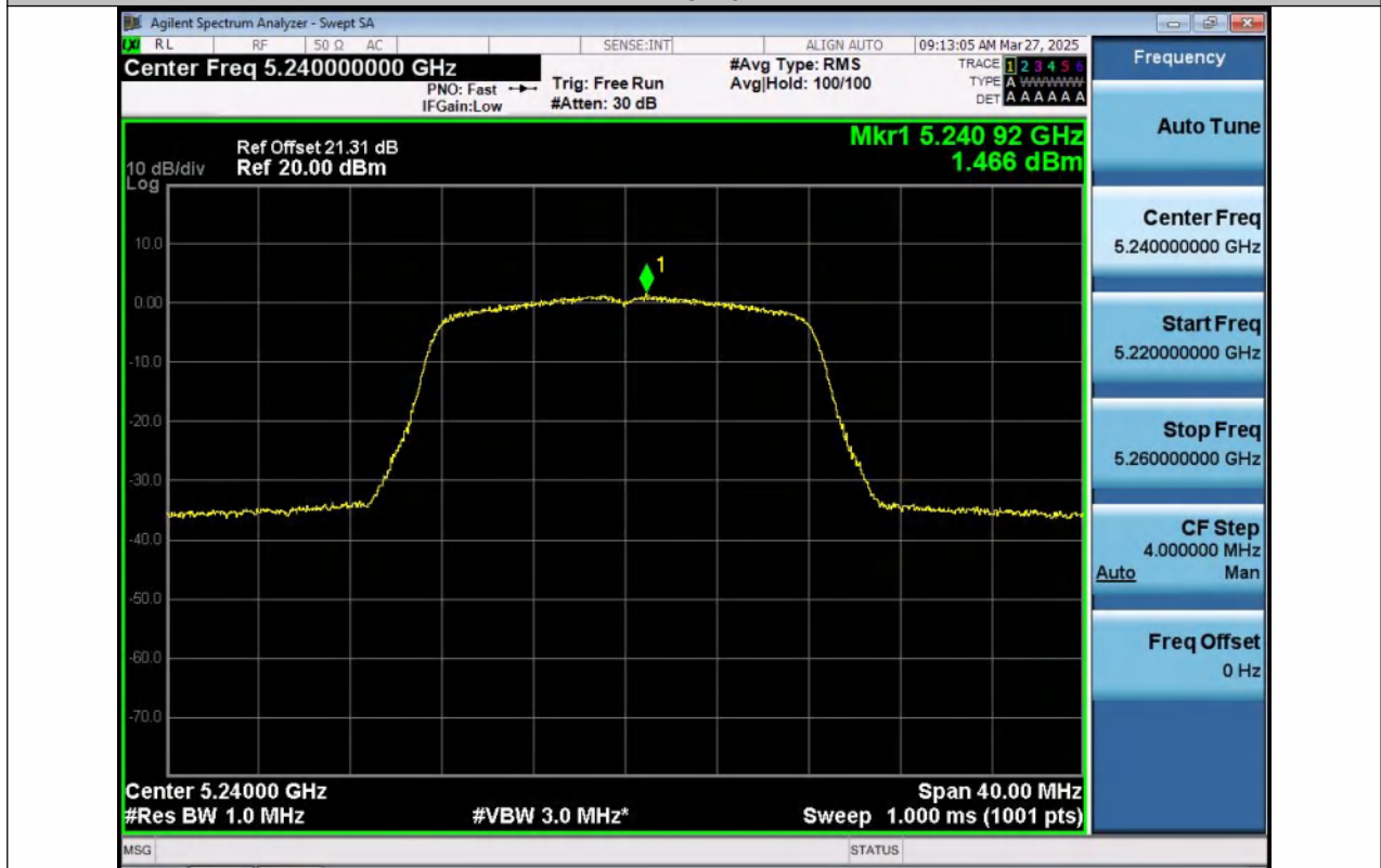
11A-Ant2-5240-PASS
