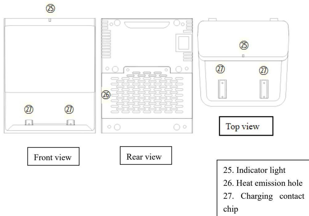
Fig. 2 Structure drawing of the charging pile
