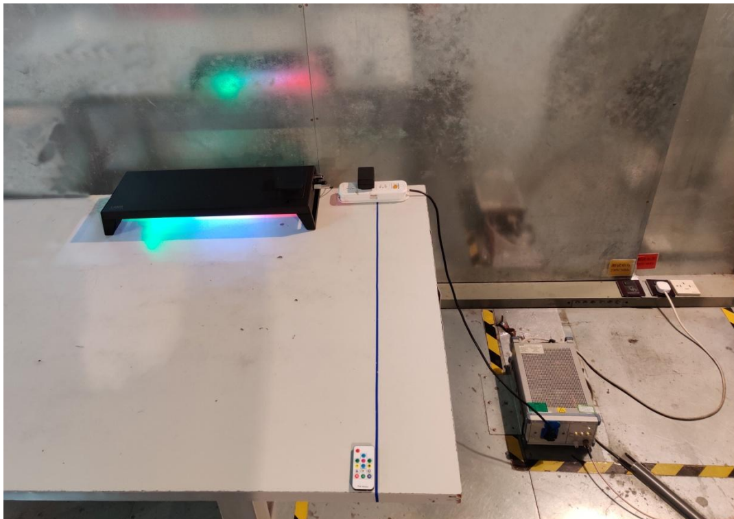
AC Conducted Measurement Photos
