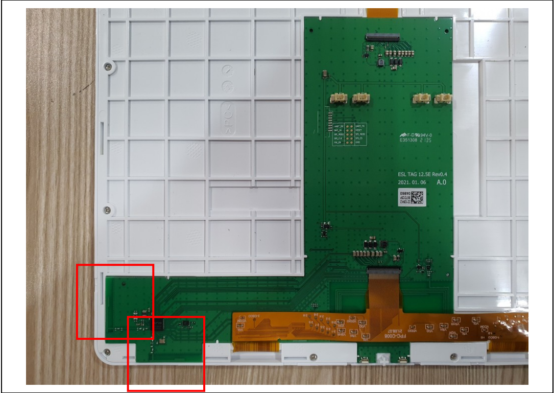
Antenna(2.4GHz ANT)
