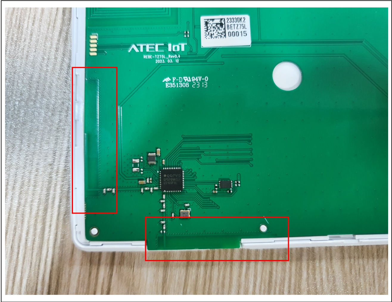
Antenna(2.4GHz ANT)
