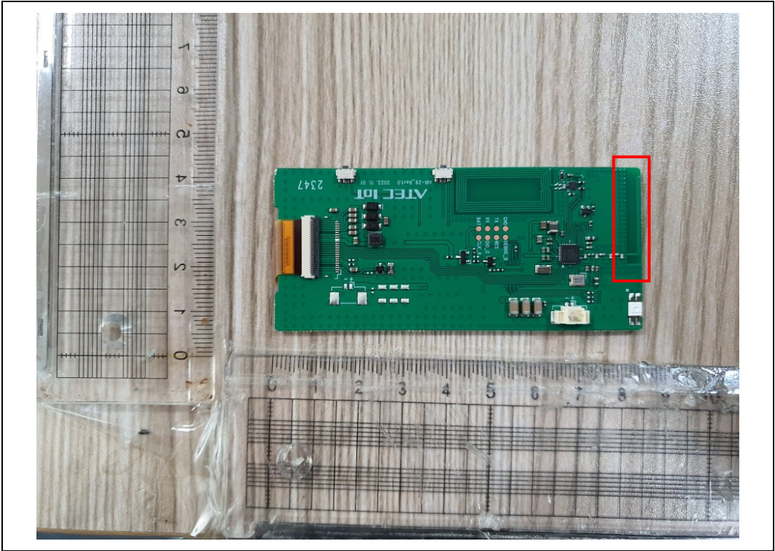
Antenna(2.4GHz ANT)
