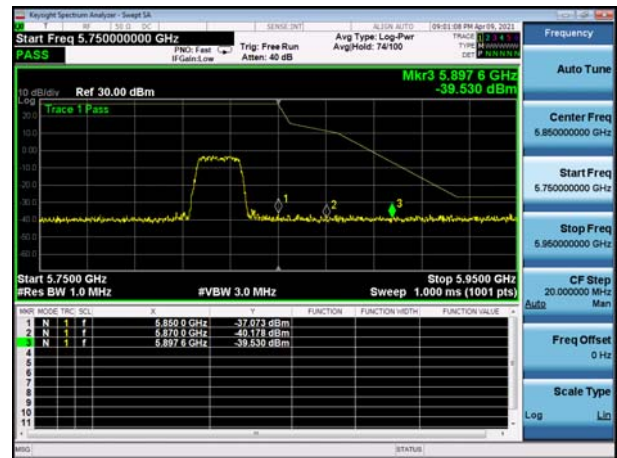
U-NII-3 ,Plot 1,Band Edge-802.11ac(80 MHz),5775MHz,Ant1 Right edge
