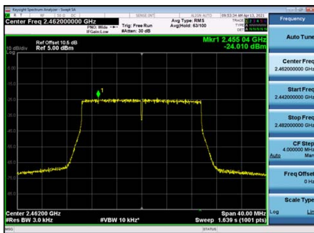
Power spectral density-802.11ax(HE20) ,2462MHz,Ant0
