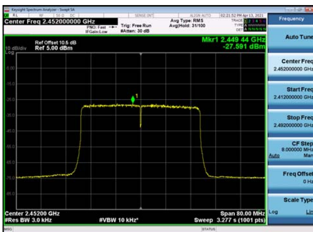
Power spectral density-802.11ax(HE40) ,2452MHz,Ant0
