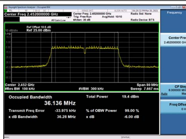
6dB Bandwidth-802.11n(HT40),2452MHz
