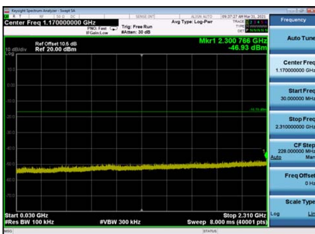
,Plot 3,30MHz~2310MHz-802.11g,2437MHz ,Ant1
