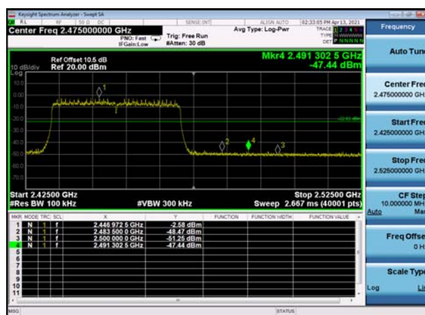
,Plot 2,Band Edge-802.11ax(HE40) ,2452MHz,Ant1
