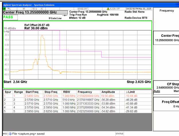
7C / 15+10MHz / High CH / QPSK / 1#74-1#0
