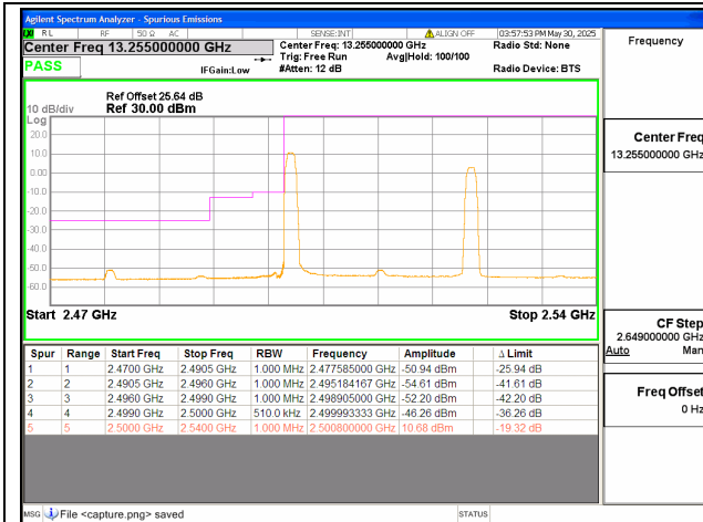
7C / 15+10MHz / Low CH / QPSK / 1#0-1#49
