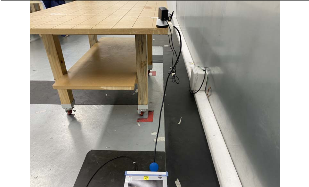
Conducted Emission_REAR
