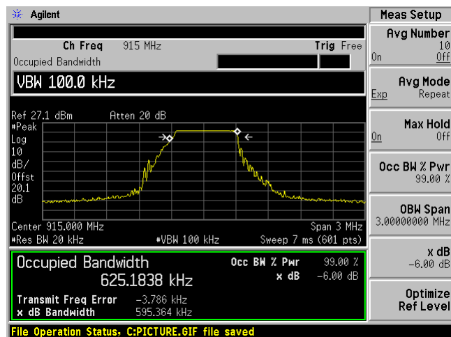
99% OBW
