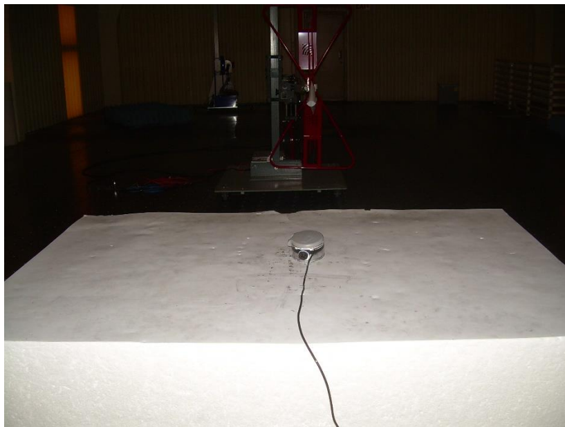
Photograph 2: Back View Radiated Emissions Configuration
