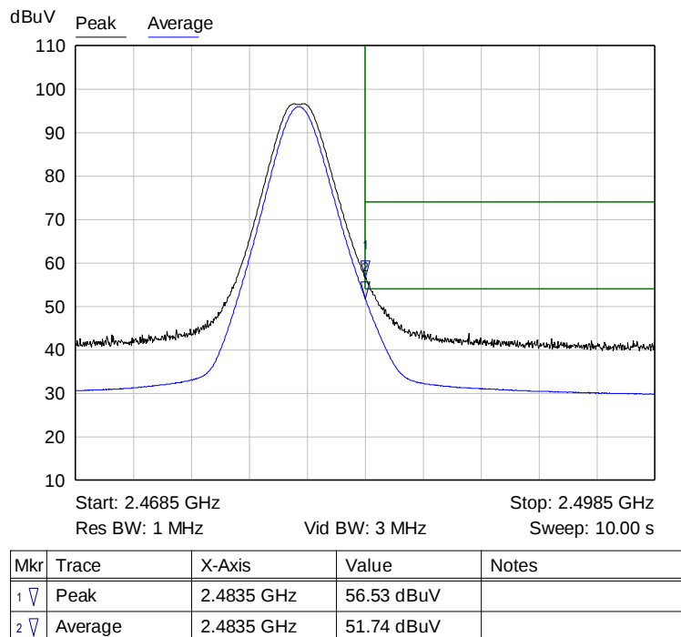
Graph 8: Radiated Upper Band Edge Plot
