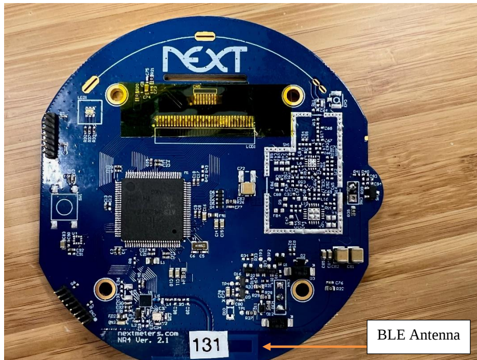
Photograph 13: Top View of the PCB
