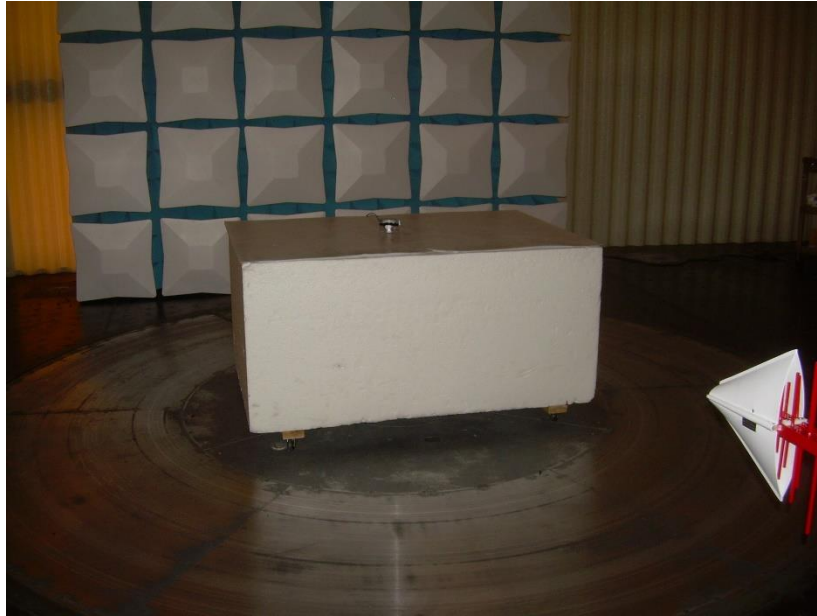
Photograph 1: Front View Radiated Emissions Configuration
