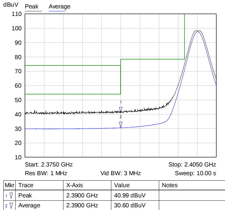
Graph 7: Radiated Lower Band Edge Plot
