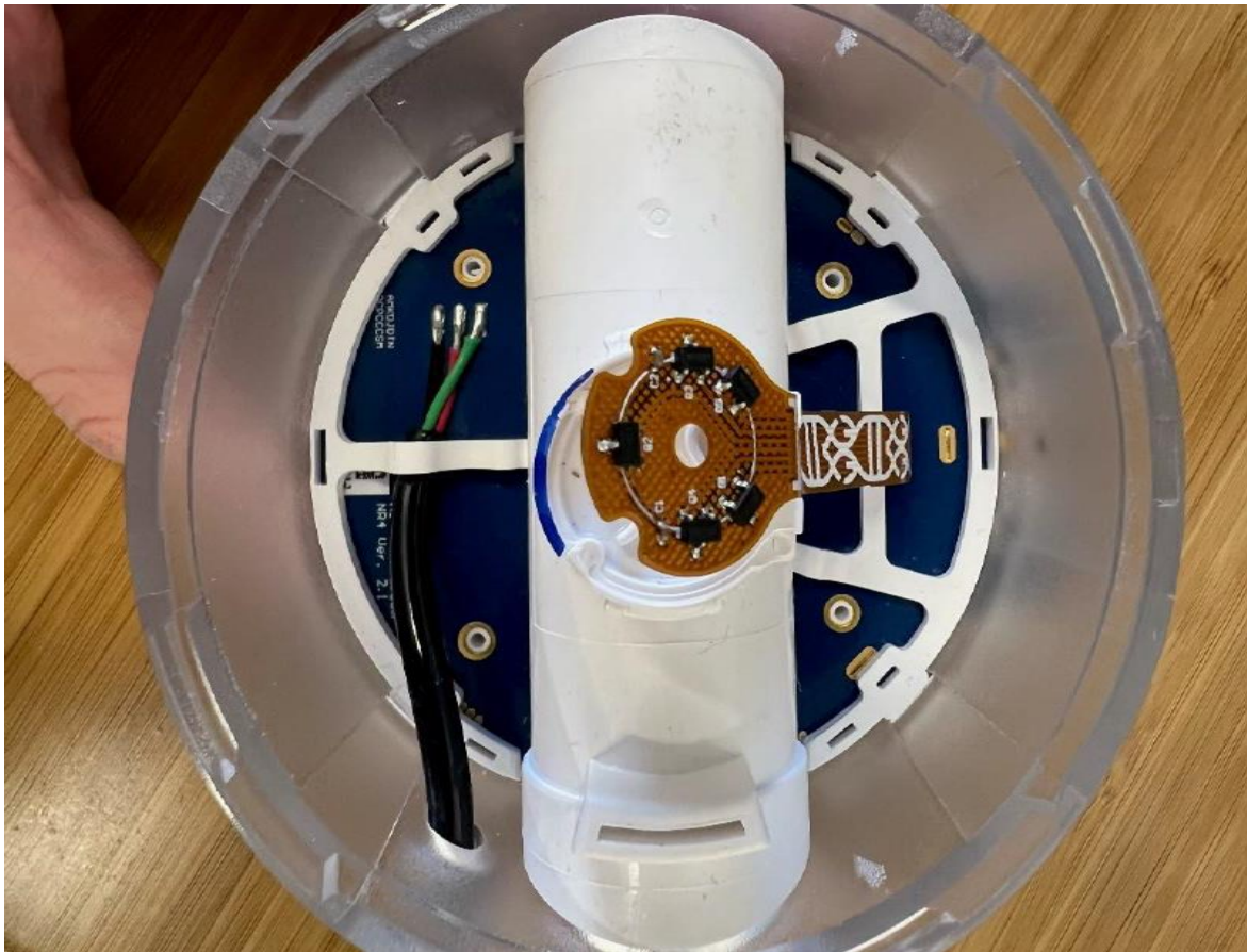
Photograph 3 – View of PCB in Housing
