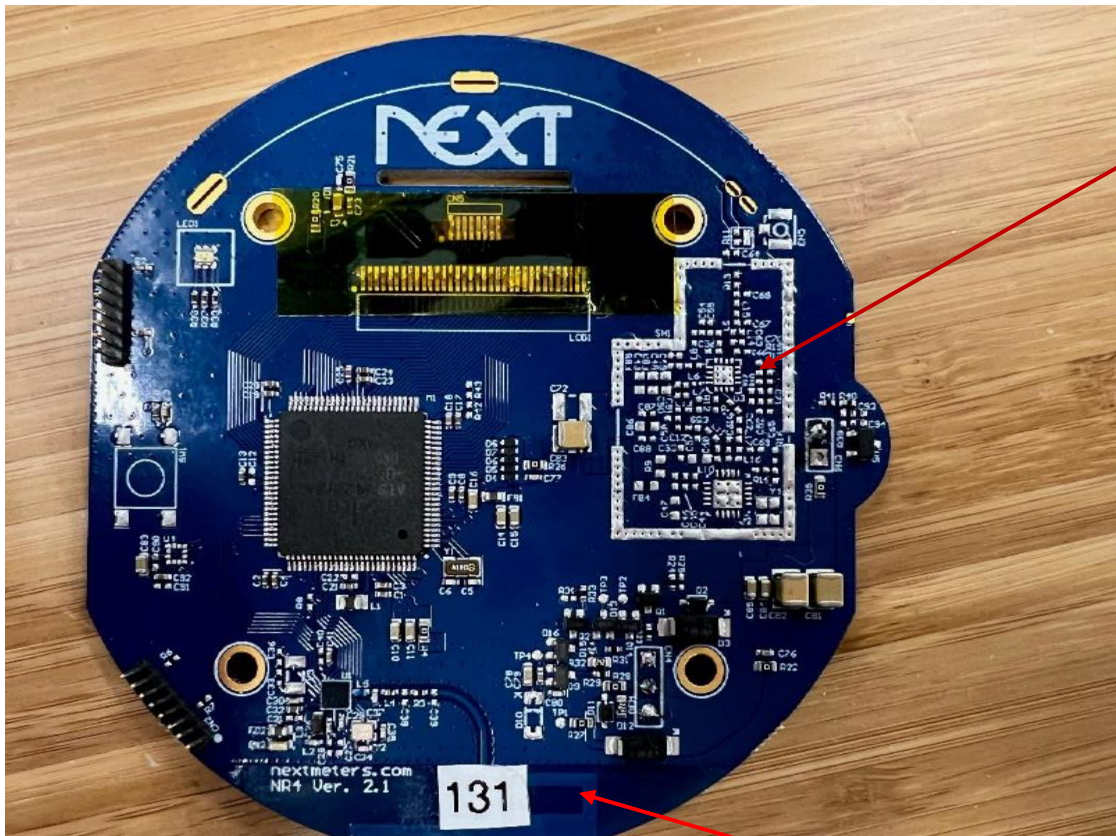
Photograph 1 – Front View of the Device
