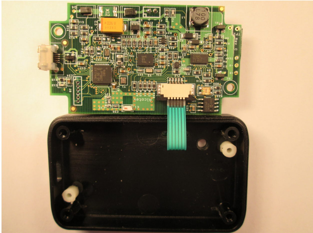
Inside – Top of Assembly
