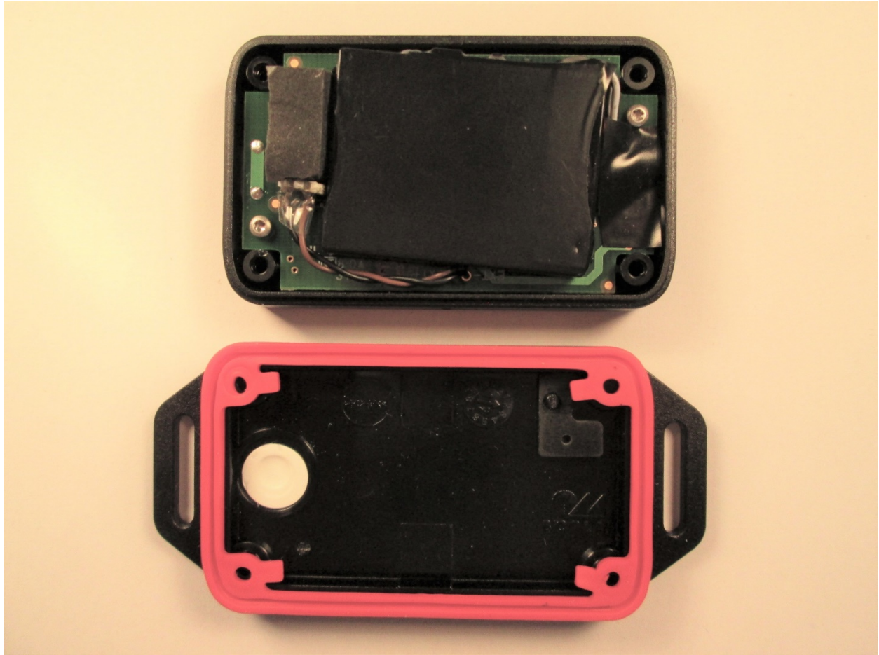
Inside – Bottom of Assembly
