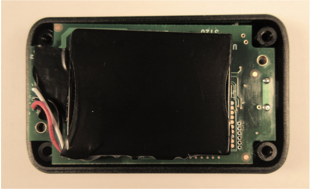
Bottom of PCB with battery
