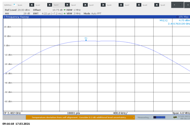
Figure 8.6-1: Output power on low channel
