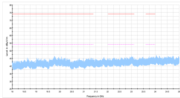
NEX-432270 Radiated Emissions 18 - 25 GHz BLE mid channel Preview Result 1-PK+ FCC 15.209 and RSS-Gen Restricted bands peak limits FCC 15.209 and RSS-Gen Restricted bands average limits
