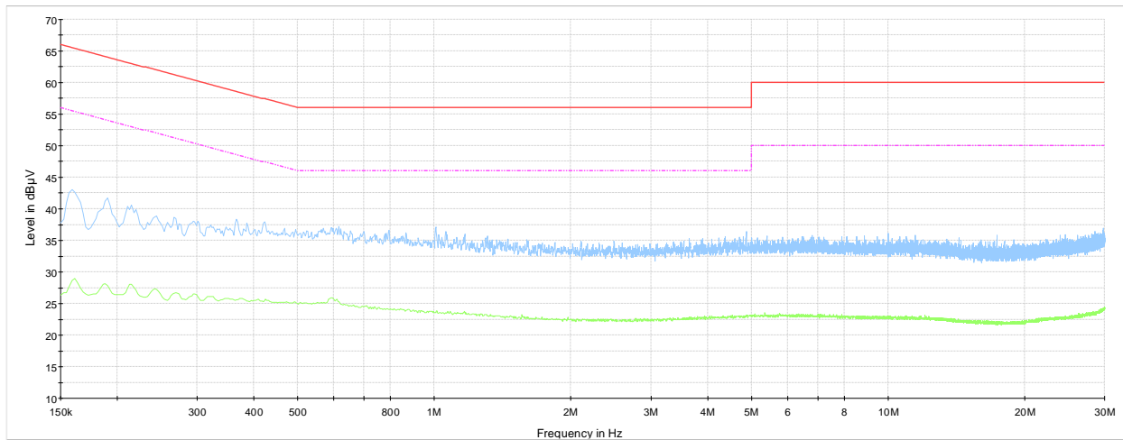
Plot 8.4-3: Conducted emissions on phase line – mid channel
