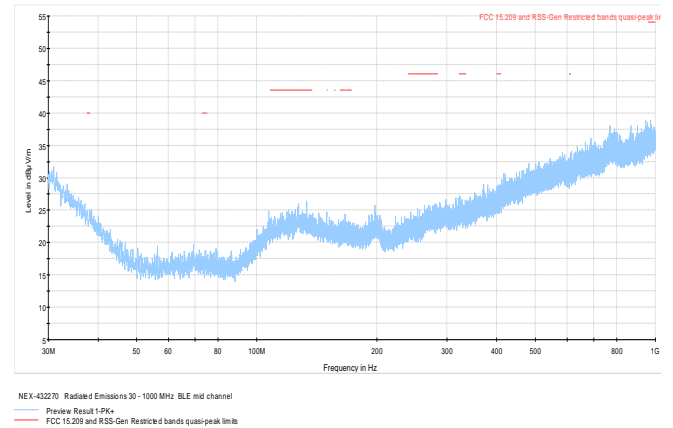
Figure 8.7-11: Radiated spurious emissions below 1 GHz on mid channel
