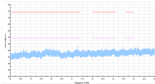
NEX-432270 Radiated Emissions 18 - 25 GHz BLE high channel Preview Result 1-PK+ FCC 15.209 and RSS-Gen Restricted bands peak limits FCC 15.209 and RSS-Gen Restricted bands average limits
