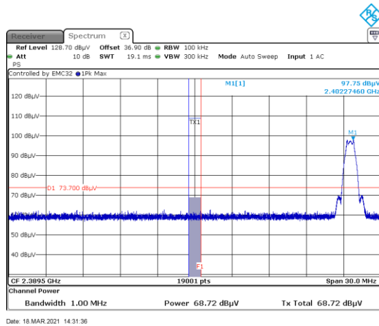
Figure 8.7-3: Radiated Restricted band edge spurious emissions low ch. - Peak
