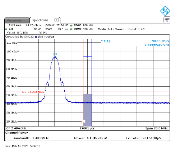
Figure 8.7-6: Radiated Restricted Band edge spurious emissions high channel - average
