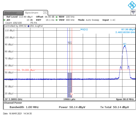
Figure 8.7-4: Radiated Restricted band edge spurious emissions low ch. - Average
