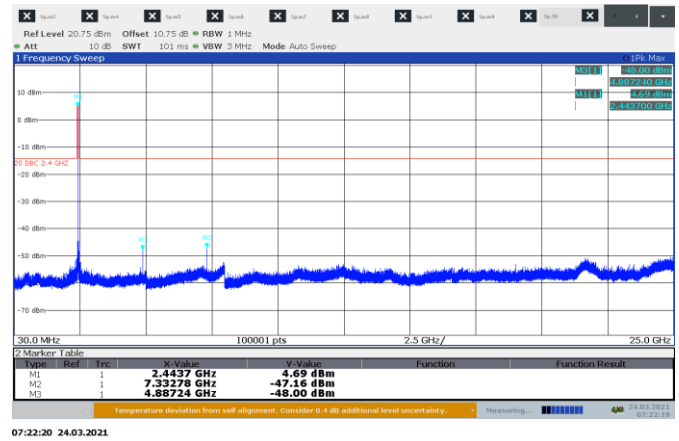
Figure 8.7-8: Conducted spurious emissions on mid channel
