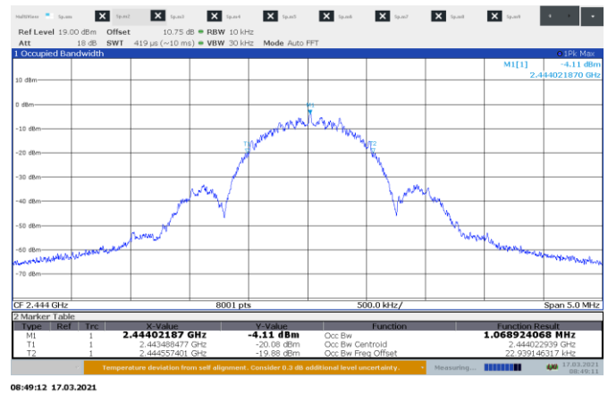
Figure 8.5-5: 99% occupied bandwidth on mid channel
