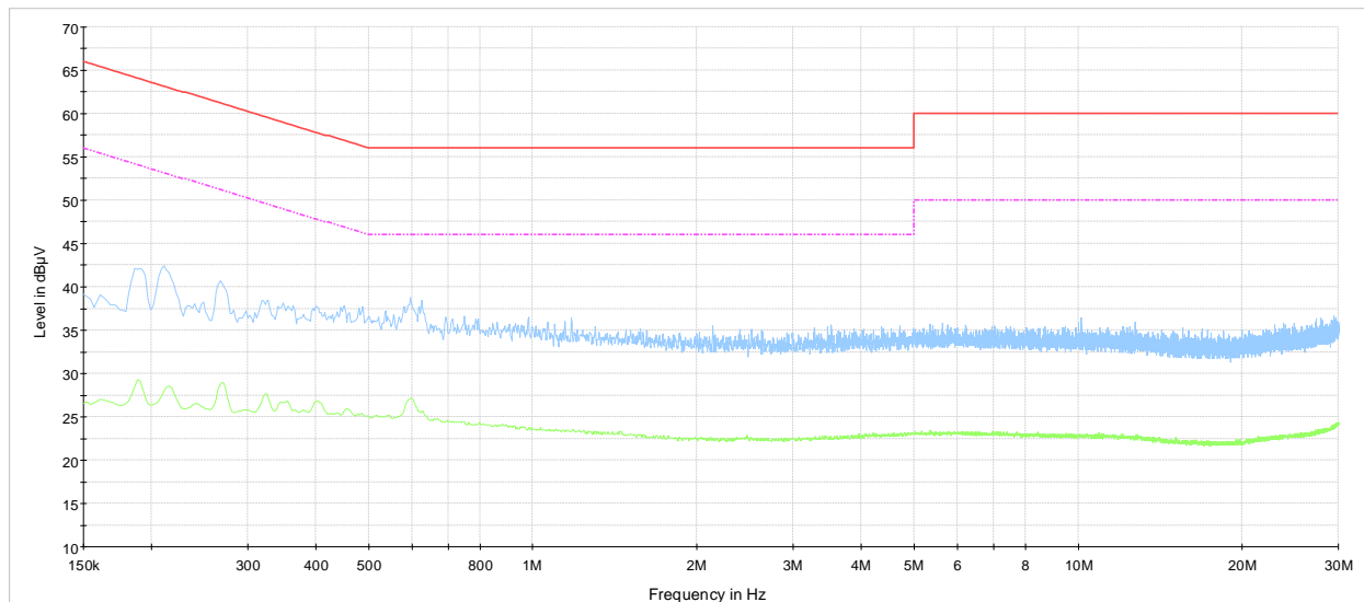
Plot 8.4-1: Conducted emissions on phase line – low channel
