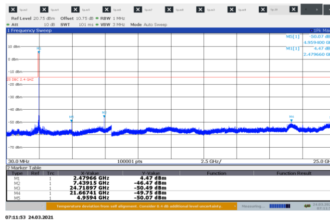
Figure 8.7-9: Conducted spurious emissions on high channel
