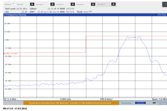
Figure 8.7-1: Conducted Band edge spurious emissions at 2400 MHz
