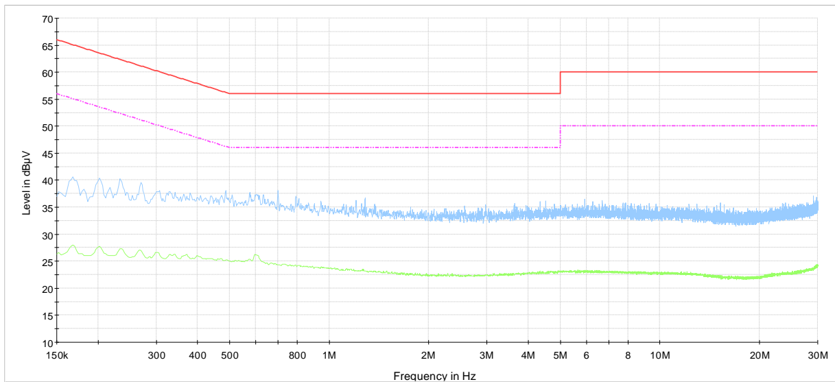
Plot 8.4-5: Conducted emissions on phase line – high channel
