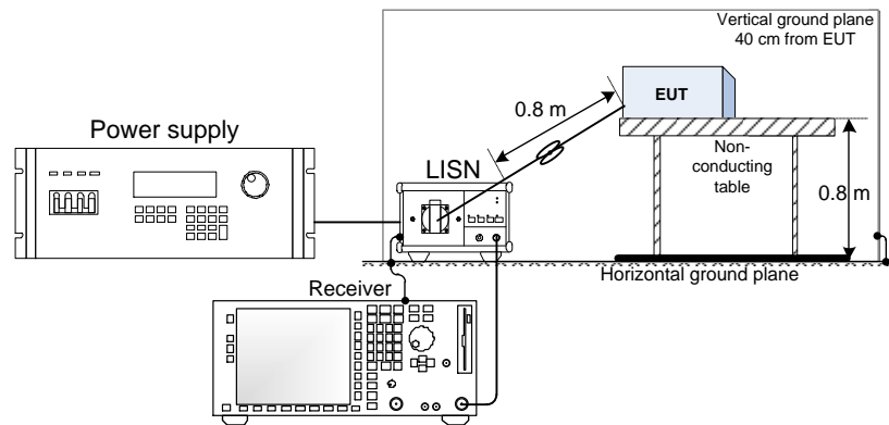
Figure 5.5-4: Conducted emission testing block diagram
