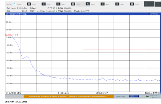
Figure 8.7-2: Conducted Band edge spurious emissions at 2483.5 MHz
