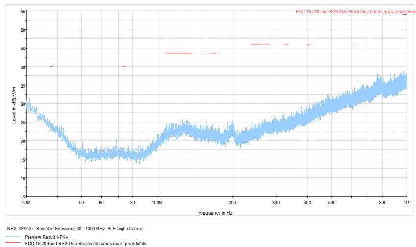
Figure 8.7-12: Radiated spurious emissions below 1 GHz on high channel
