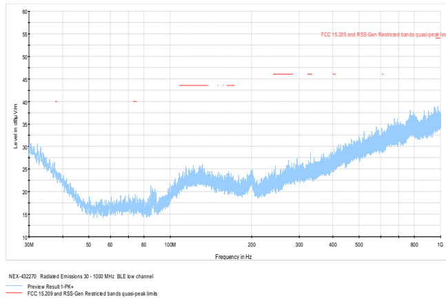
Figure 8.7-10: Radiated spurious emissions below 1 GHz on low channel
