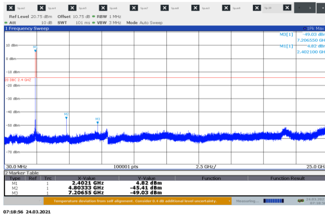
Figure 8.7-7: Conducted spurious emissions on low channel
