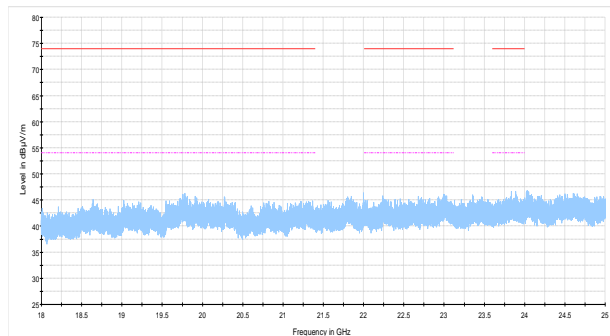
NEX-432270 Radiated Emissions 18 - 25 GHz BLE low channel Preview Result 1-PK+ FCC 15.209 and RSS-Gen Restricted bands peak limits FCC 15.209 and RSS-Gen Restricted bands average limits
