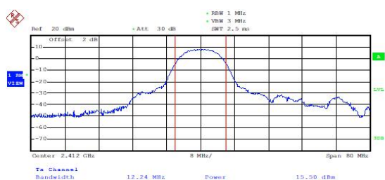
Output Power-Conducted (802.11b, Ch1)
