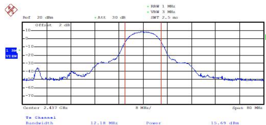
Output Power-Conducted (802.11b, Ch6)
