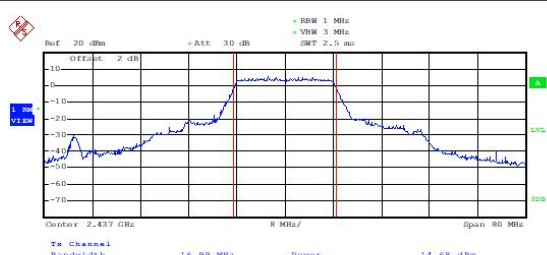
Output Power-Conducted (802.11g, Ch6)
