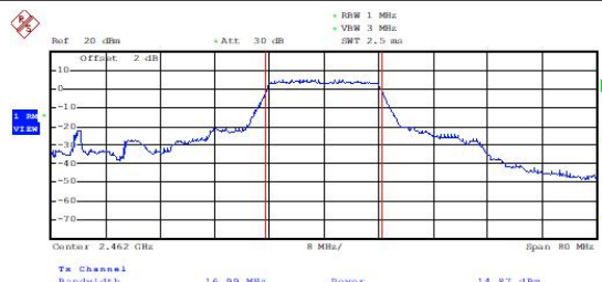
Output Power-Conducted (802.11g, Ch11)
