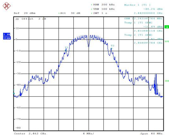
99% Occupied Bandwidth (802.11b, Ch11) 12.244 MHz
