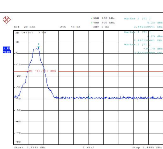
Frequency Band Edge: GFSK, Ch78, Hopping OFF
