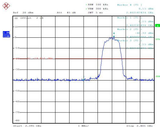
Frequency Band Edge: \pi/4 DQPSK, Ch0, Hopping OFF
