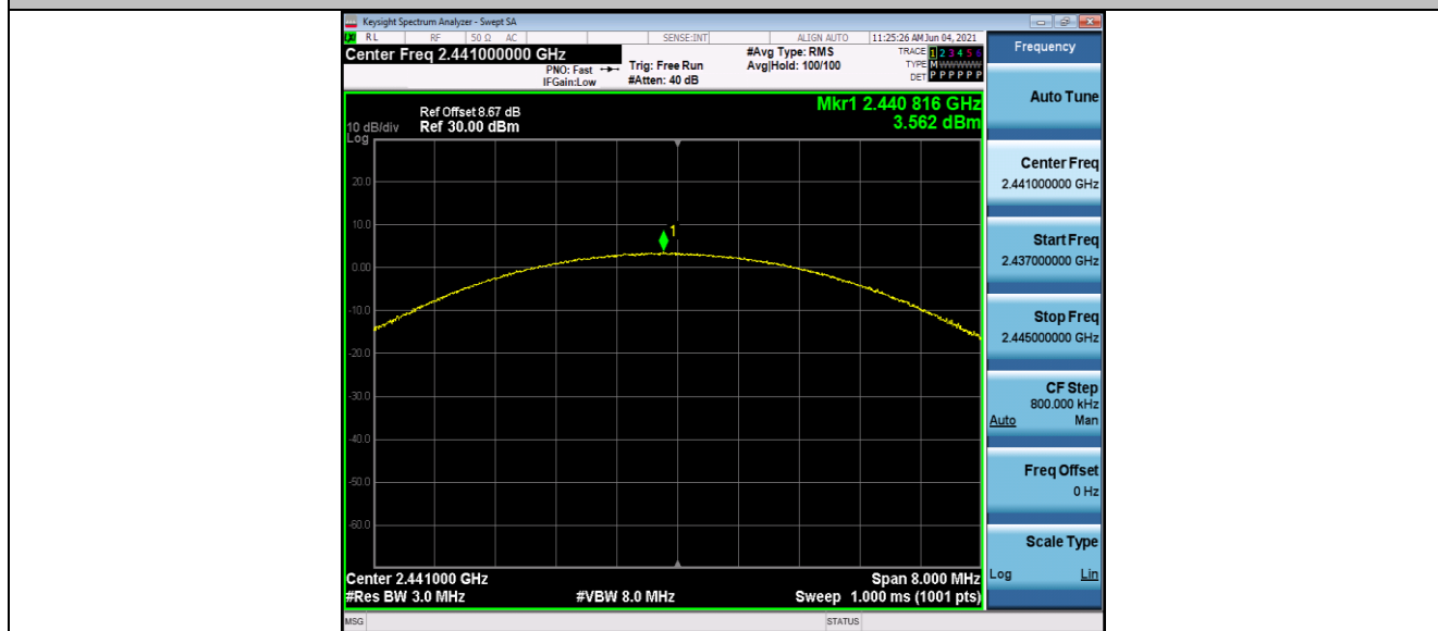
3DH5_Ant1_2441
