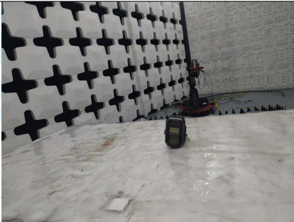
Radiated emission Above 1GHz Test Setup
