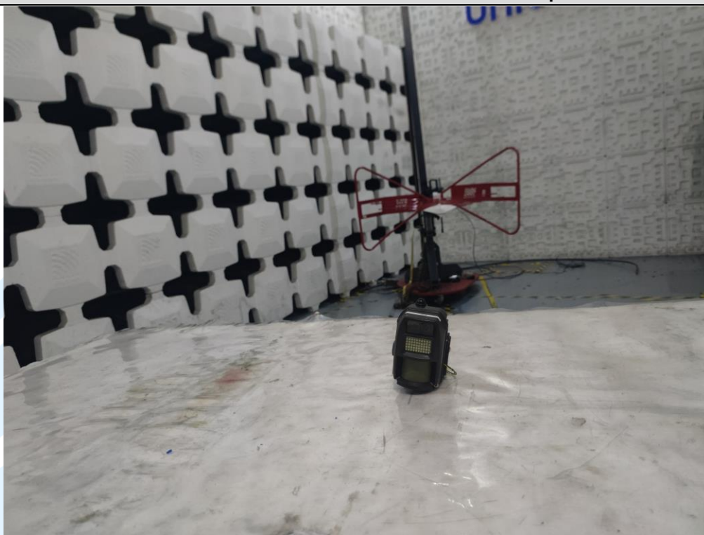
Radiated emission 30MHz to 1GHz Test Setup
