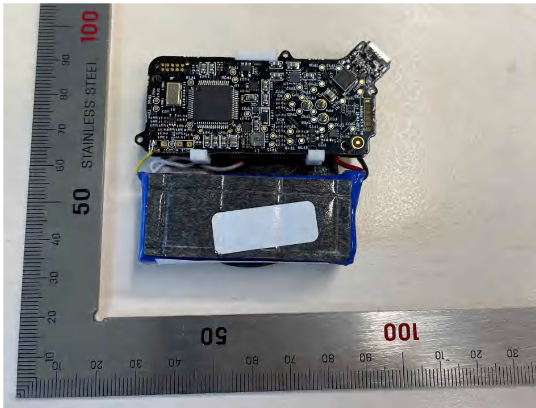
Figure 4 Internal electronics unit view with cover removed -2
