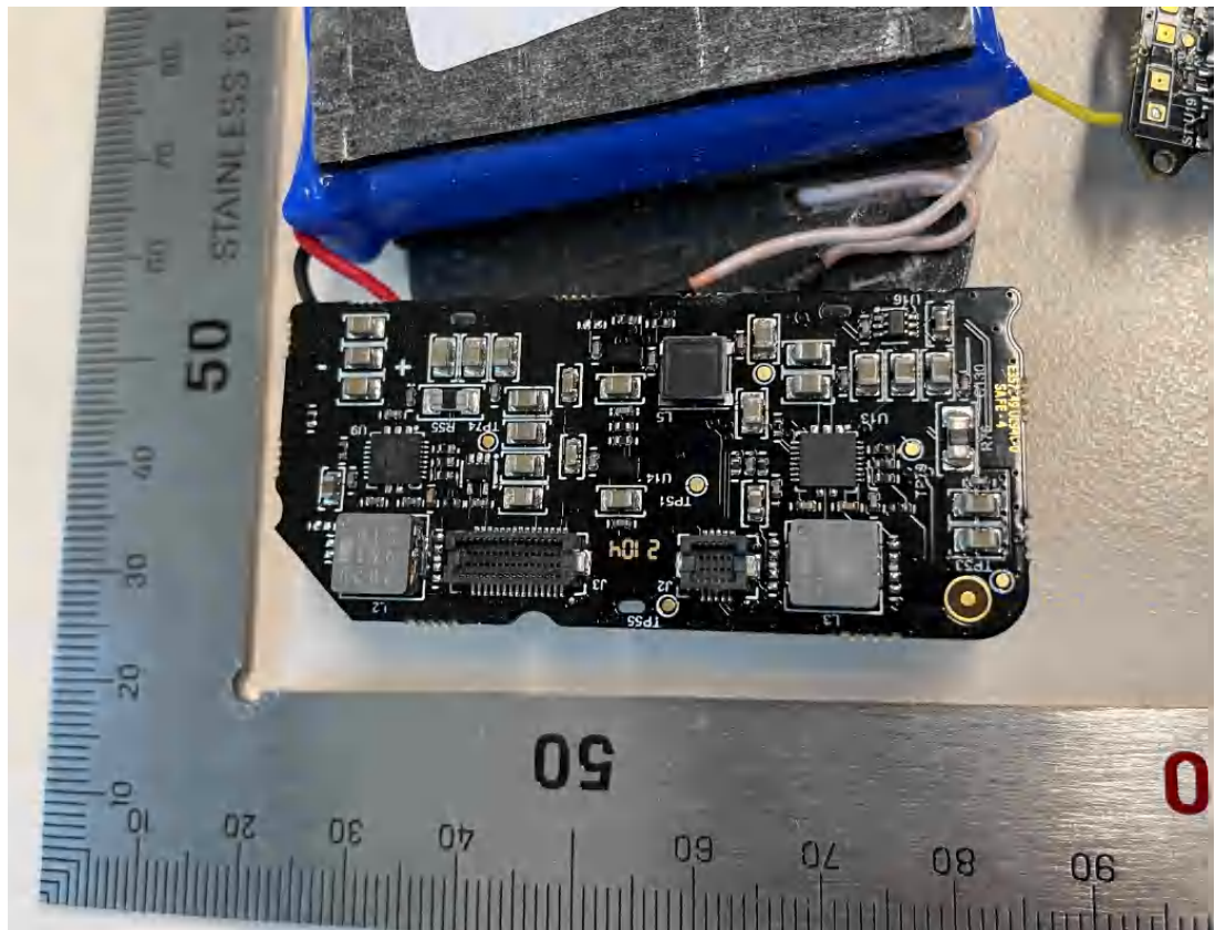
Figure 8 Internal electronics unit view with cover removed -6
