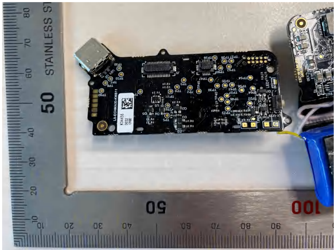
Figure 6 Internal electronics unit view with cover removed -4
