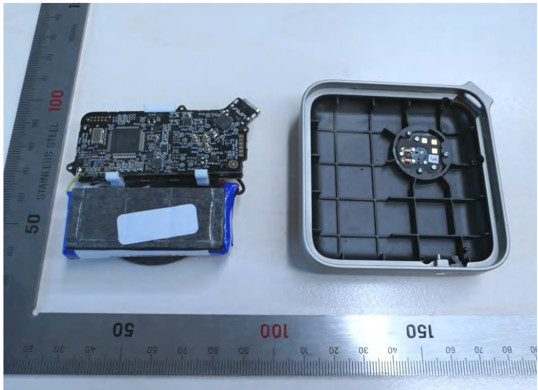
Figure 2 Internal view -2
