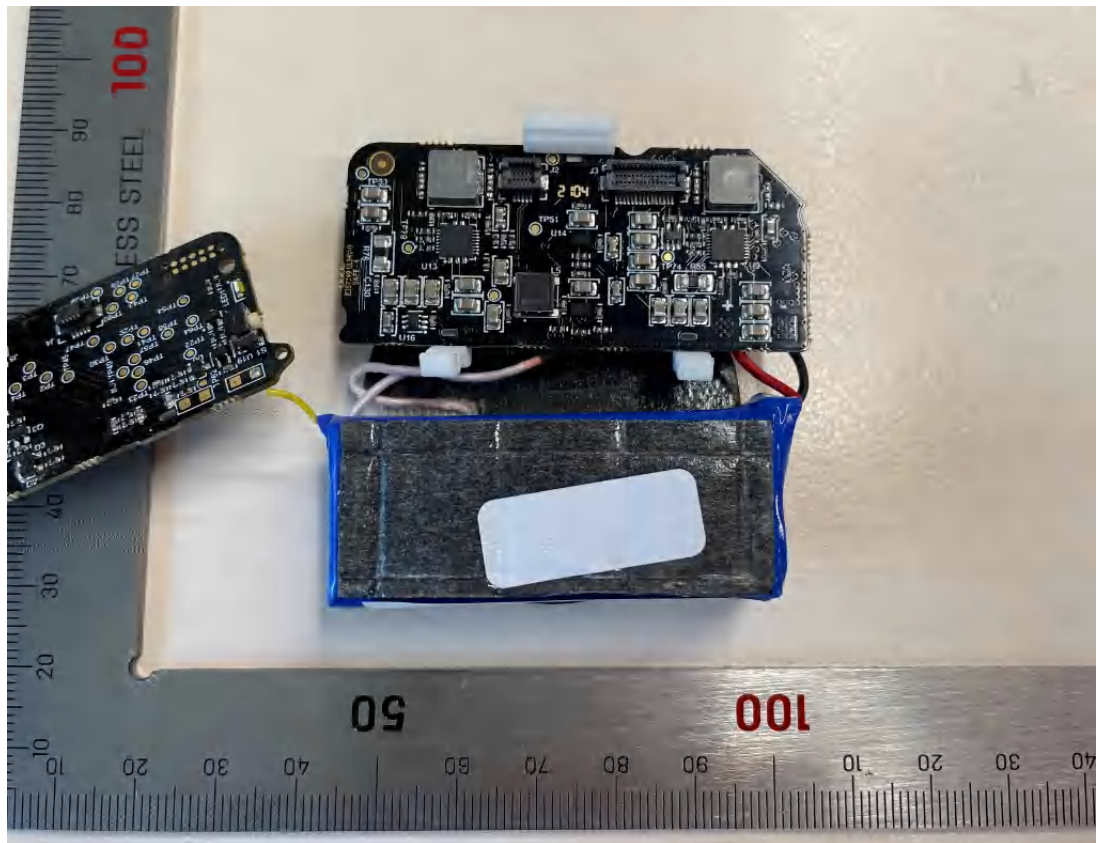
Figure 5 Internal electronics unit view with cover removed -3
