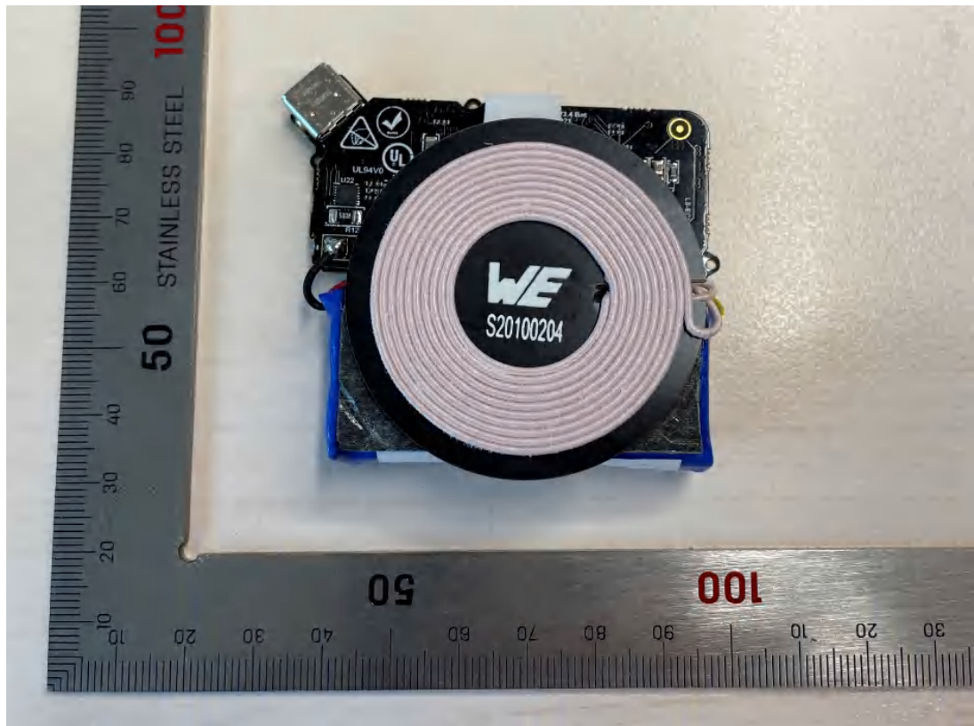
Figure 3 Internal electronics unit view with cover removed -1
