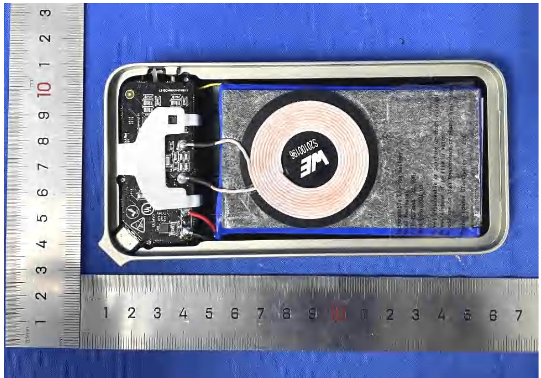
Figure 2 Internal view -2
