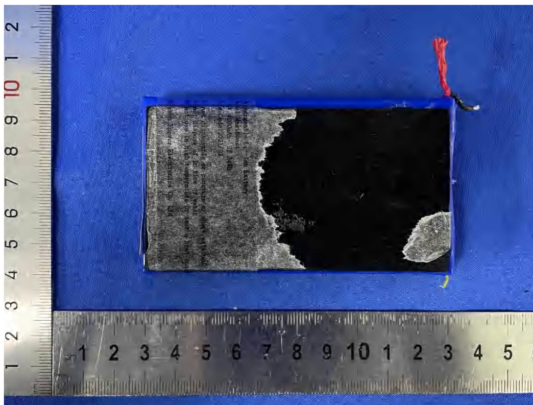
Figure 13 Battery view -1
