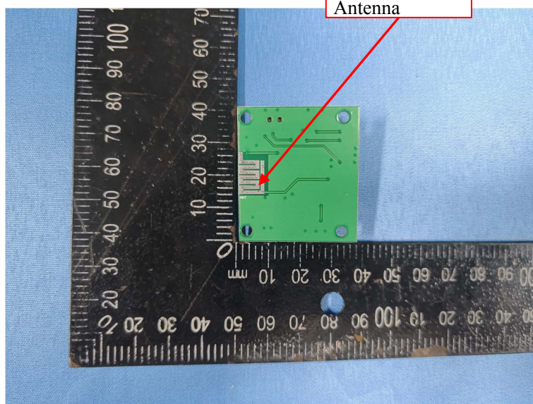
SRD 2.4G RX Antenna
