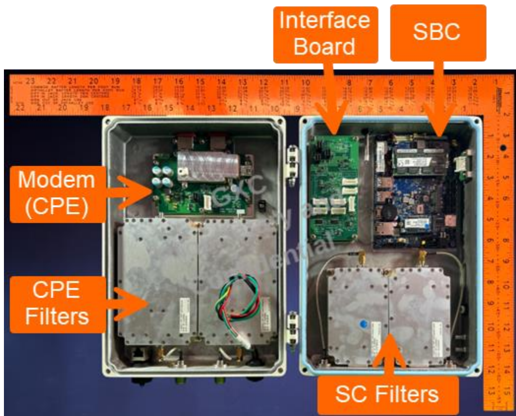
Figure 1 Internal Top View
