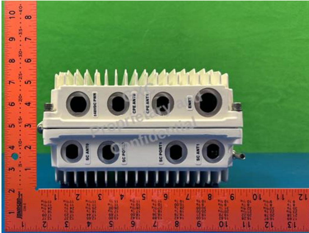
Figure 1 Antenna side view
