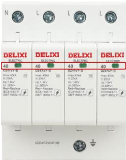
Fig. 6-1 surge protection device
