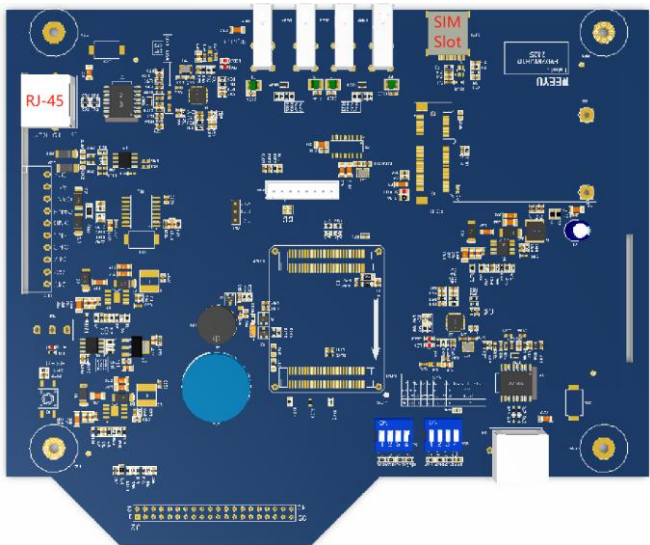
Fig. 5-6 RJ-45 Socket
