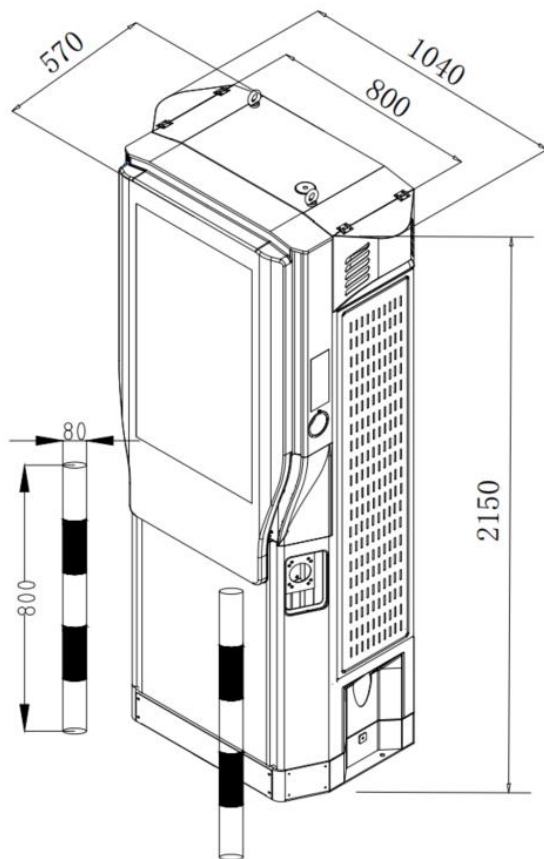
Fig. 5-1 Dimensions of Ampax
