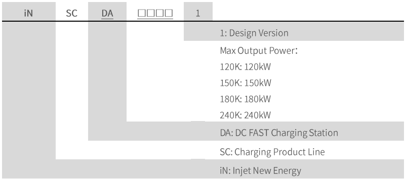
Fig. 4-3 Model definition of Ampax
