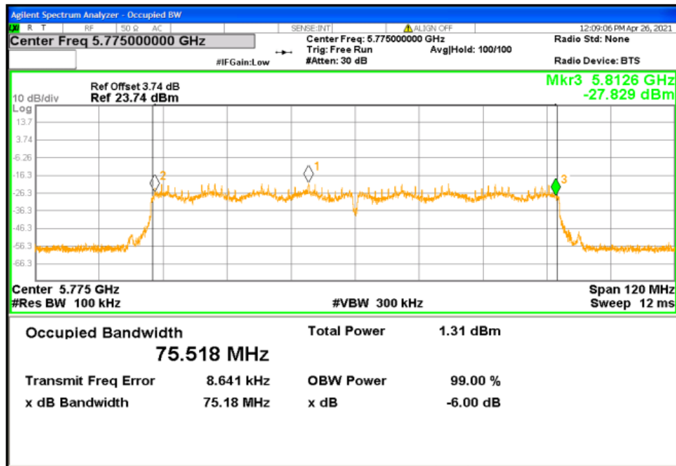
-6dB Bandwidth NVNT ac80 5775MHz Ant2
