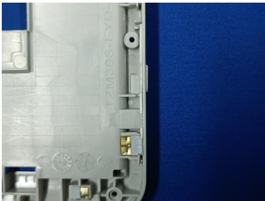
WIFI Antenna CLOSE VIEW
