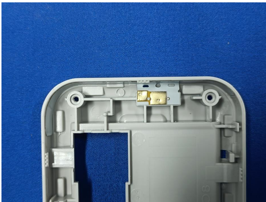
LTE Antenna CLOSE VIEW
