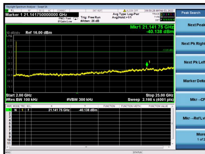
802.11b LOW CHANNEL, SPURIOUS 2 GHz ~ 25 GHz
