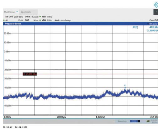
Band38-20MHz-QPSK-38150-1RB#0-Range3:3000~26500MHz
