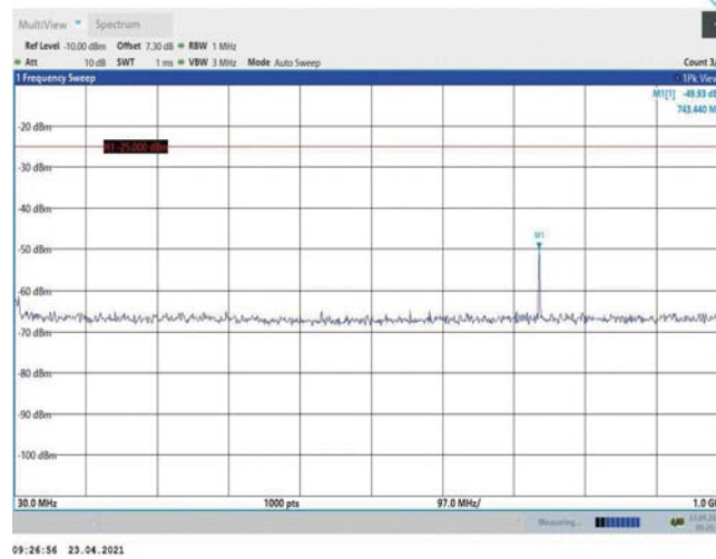
Band38-10MHz-QPSK-37800-1RB#0-Range1:30~1000MHz
