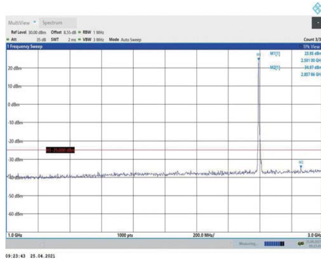
Band38-10MHz-QPSK-38000-1RB#0-Range2:1000~3000MHz
