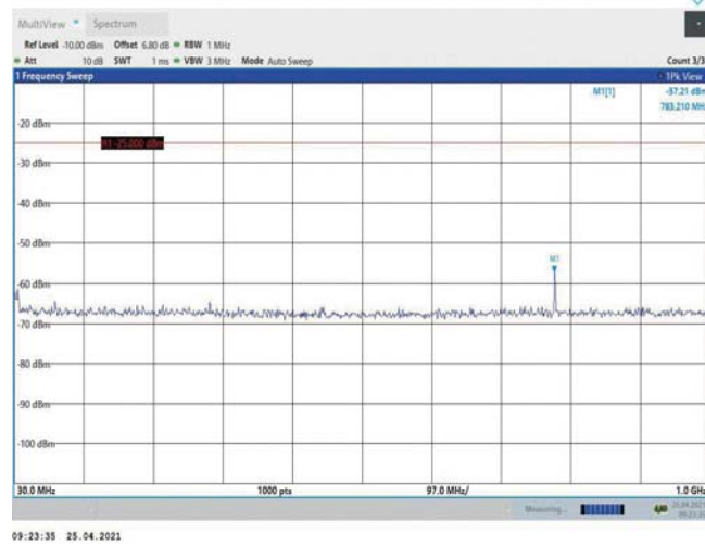
Band38-10MHz-QPSK-38000-1RB#0-Range1:30~1000MHz
