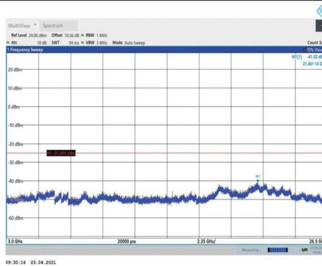
Band38-10MHz-16QAM-38200-1RB#0-Range3:3000~26500MHz
