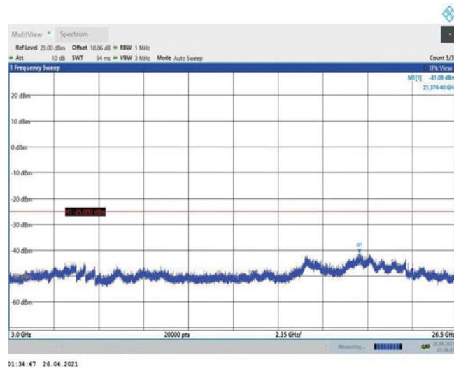
Band38-20MHz-QPSK-38000-1RB#0-Range3:3000~26500MHz
