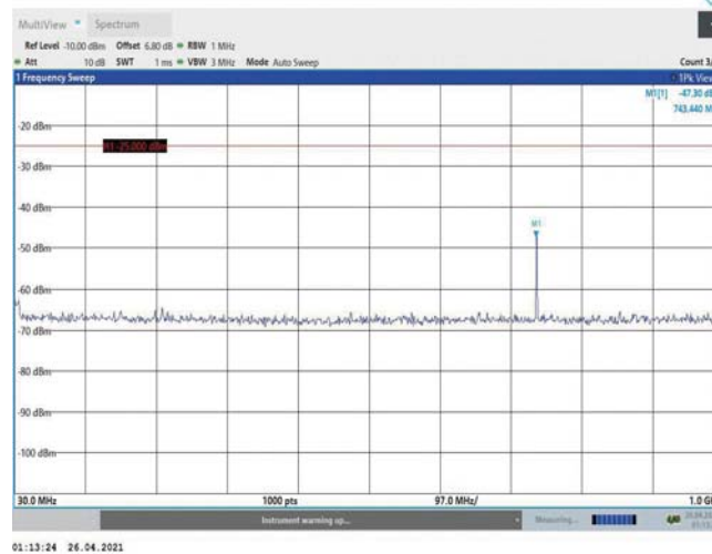
Band38-15MHz-16QAM-37825-1RB#0-Range1:30~1000MHz
