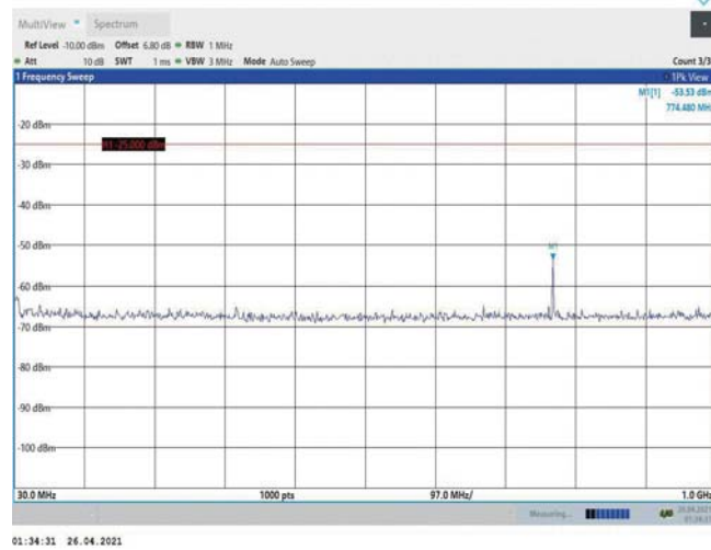
Band38-20MHz-QPSK-38000-1RB#0-Range1:30~1000MHz
