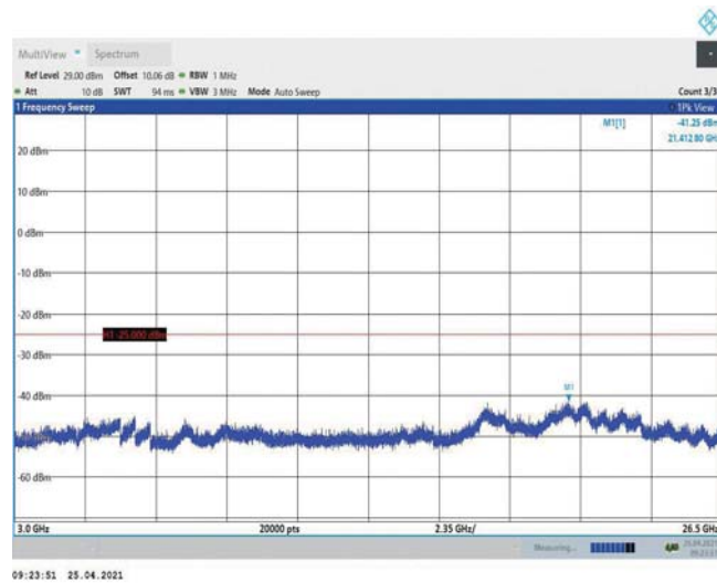
Band38-10MHz-QPSK-38000-1RB#0-Range3:3000~26500MHz
