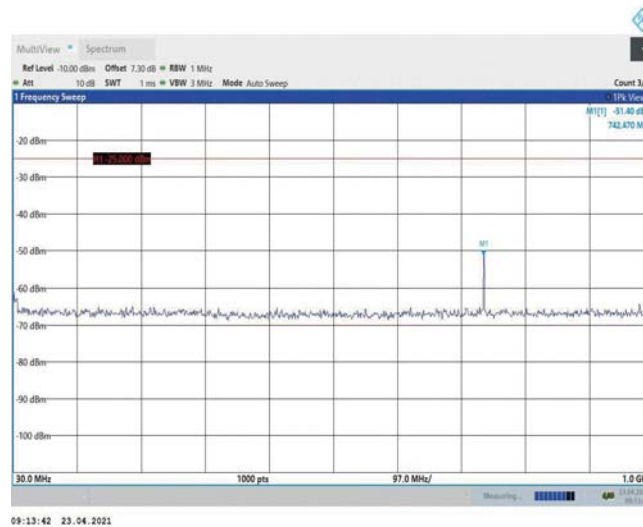
Band38-5MHz-QPSK-37775-1RB#0-Range1:30~1000MHz
