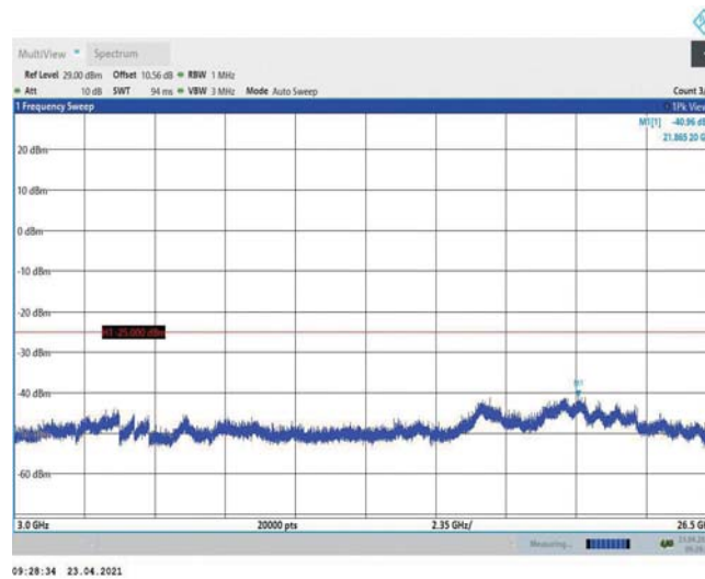
Band38-10MHz-QPSK-38000-1RB#0-Range3:3000~26500MHz
