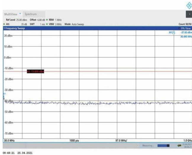
Band4-20MHz-16QAM-20300-1RB#0-Range1:30~1000MHz
