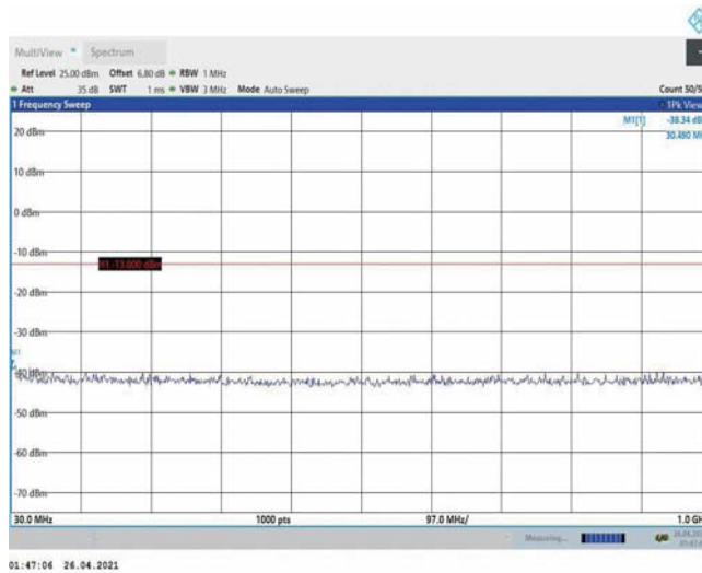
Band4-10MHz-16QAM-20175-1RB#0-Range1:30~1000MHz
