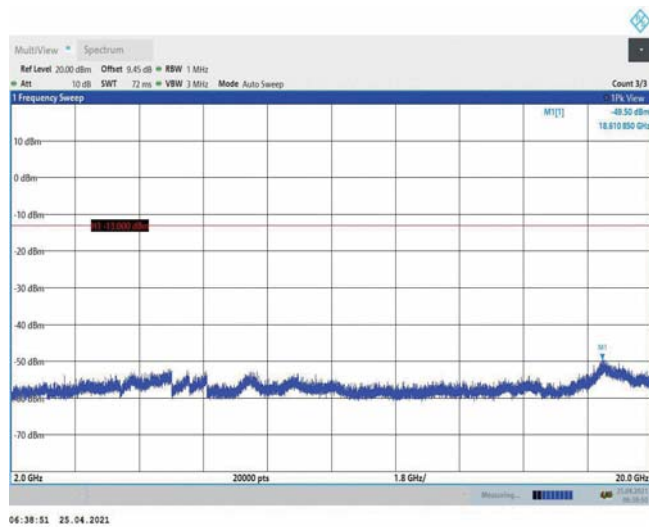
Band4-5MHz-16QAM-20375-1RB#0-Range3:2000~20000MHz
