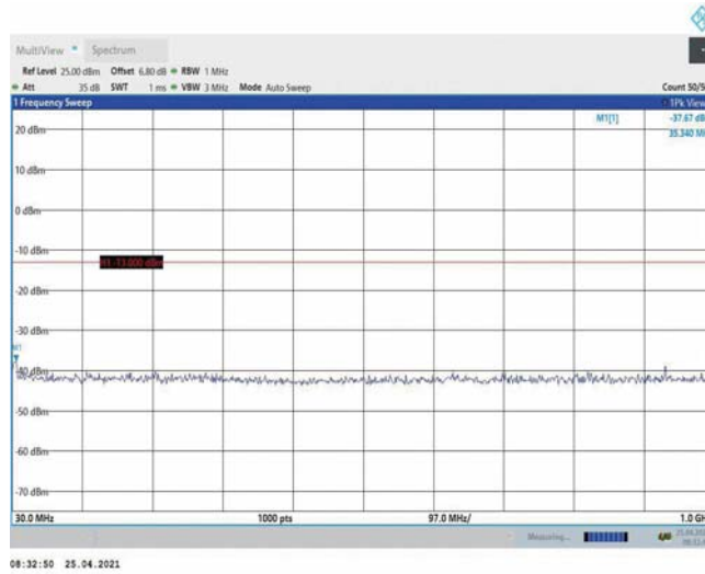
Band4-15MHz-QPSK-20175-1RB#0-Range1:30~1000MHz
