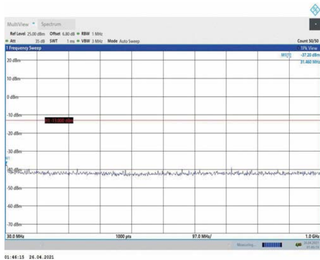
Band4-10MHz-16QAM-20000-1RB#0-Range1:30~1000MHz
