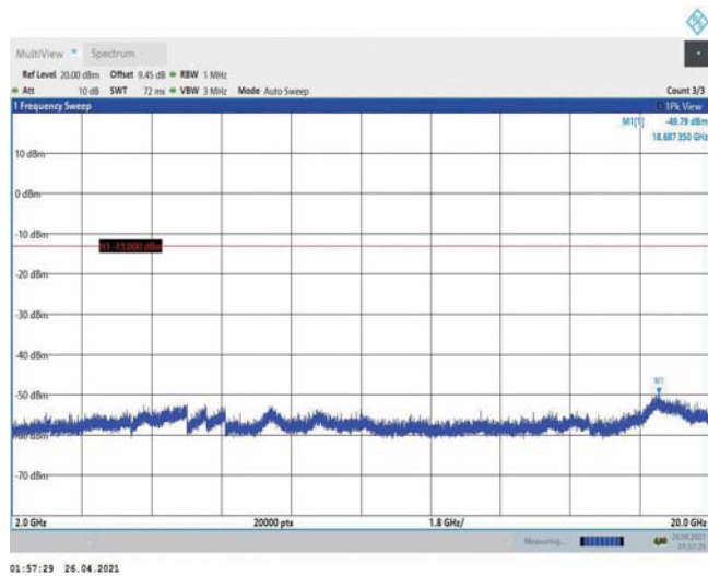
Band4-10MHz-QPSK-20350-1RB#0-Range3:2000~20000MHz
