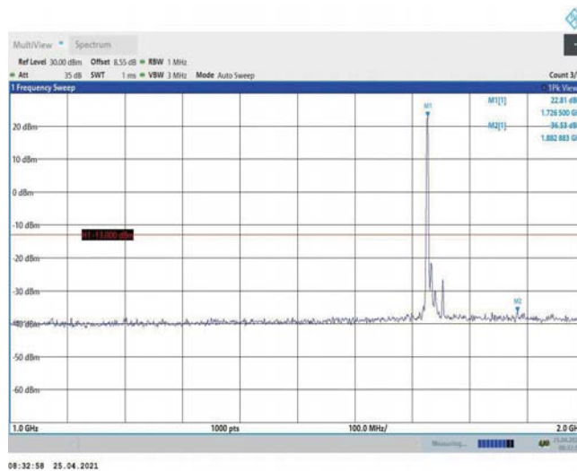
Band4-15MHz-QPSK-20175-1RB#0-Range2:1000~2000MHz
