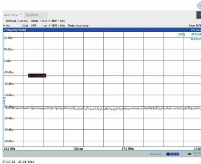
Band4-10MHz-16QAM-20000-1RB#0-Range1:30~1000MHz
