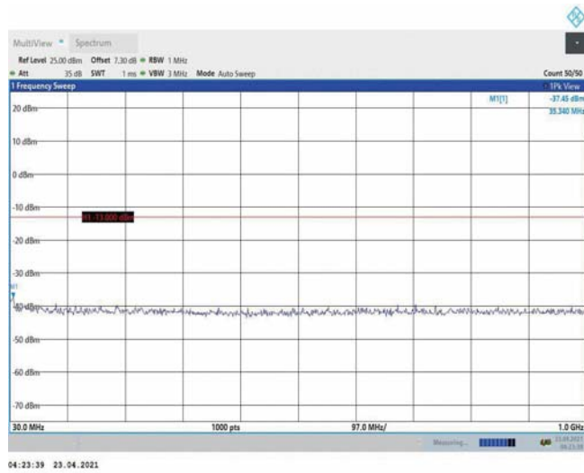
Band4-3MHz-16QAM-20385-1RB#0-Range1:30~1000MHz
