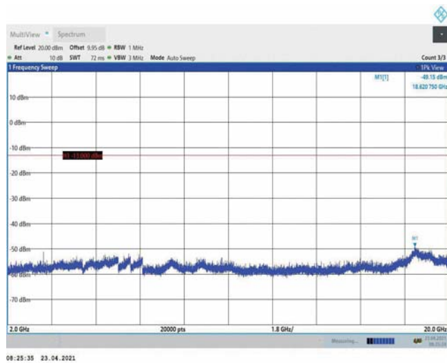
Band4-15MHz-16QAM-20175-1RB#0-Range3:2000~20000MHz
