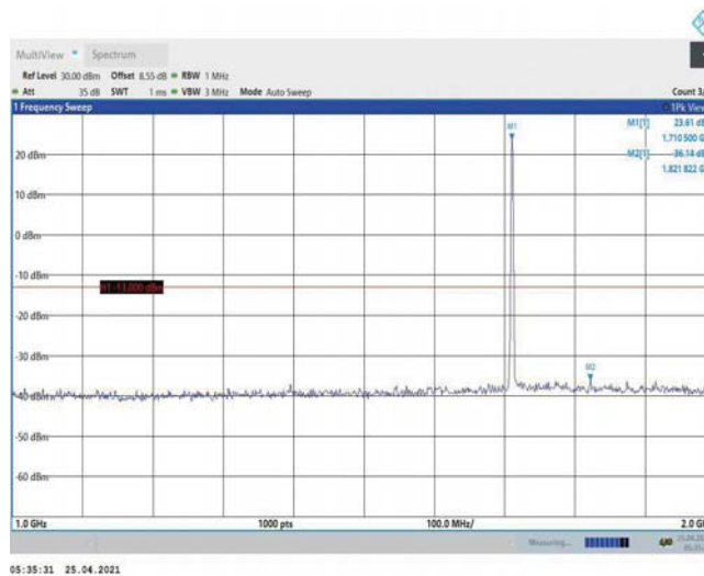
Band4-1.4MHz-16QAM-19957-1RB#0-Range2:1000~2000MHz
