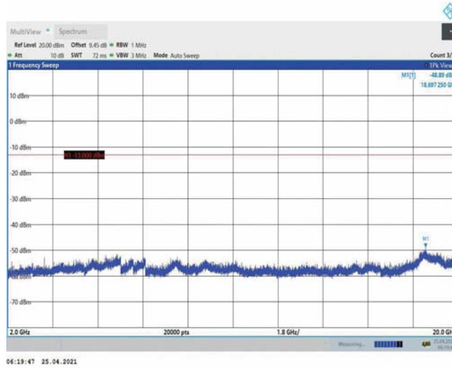
Band4-3MHz-QPSK-20175-1RB#0-Range3:2000~20000MHz
