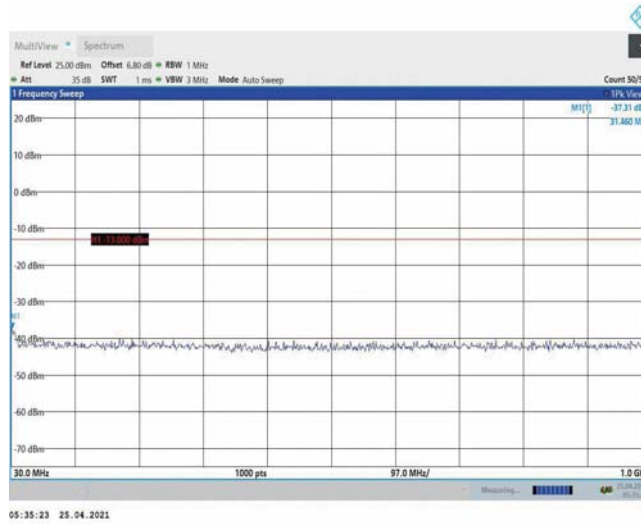
Band4-1.4MHz-16QAM-19957-1RB#0-Range1:30~1000MHz
