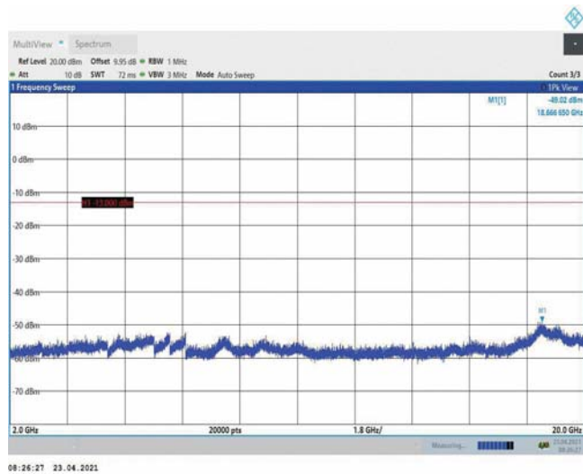
Band4-15MHz-16QAM-20325-1RB#0-Range3:2000~20000MHz
