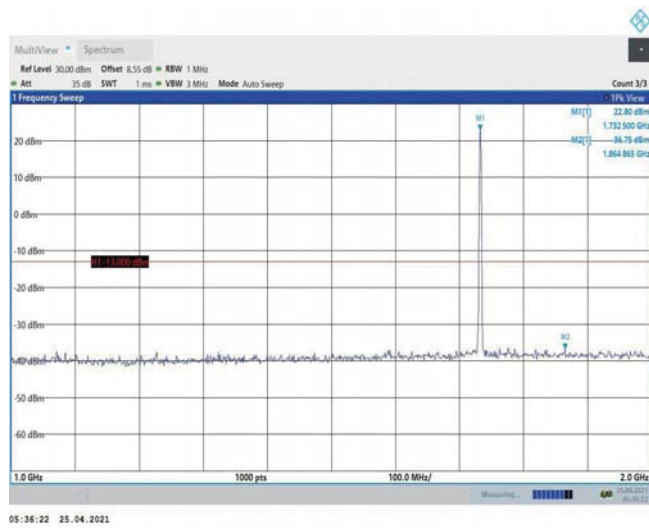
Band4-1.4MHz-16QAM-20175-1RB#0-Range2:1000~2000MHz
