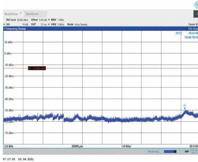
Band4-10MHz-QPSK-20000-1RB#0-Range3:2000~20000MHz
