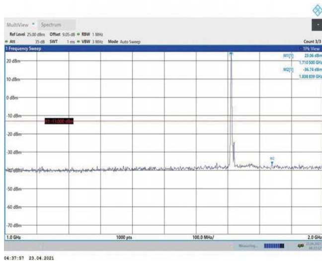
Band4-5MHz-16QAM-19975-1RB#0-Range2:1000~2000MHz
