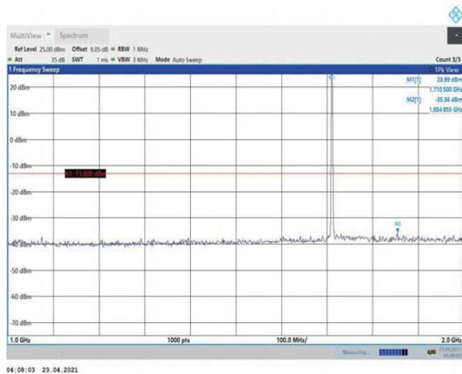
Band4-1.4MHz-16QAM-19957-1RB#0-Range2:1000~2000MHz
