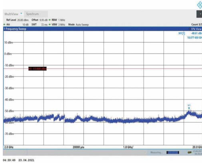
Band4-5MHz-16QAM-20375-1RB#0-Range3:2000~20000MHz
