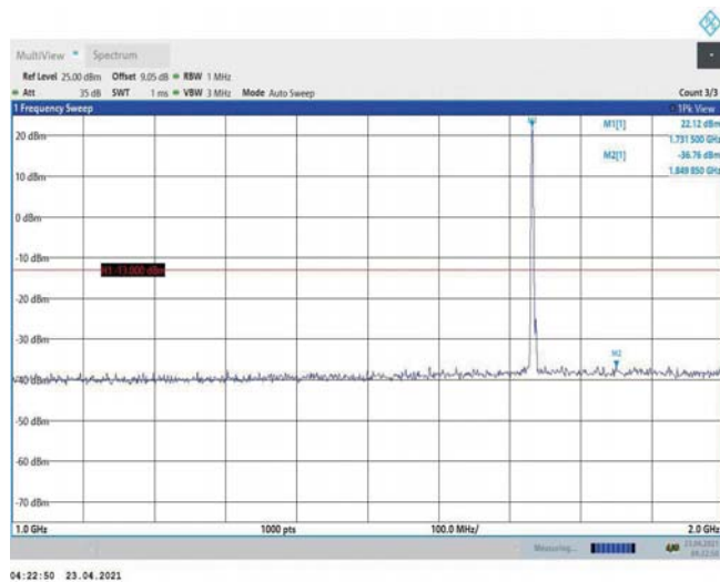
Band4-3MHz-16QAM-20175-1RB#0-Range2:1000~2000MHz
