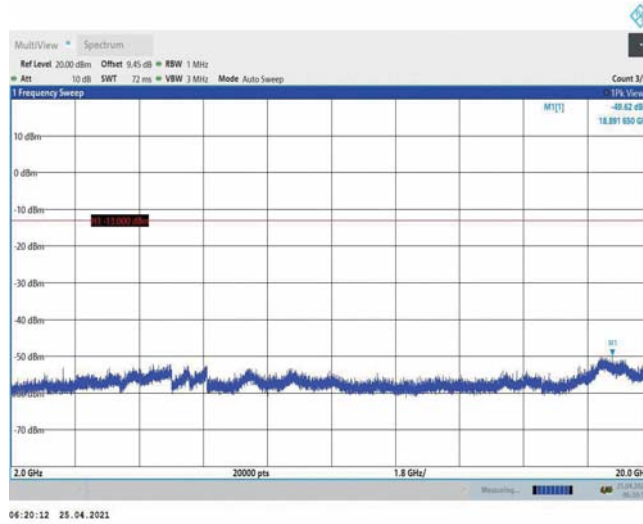
Band4-3MHz-16QAM-20175-1RB#0-Range3:2000~20000MHz
