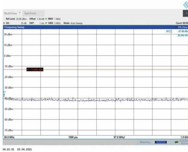
Band4-3MHz-16QAM-19965-1RB#0-Range1:30~1000MHz
