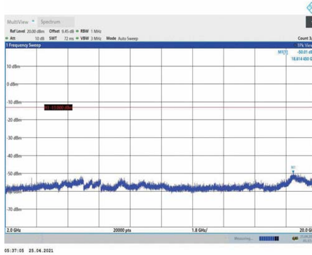
Band4-1.4MHz-QPSK-20393-1RB#0-Range3:2000~20000MHz
