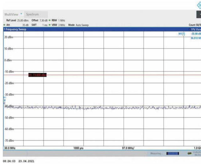
Band4-15MHz-QPSK-20025-1RB#0-Range1:30~1000MHz
