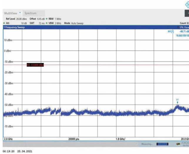
Band4-3MHz-16QAM-19965-1RB#0-Range3:2000~20000MHz
