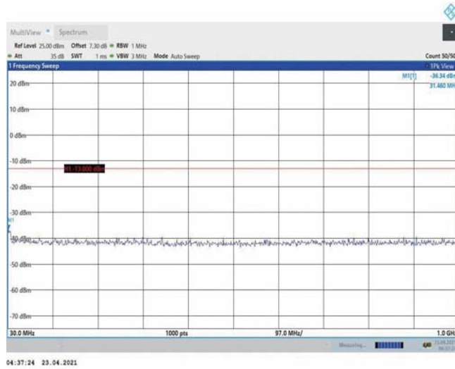
Band4-5MHz-QPSK-19975-1RB#0-Range1:30~1000MHz
