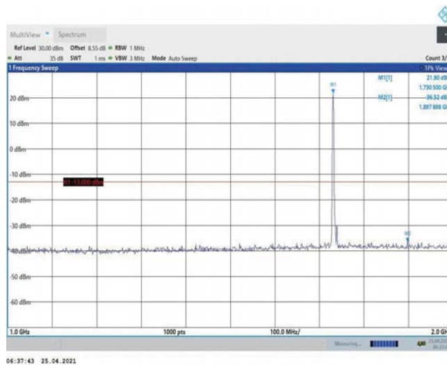
Band4-5MHz-16QAM-20175-1RB#0-Range2:1000~2000MHz
