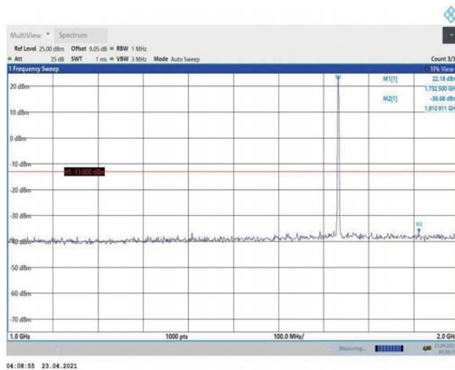
Band4-1.4MHz-16QAM-20175-1RB#0-Range2:1000~2000MHz
