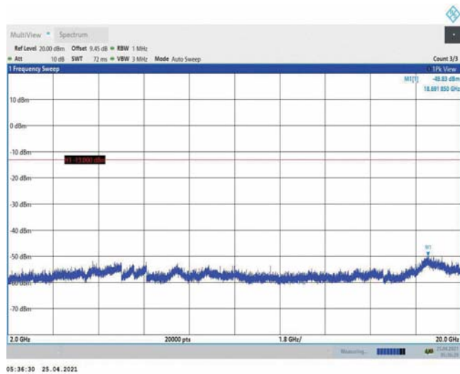
Band4-1.4MHz-16QAM-20175-1RB#0-Range3:2000~20000MHz
