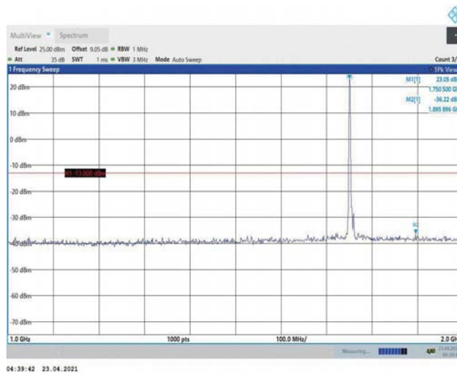
Band4-5MHz-16QAM-20375-1RB#0-Range2:1000~2000MHz
