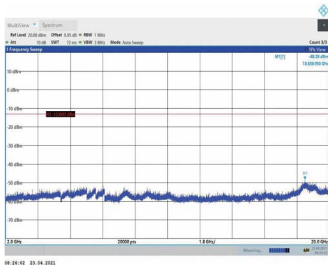
Band4-15MHz-QPSK-20325-1RB#0-Range3:2000~20000MHz
