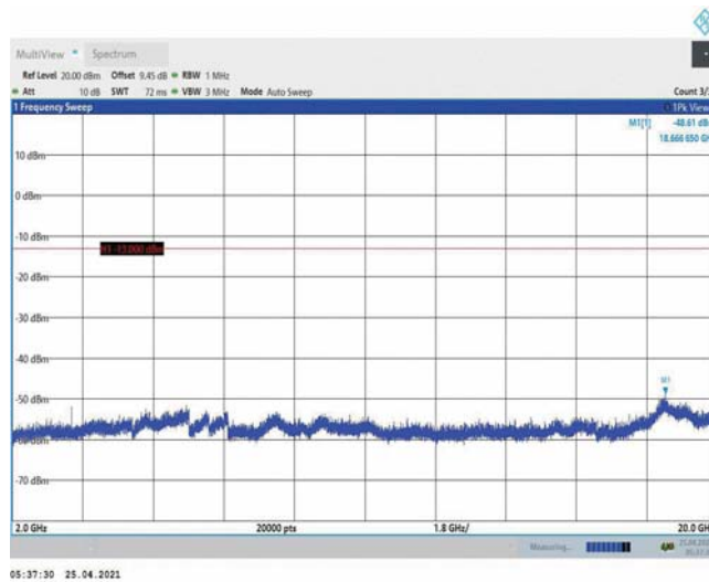
Band4-1.4MHz-16QAM-20393-1RB#0-Range3:2000~20000MHz
