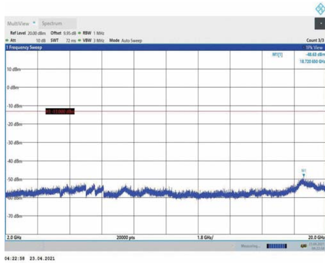
Band4-3MHz-16QAM-20175-1RB#0-Range3:2000~20000MHz
