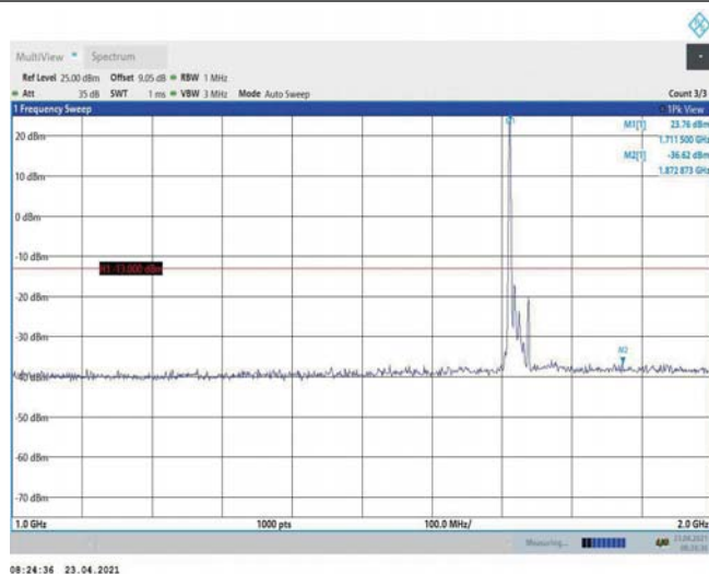
Band4-15MHz-16QAM-20025-1RB#0-Range2:1000~2000MHz
