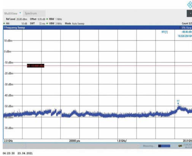
Band4-3MHz-QPSK-20385-1RB#0-Range3:2000~20000MHz
