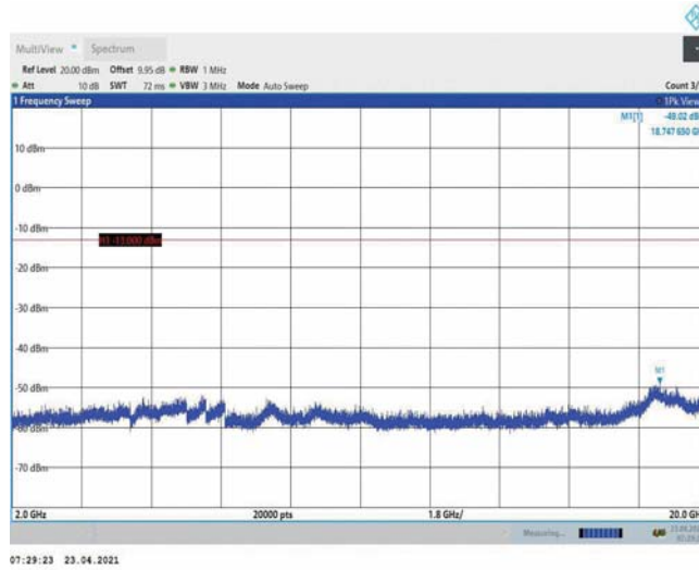
Band4-10MHz-16QAM-20350-1RB#0-Range3:2000~20000MHz
