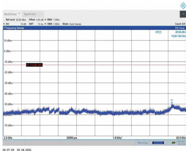
Band4-5MHz-QPSK-20175-1RB#0-Range3:2000~20000MHz
