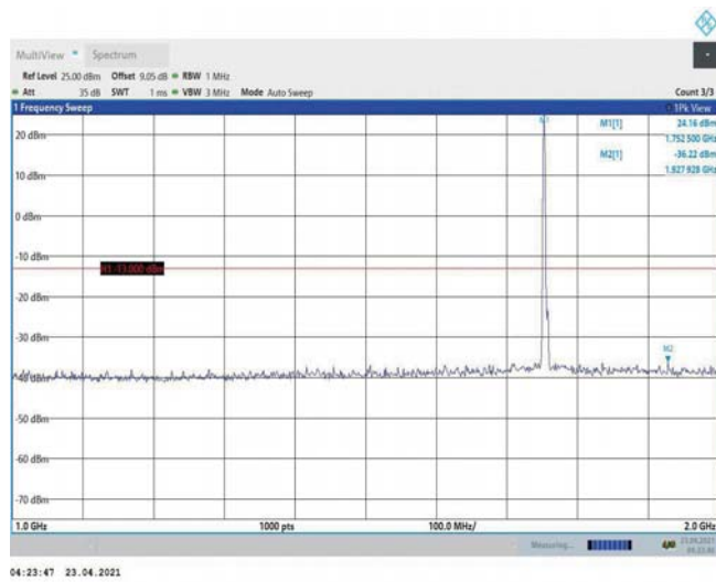
Band4-3MHz-16QAM-20385-1RB#0-Range2:1000~2000MHz
