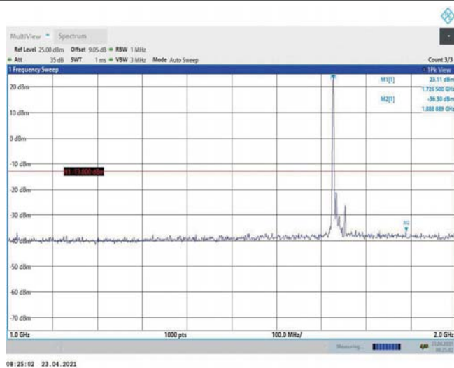
Band4-15MHz-QPSK-20175-1RB#0-Range2:1000~2000MHz
