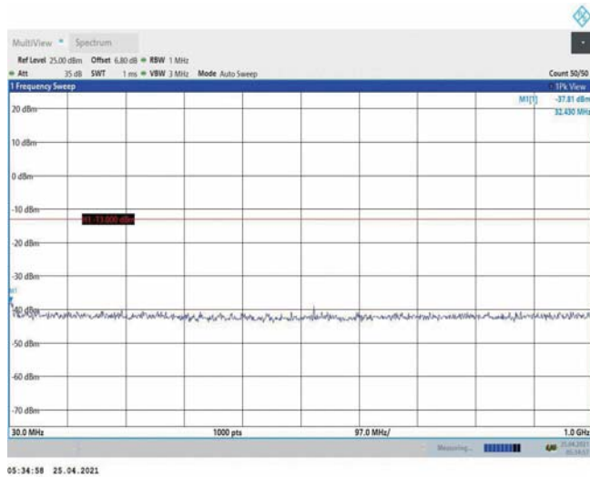
Band4-1.4MHz-QPSK-19957-1RB#0-Range1:30~1000MHz
