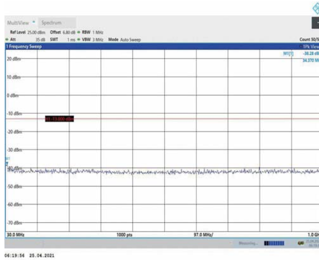
Band4-3MHz-16QAM-20175-1RB#0-Range1:30~1000MHz
