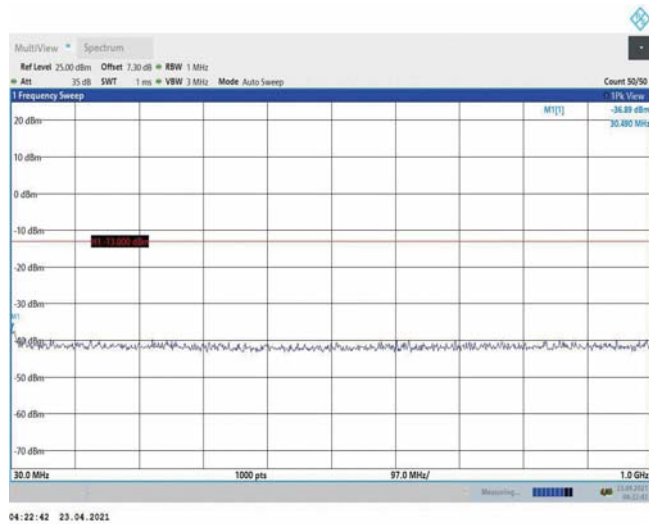
Band4-3MHz-16QAM-20175-1RB#0-Range1:30~1000MHz
