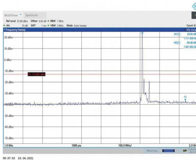
Band4-20MHz-16QAM-20050-1RB#0-Range2:1000~2000MHz
