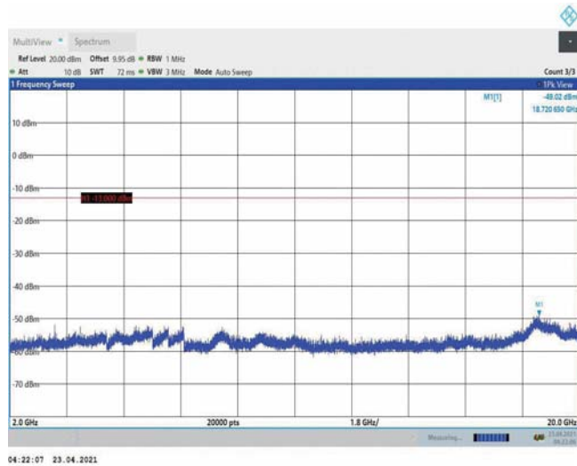
Band4-3MHz-16QAM-19965-1RB#0-Range3:2000~20000MHz
