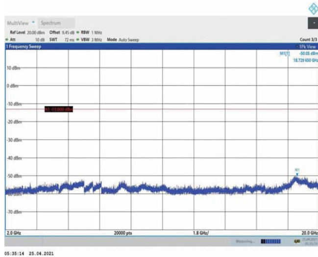
Band4-1.4MHz-QPSK-19957-1RB#0-Range3:2000~20000MHz
