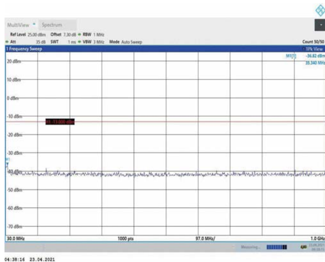
Band4-5MHz-QPSK-20175-1RB#0-Range1:30~1000MHz
