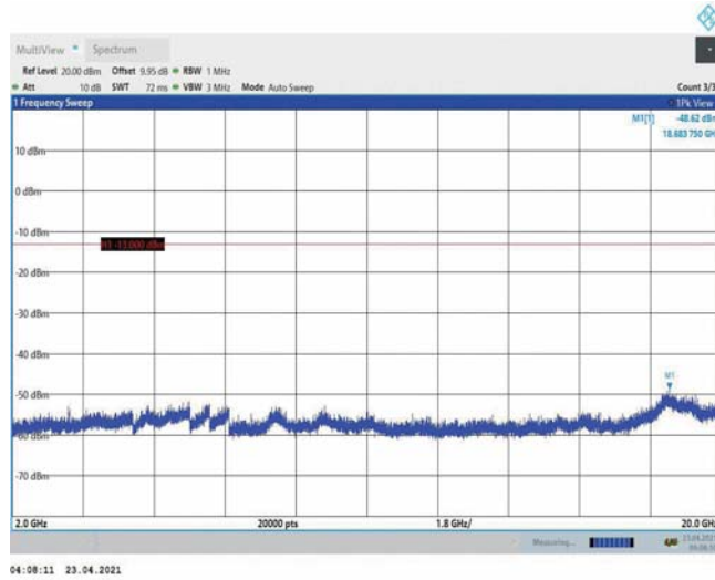
Band4-1.4MHz-16QAM-19957-1RB#0-Range3:2000~20000MHz
