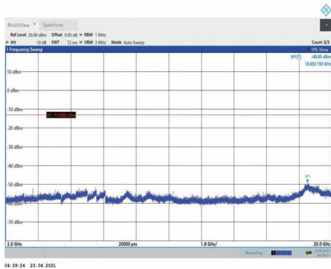
Band4-5MHz-QPSK-20375-1RB#0-Range3:2000~20000MHz
