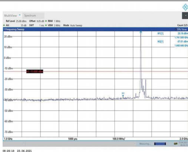
Band4-15MHz-16QAM-20325-1RB#0-Range2:1000~2000MHz
