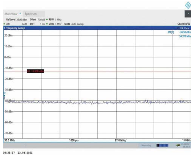
Band4-20MHz-16QAM-20175-1RB#0-Range1:30~1000MHz
