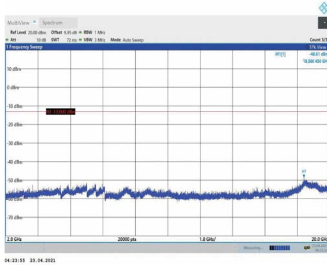
Band4-3MHz-16QAM-20385-1RB#0-Range3:2000~20000MHz
