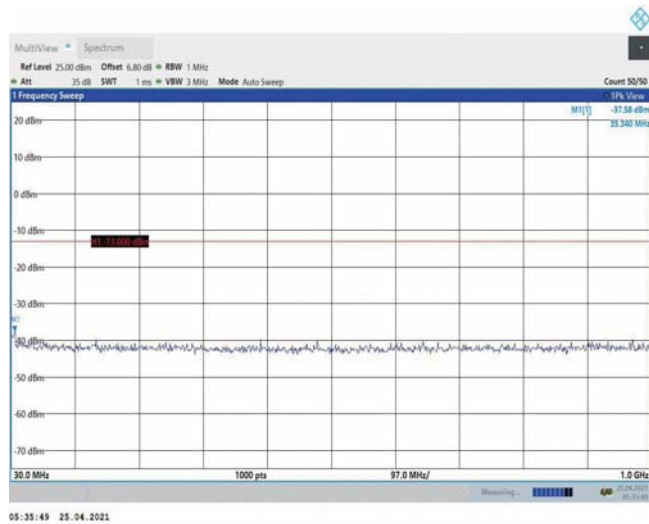
Band4-1.4MHz-QPSK-20175-1RB#0-Range1:30~1000MHz
