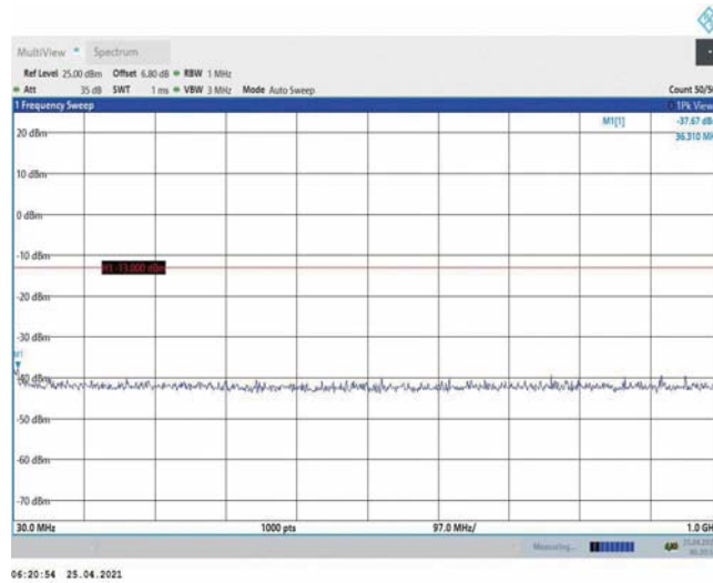
Band4-3MHz-16QAM-20385-1RB#0-Range1:30~1000MHz
