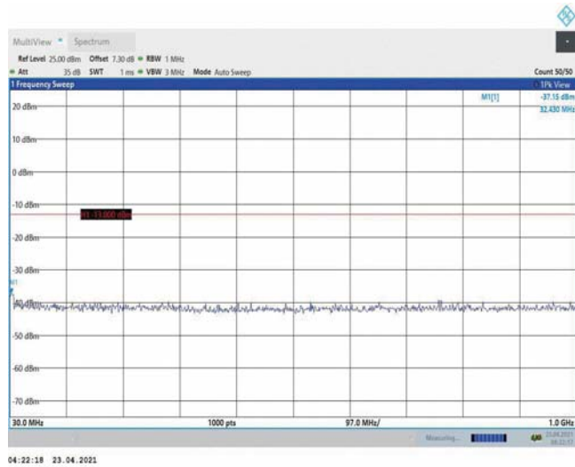
Band4-3MHz-QPSK-20175-1RB#0-Range1:30~1000MHz
