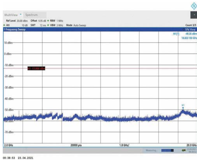
Band4-20MHz-16QAM-20175-1RB#0-Range3:2000~20000MHz
