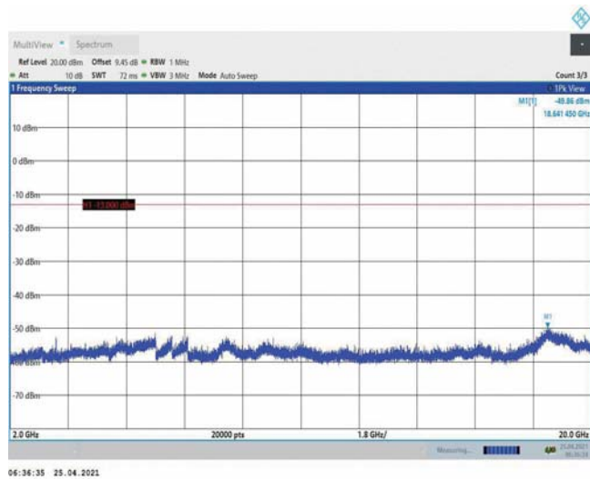
Band4-5MHz-QPSK-19975-1RB#0-Range3:2000~20000MHz
