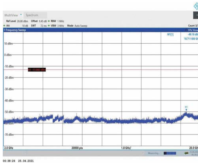
Band4-5MHz-QPSK-20375-1RB#0-Range3:2000~20000MHz
