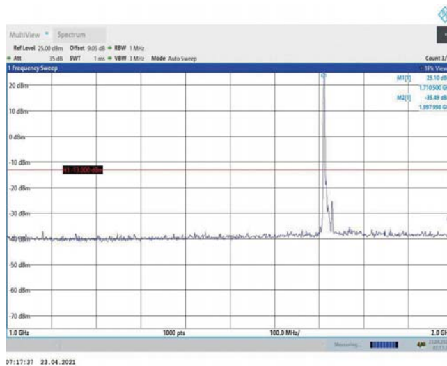
Band4-10MHz-16QAM-20000-1RB#0-Range2:1000~2000MHz
