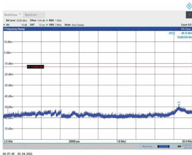
Band4-5MHz-QPSK-19975-1RB#0-Range3:2000~20000MHz
