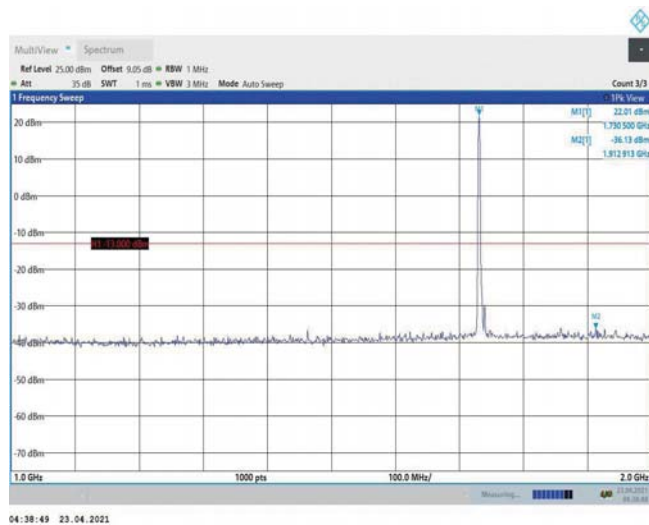
Band4-5MHz-16QAM-20175-1RB#0-Range2:1000~2000MHz
