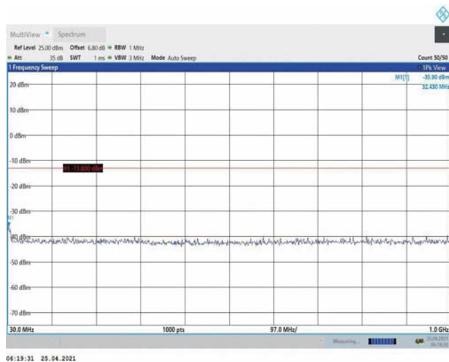
Band4-3MHz-QPSK-20175-1RB#0-Range1:30~1000MHz
