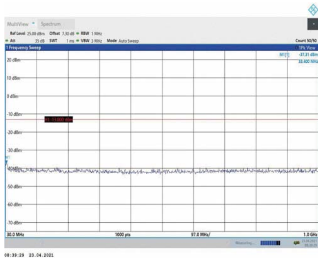
Band4-20MHz-16QAM-20300-1RB#0-Range1:30~1000MHz
