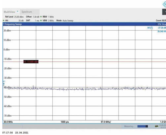
Band4-10MHz-QPSK-20175-1RB#0-Range1:30~1000MHz
