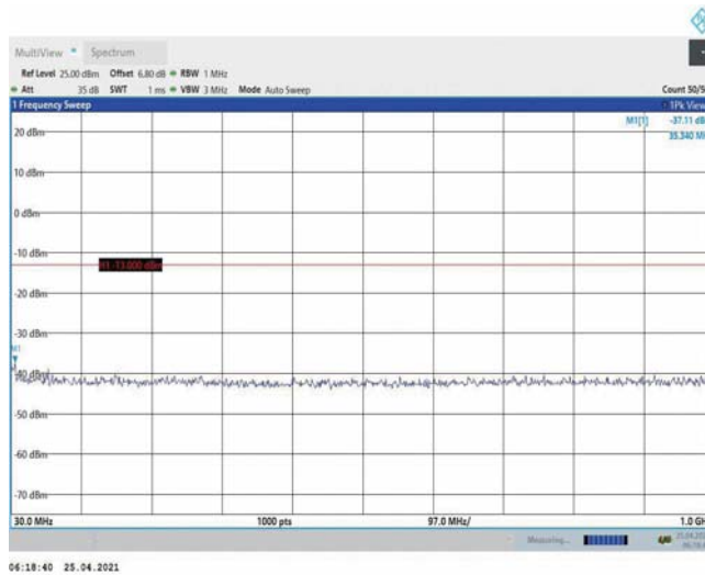
Band4-3MHz-QPSK-19965-1RB#0-Range1:30~1000MHz
