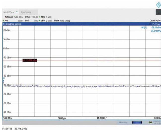
Band4-5MHz-QPSK-20375-1RB#0-Range1:30~1000MHz
