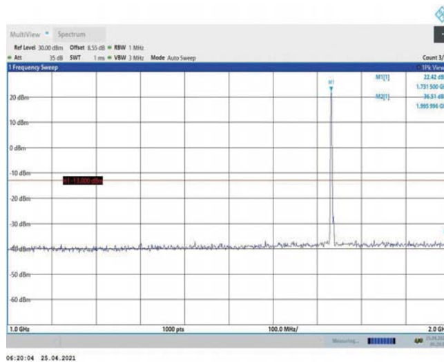
Band4-3MHz-16QAM-20175-1RB#0-Range2:1000~2000MHz
