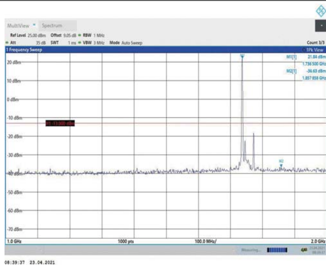
Band4-20MHz-16QAM-20300-1RB#0-Range2:1000~2000MHz
