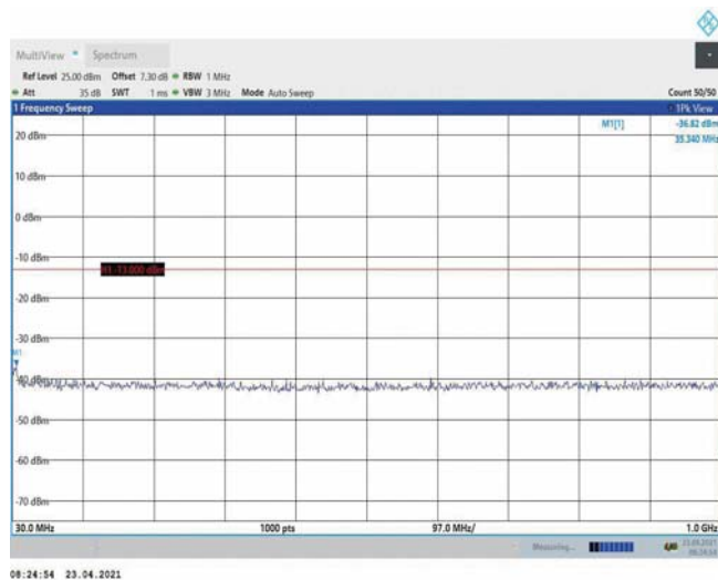
Band4-15MHz-QPSK-20175-1RB#0-Range1:30~1000MHz
