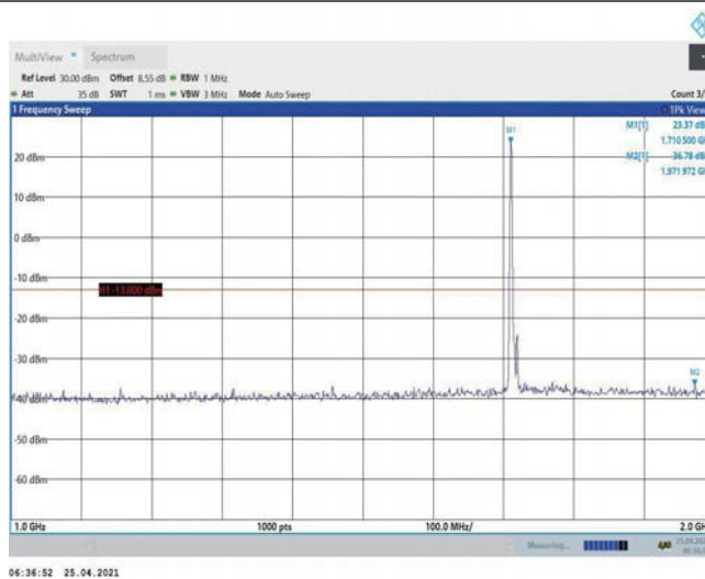
Band4-5MHz-16QAM-19975-1RB#0-Range2:1000~2000MHz
