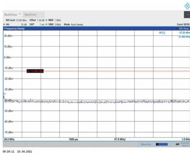
Band4-15MHz-16QAM-20325-1RB#0-Range1:30~1000MHz
