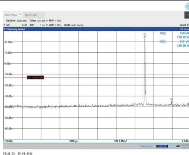
Band4-3MHz-16QAM-20385-1RB#0-Range2:1000~2000MHz
