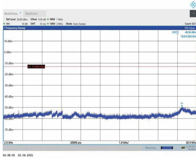
Band4-5MHz-16QAM-19975-1RB#0-Range3:2000~20000MHz
