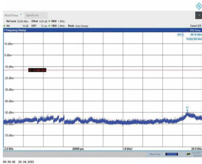
Band4-20MHz-16QAM-20300-1RB#0-Range3:2000~20000MHz
