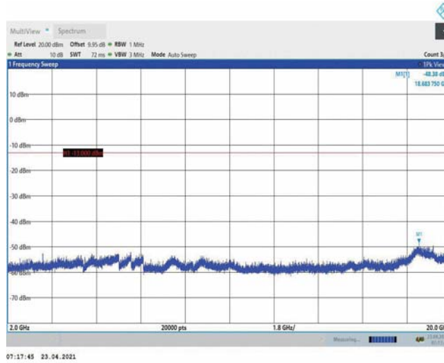
Band4-10MHz-16QAM-20000-1RB#0-Range3:2000~20000MHz
