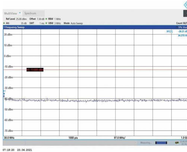
Band4-10MHz-16QAM-20175-1RB#0-Range1:30~1000MHz
