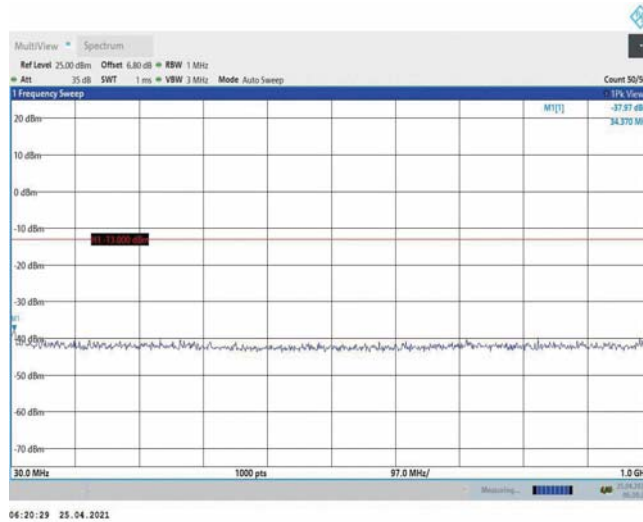
Band4-3MHz-QPSK-20385-1RB#0-Range1:30~1000MHz
