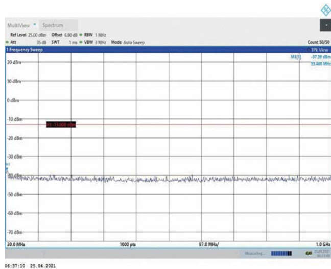
Band4-5MHz-QPSK-20175-1RB#0-Range1:30~1000MHz
