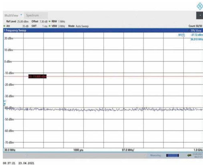
Band4-20MHz-QPSK-20050-1RB#0-Range1:30~1000MHz
