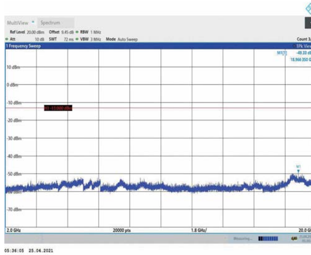
Band4-1.4MHz-QPSK-20175-1RB#0-Range3:2000~20000MHz
