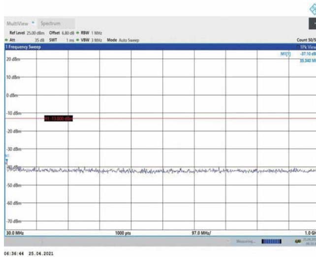
Band4-5MHz-16QAM-19975-1RB#0-Range1:30~1000MHz
