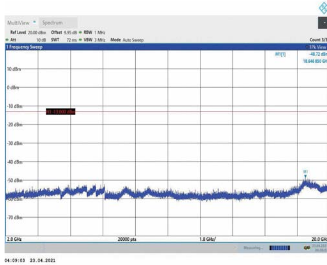
Band4-1.4MHz-16QAM-20175-1RB#0-Range3:2000~20000MHz
