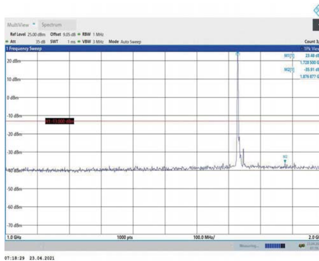
Band4-10MHz-16QAM-20175-1RB#0-Range2:1000~2000MHz
