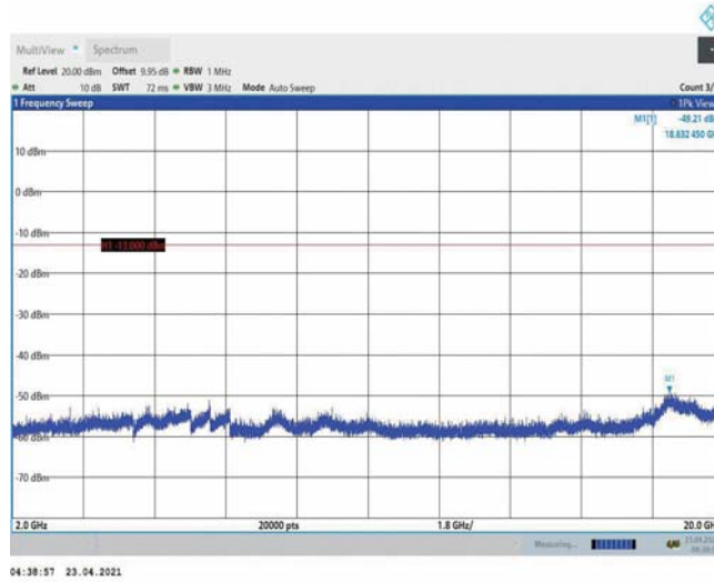
Band4-5MHz-16QAM-20175-1RB#0-Range3:2000~20000MHz
