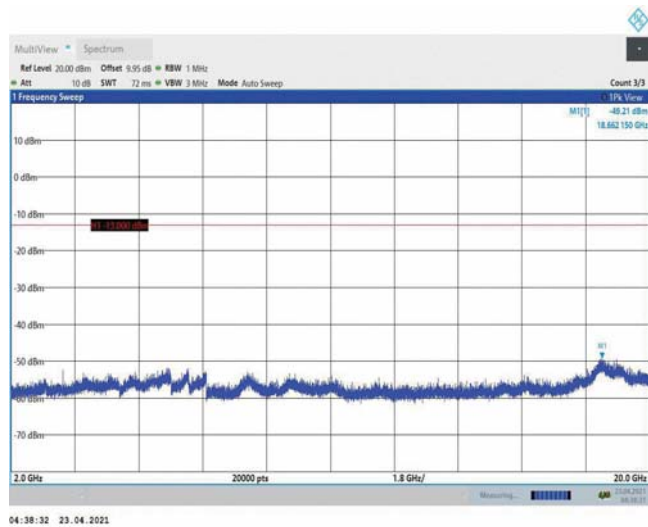
Band4-5MHz-QPSK-20175-1RB#0-Range3:2000~20000MHz
