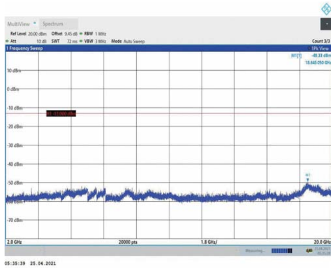
Band4-1.4MHz-16QAM-19957-1RB#0-Range3:2000~20000MHz
