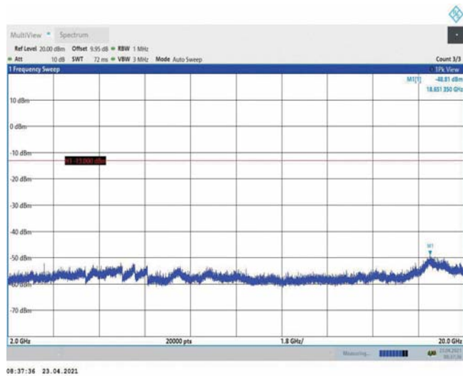
Band4-20MHz-QPSK-20050-1RB#0-Range3:2000~20000MHz
