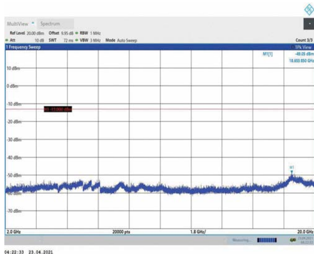
Band4-3MHz-QPSK-20175-1RB#0-Range3:2000~20000MHz
