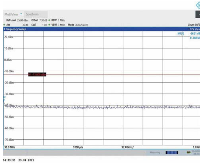
Band4-5MHz-16QAM-20375-1RB#0-Range1:30~1000MHz
