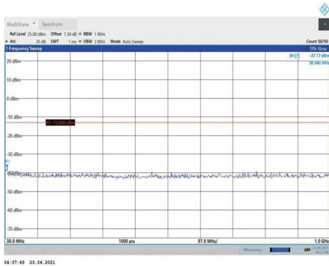
Band4-5MHz-16QAM-19975-1RB#0-Range1:30~1000MHz
