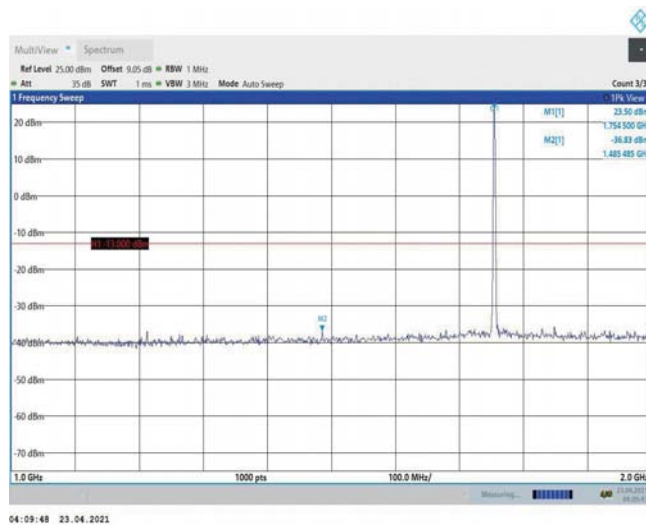
Band4-1.4MHz-16QAM-20393-1RB#0-Range2:1000~2000MHz
