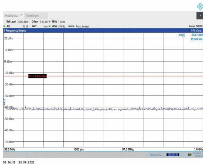
Band4-15MHz-16QAM-20025-1RB#0-Range1:30~1000MHz
