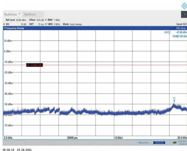
Band4-15MHz-QPSK-20025-1RB#0-Range3:2000~20000MHz
