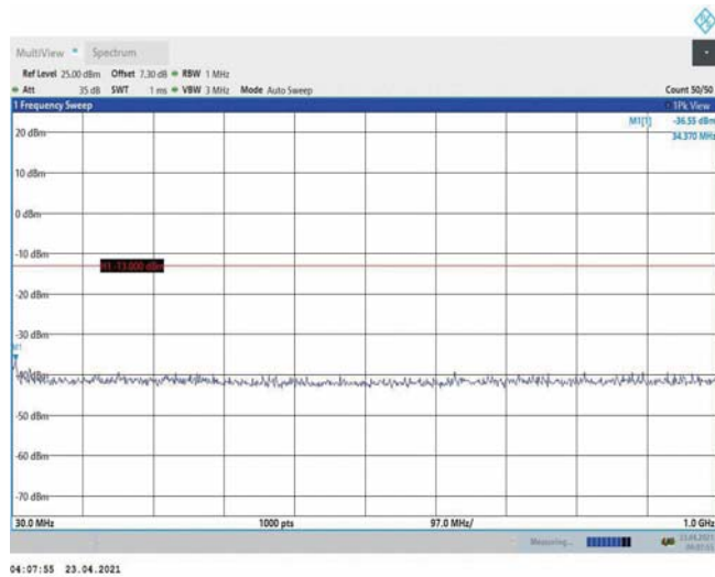
Band4-1.4MHz-16QAM-19957-1RB#0-Range1:30~1000MHz
