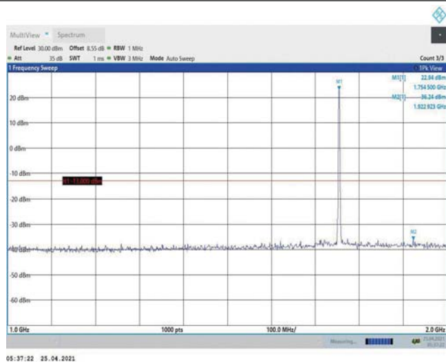
Band4-1.4MHz-16QAM-20393-1RB#0-Range2:1000~2000MHz
