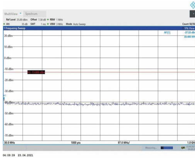
Band4-1.4MHz-16QAM-20393-1RB#0-Range1:30~1000MHz
