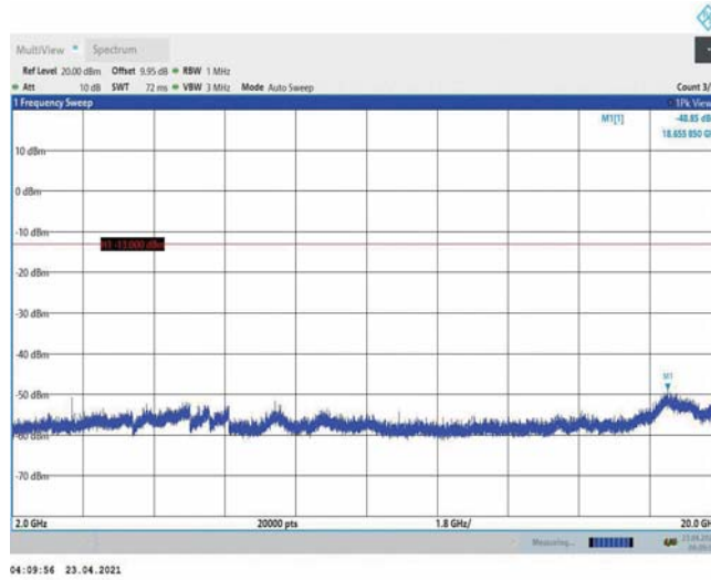
Band4-1.4MHz-16QAM-20393-1RB#0-Range3:2000~20000MHz
