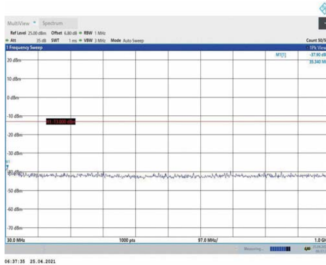
Band4-5MHz-16QAM-20175-1RB#0-Range1:30~1000MHz
