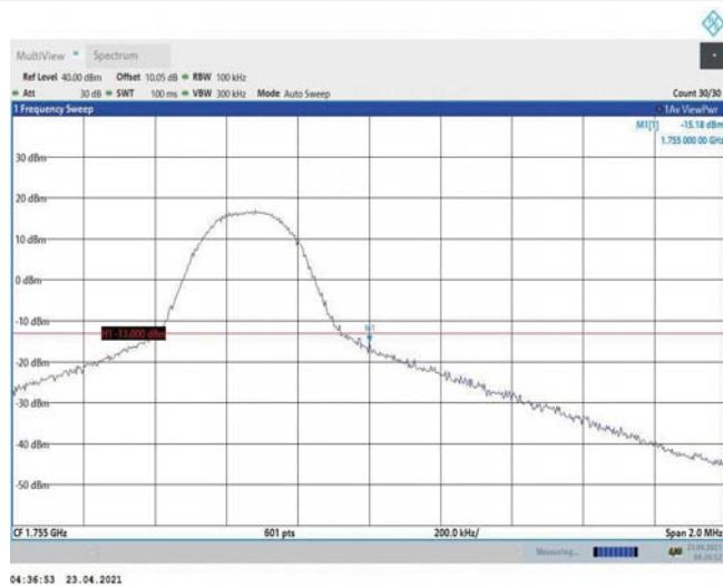
Band4-5MHz-16QAM-20375-1RB#24
