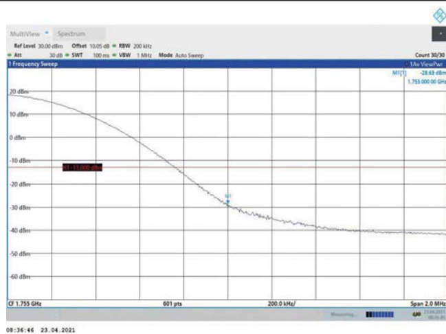
Band4-20MHz-16QAM-20300-1RB#99
