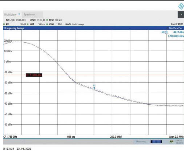
Band4-15MHz-QPSK-20325-1RB#74
