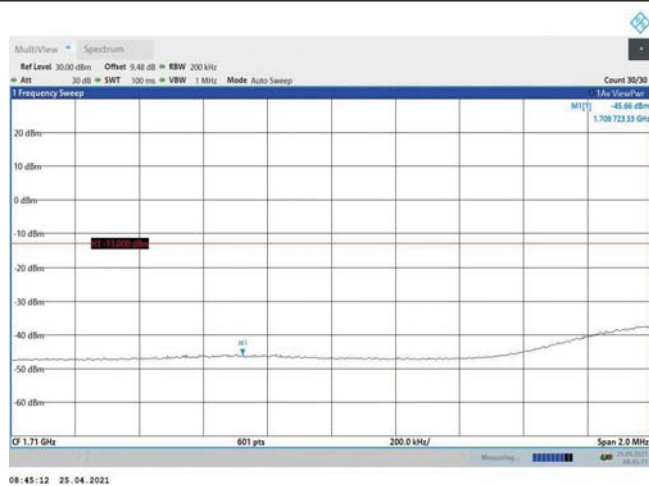
Band4-20MHz-16QAM-20050-1RB#99
