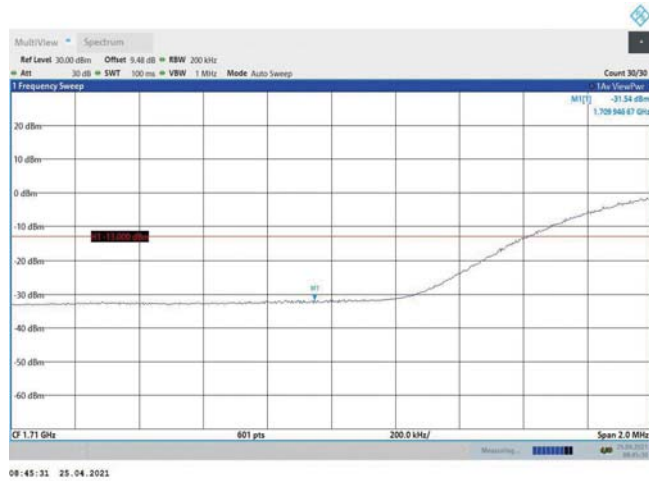
Band4-20MHz-16QAM-20050-100RB#0
