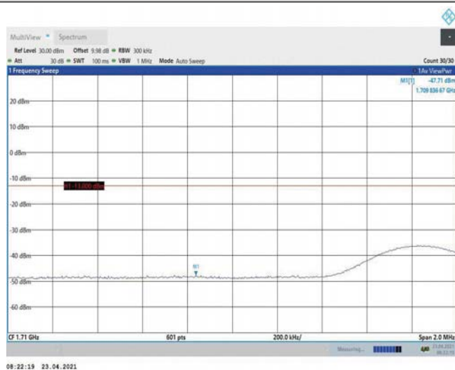
Band4-15MHz-QPSK-20025-1RB#74
