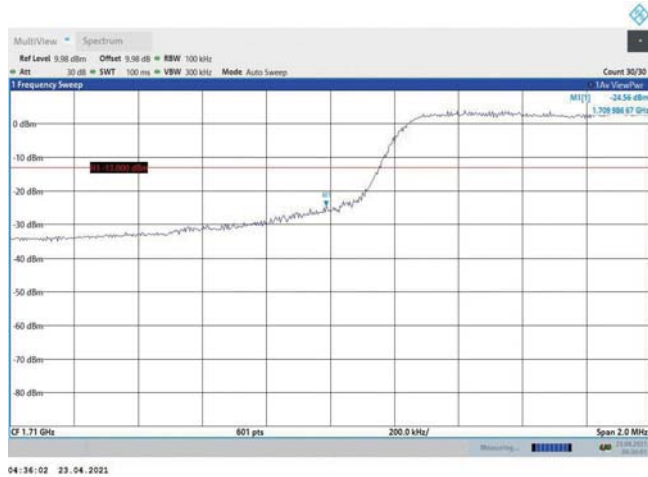
Band4-5MHz-QPSK-19975-25RB#0
