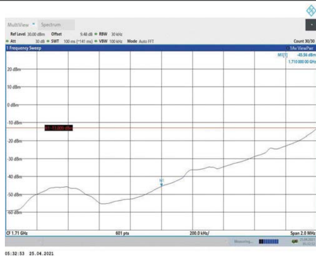
Band4-1.4MHz-16QAM-19957-1RB#5
