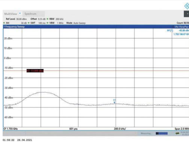
Band4-10MHz-16QAM-20350-1RB#0
