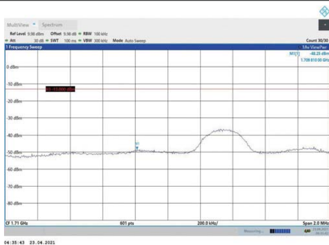
Band4-5MHz-QPSK-19975-1RB#24
