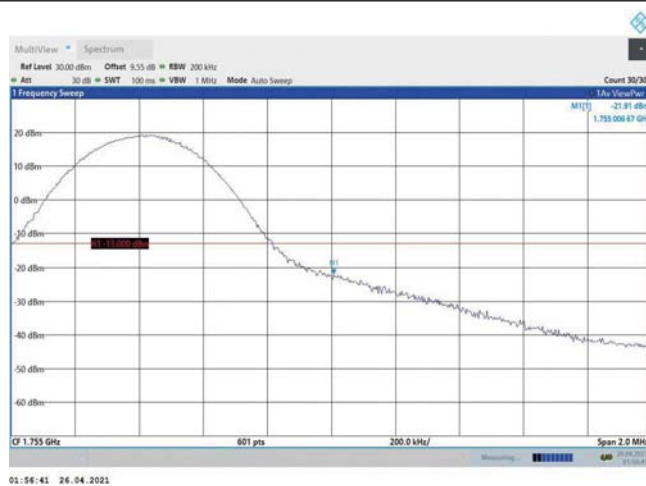
Band4-10MHz-16QAM-20350-1RB#49
