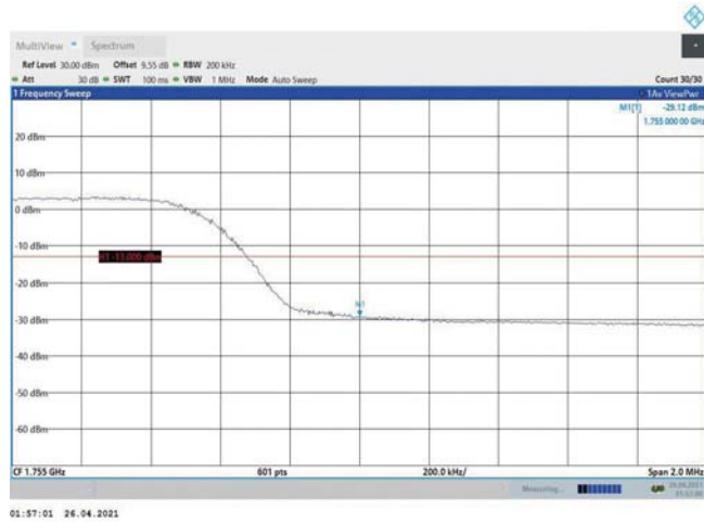
Band4-10MHz-16QAM-20350-50RB#0
