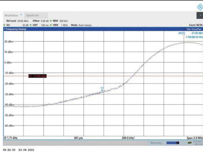
Band4-15MHz-QPSK-20025-1RB#0
