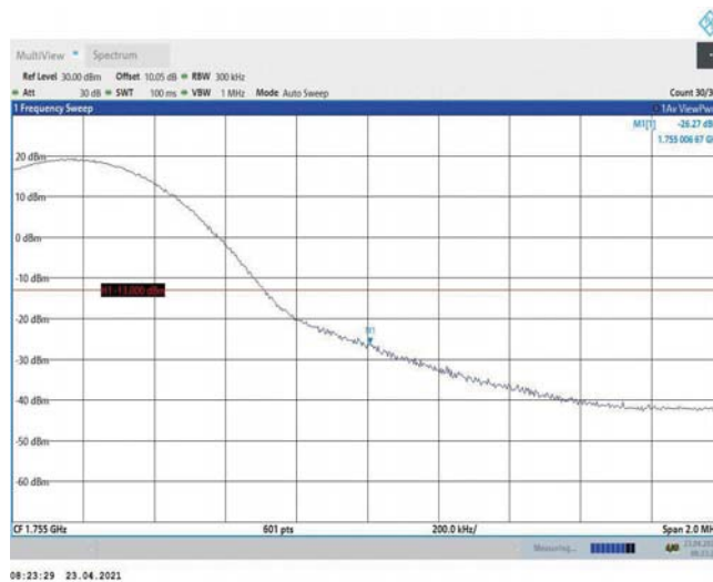
Band4-15MHz-16QAM-20325-1RB#74
