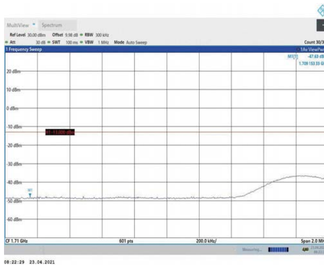
Band4-15MHz-16QAM-20025-1RB#74
