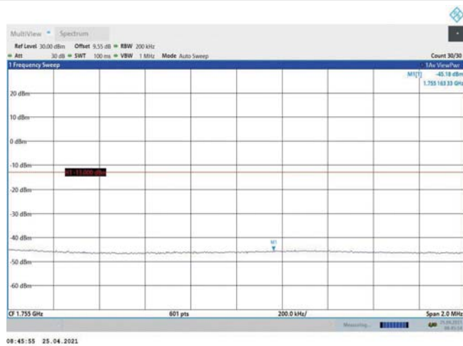
Band4-20MHz-QPSK-20300-1RB#0
