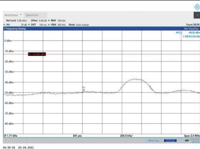
Band4-5MHz-16QAM-19975-1RB#24
