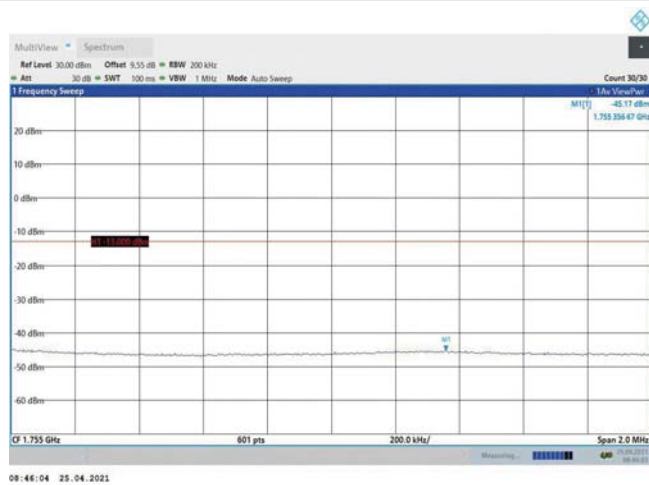
Band4-20MHz-16QAM-20300-1RB#0
