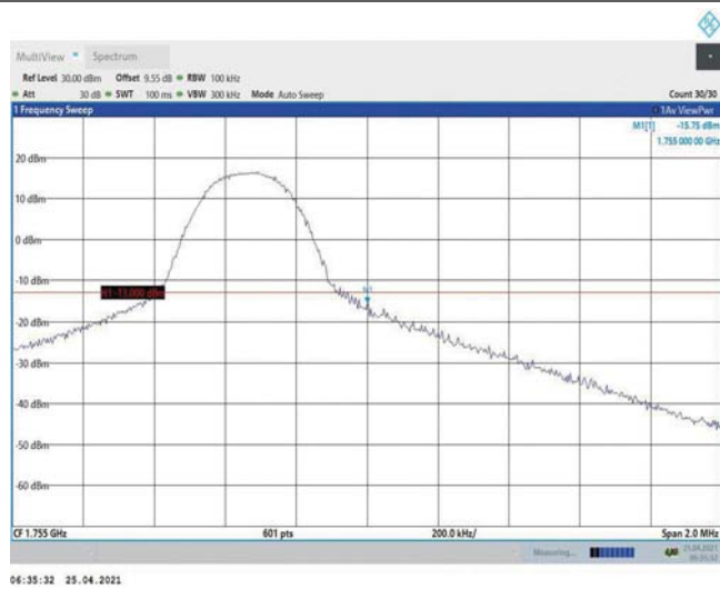
Band4-5MHz-16QAM-20375-1RB#24
