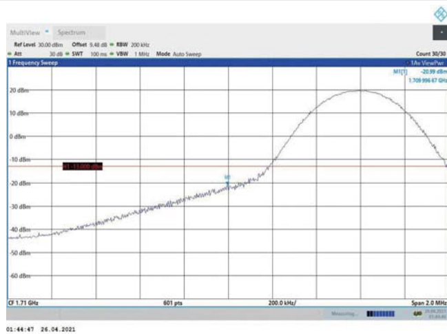
Band4-10MHz-16QAM-20000-1RB#0
