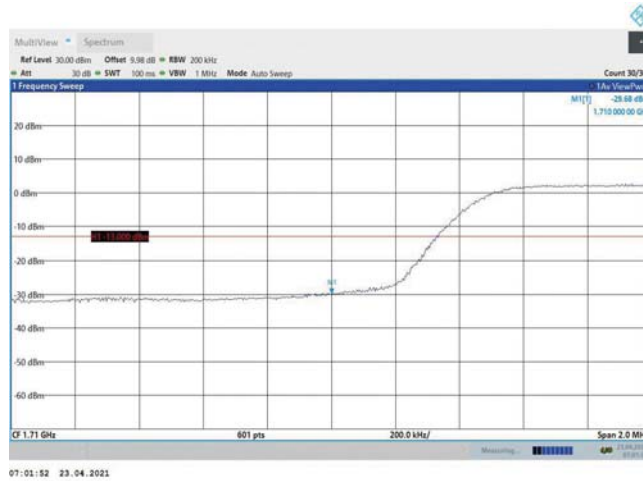
Band4-10MHz-16QAM-20000-50RB#0
