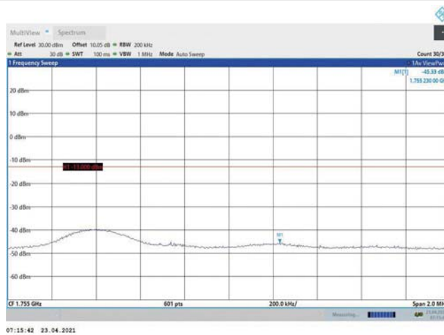
Band4-10MHz-16QAM-20350-1RB#0
