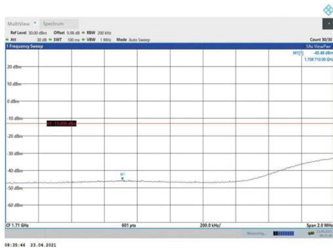
Band4-20MHz-16QAM-20050-1RB#99
