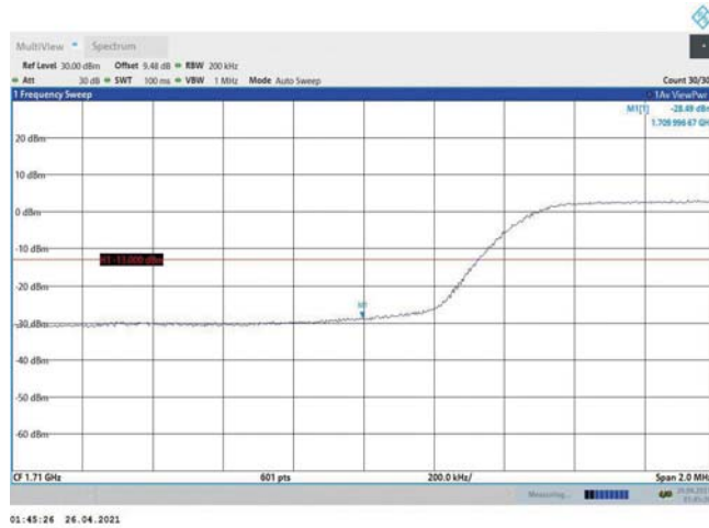
Band4-10MHz-16QAM-20000-50RB#0
