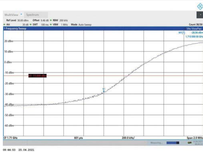
Band4-20MHz-16QAM-20050-1RB#0
