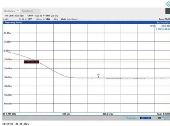
Band4-20MHz-16QAM-20300-100RB#0
