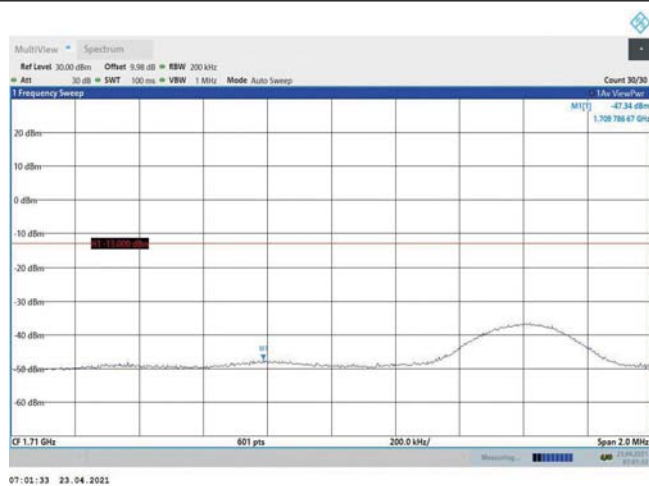
Band4-10MHz-16QAM-20000-1RB#49
