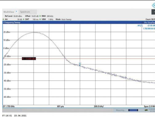
Band4-10MHz-16QAM-20350-1RB#49
