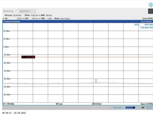
Band4-20MHz-QPSK-20300-1RB#0
