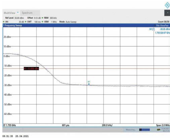
Band4-15MHz-16QAM-20325-75RB#0
