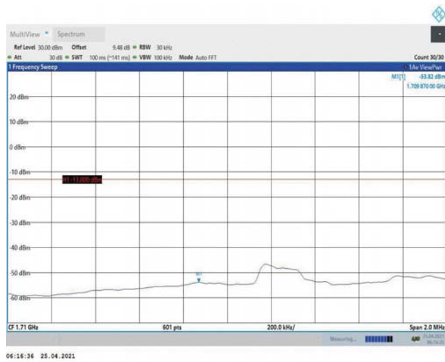
Band4-3MHz-16QAM-19965-1RB#14
