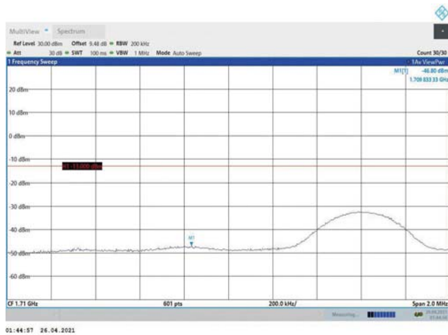
Band4-10MHz-QPSK-20000-1RB#49
