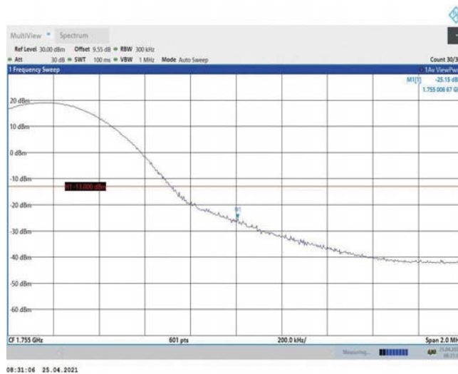
Band4-15MHz-QPSK-20325-1RB#74
