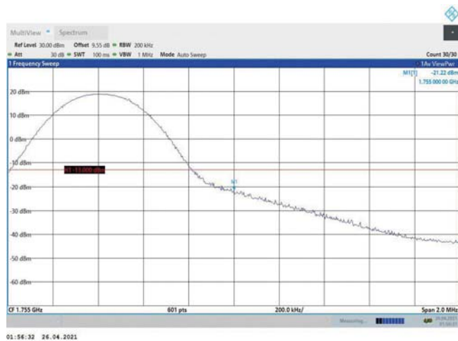
Band4-10MHz-QPSK-20350-1RB#49
