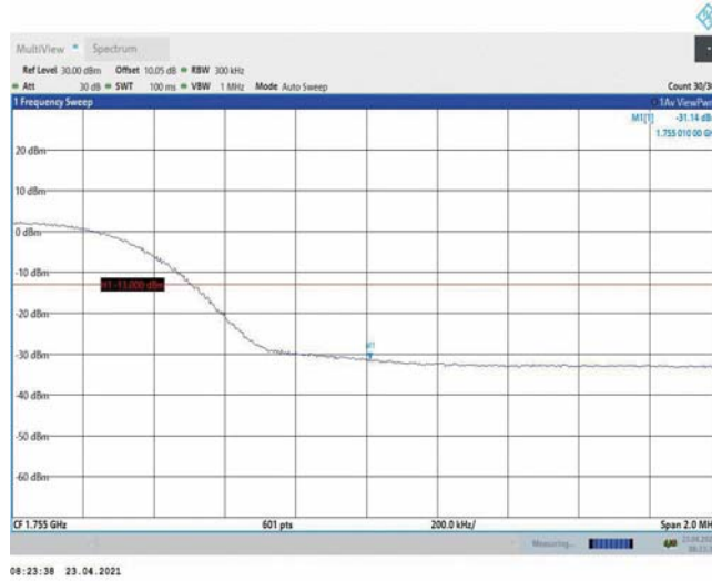
Band4-15MHz-QPSK-20325-75RB#0
