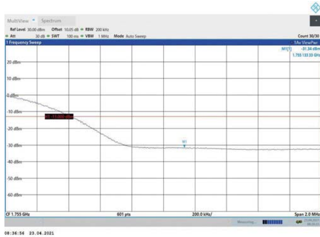
Band4-20MHz-QPSK-20300-100RB#0
