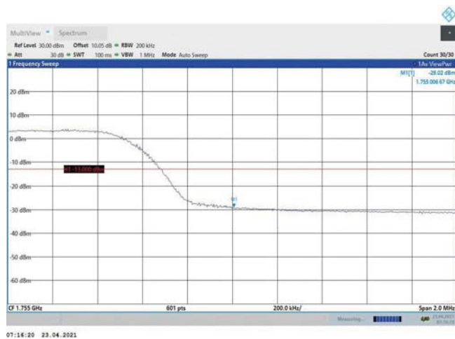
Band4-10MHz-16QAM-20350-50RB#0
