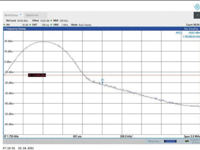
Band4-10MHz-QPSK-20350-1RB#49
