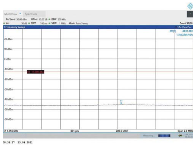
Band4-20MHz-16QAM-20300-1RB#0
