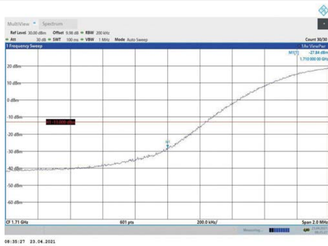
Band4-20MHz-16QAM-20050-1RB#0
