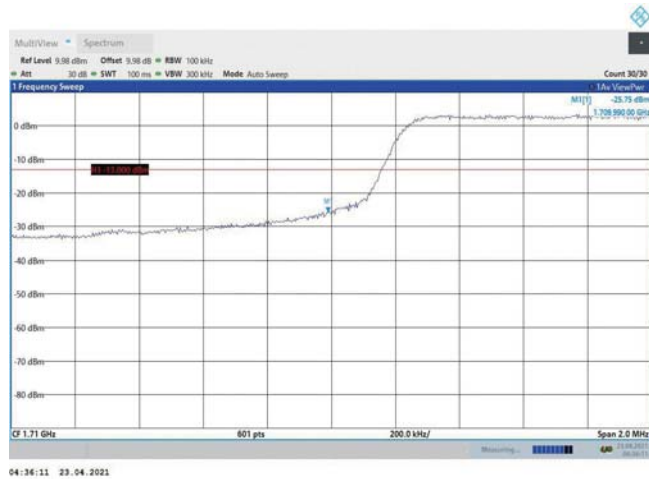
Band4-5MHz-16QAM-19975-25RB#0
