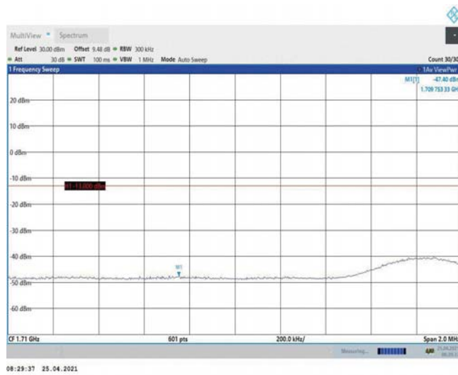
Band4-15MHz-16QAM-20025-1RB#74
