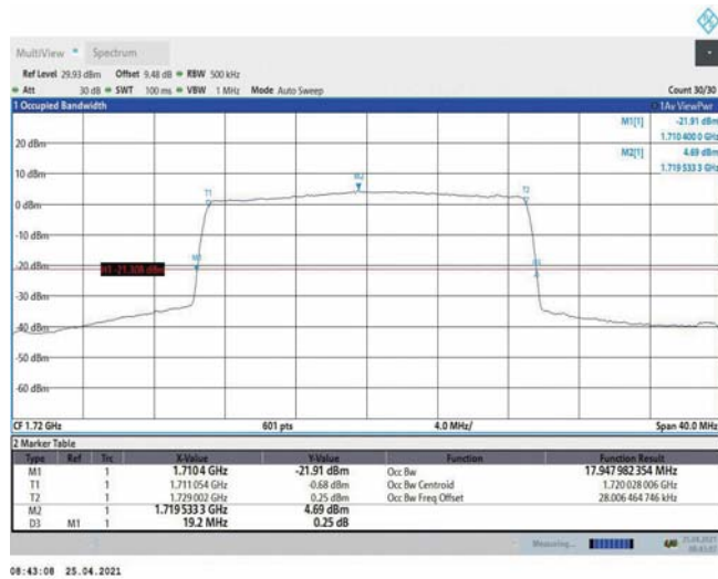
Band4-20MHz-QPSK-20050-100RB#0-17.948
