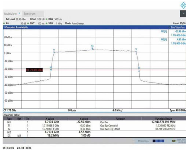
Band4-20MHz-QPSK-20050-100RB#0-17.945
