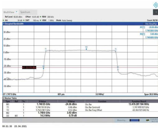
Band4-15MHz-QPSK-20325-75RB#0-13.476
