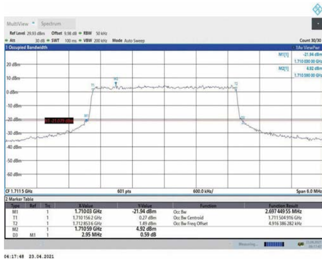
Band4-3MHz-16QAM-19965-15RB#0-2.697
