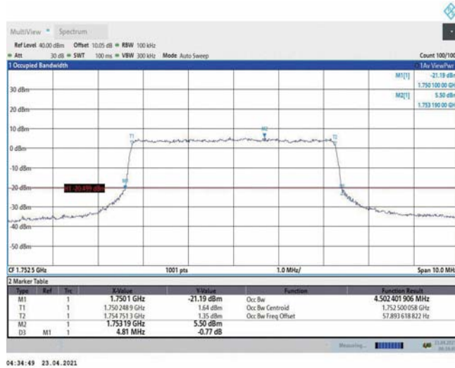
Band4-5MHz-QPSK-20375-25RB#0-4.502
