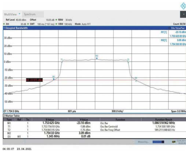
Band4-1.4MHz-16QAM-20393-6RB#0-1.087
