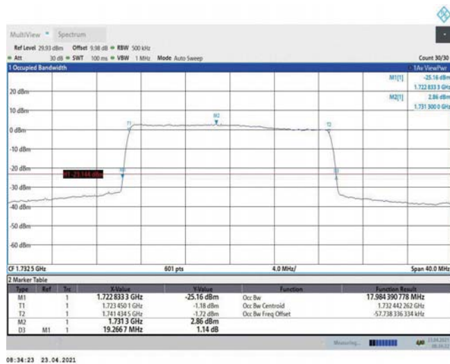
Band4-20MHz-QPSK-20175-100RB#0-17.984
