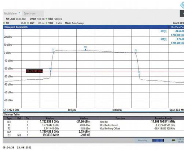
Band4-20MHz-16QAM-20175-100RB#0-17.999
