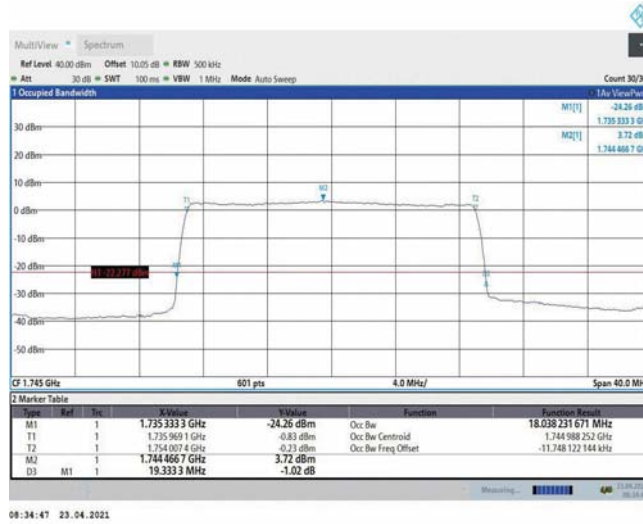
Band4-20MHz-QPSK-20300-100RB#0-18.038
