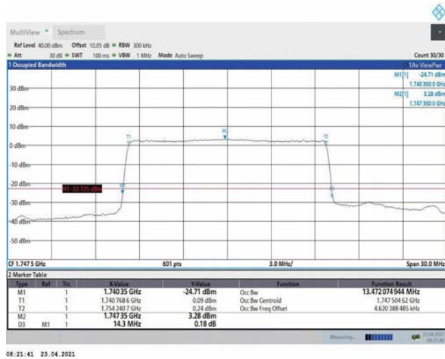
Band4-15MHz-16QAM-20325-75RB#0-13.472
