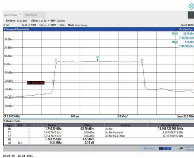
Band4-15MHz-16QAM-20325-75RB#0-13.468
