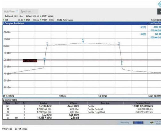
Band4-20MHz-16QAM-20050-100RB#0-17.941
