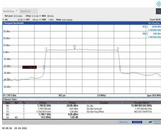
Band4-15MHz-QPSK-20325-75RB#0-13.485
