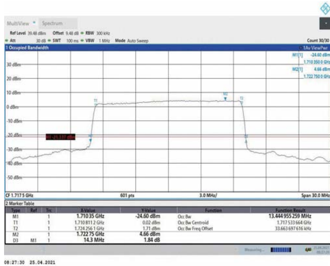
Band4-15MHz-16QAM-20025-75RB#0-13.445
