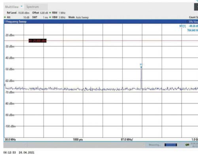
Band7-20MHz-16QAM-21350-1RB#0-Range1:30~1000MHz
