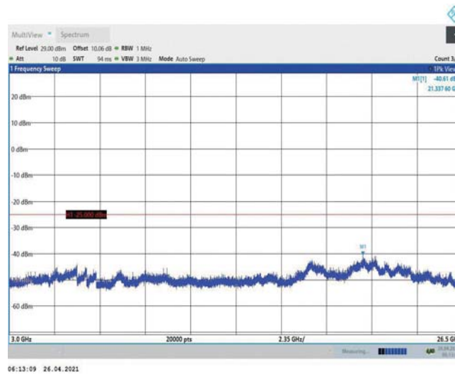
Band7-20MHz-16QAM-21350-1RB#0-Range3:3000~26500MHz
