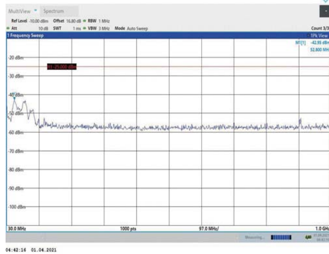
Band7-20MHz-16QAM-20850-1RB#0-Range1:30~1000MHz
