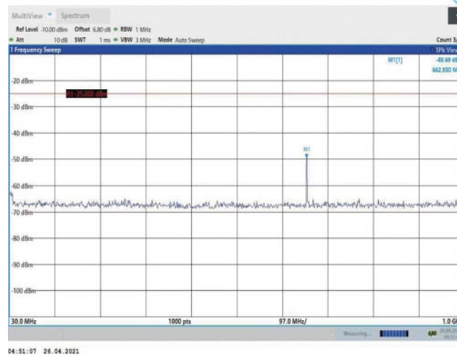
Band7-10MHz-16QAM-21100-1RB#0-Range1:30~1000MHz
