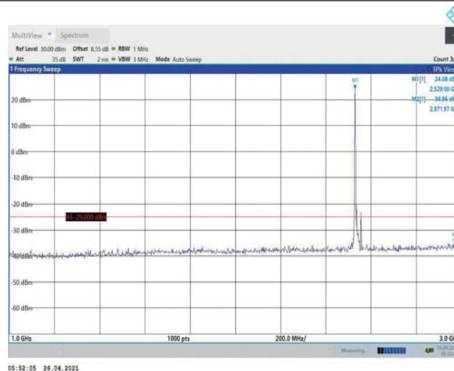
Band7-15MHz-QPSK-21100-1RB#0-Range2:1000~3000MHz
