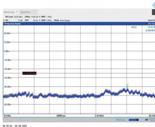
Band7-10MHz-16QAM-20800-1RB#0-Range3:3000~26500MHz
