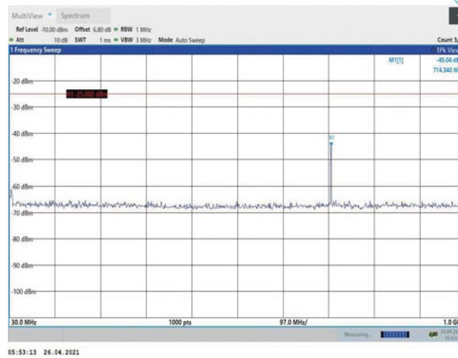
Band7-15MHz-16QAM-21375-1RB#0-Range1:30~1000MHz
