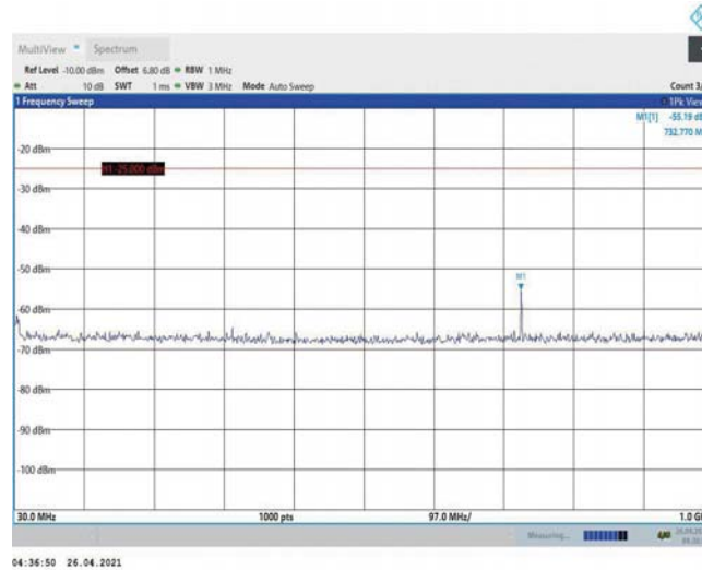
Band7-5MHz-QPSK-21425-1RB#0-Range1:30~1000MHz
