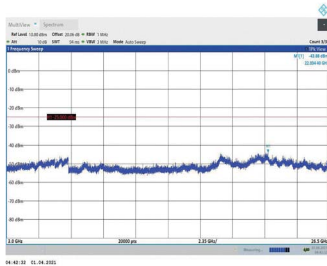
Band7-20MHz-16QAM-20850-1RB#0-Range3:3000~26500MHz
