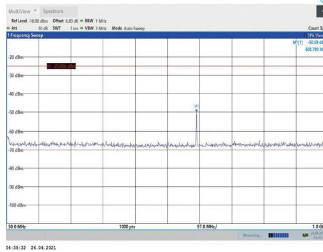
Band7-5MHz-16QAM-20775-1RB#0-Range1:30~1000MHz
