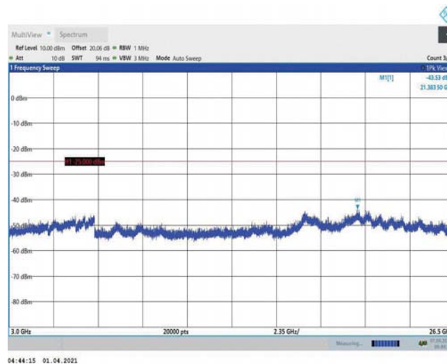
Band7-20MHz-16QAM-21350-1RB#0-Range3:3000~26500MHz
