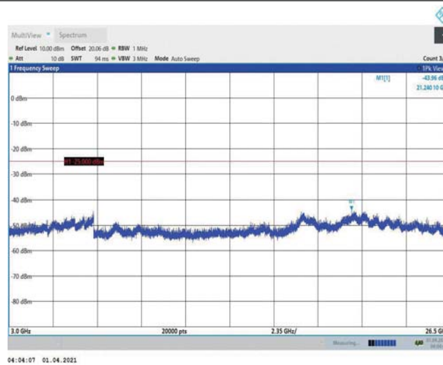
Band7-10MHz-16QAM-20800-1RB#0-Range3:3000~26500MHz
