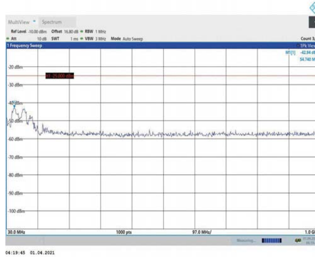
Band7-15MHz-QPSK-21100-1RB#0-Range1:30~1000MHz
