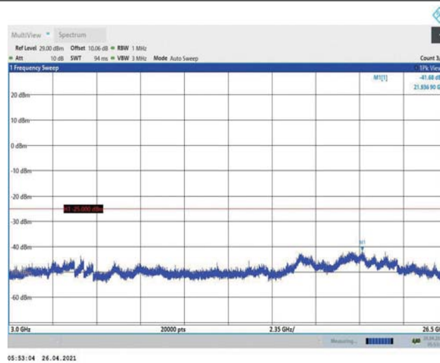
Band7-15MHz-QPSK-21375-1RB#0-Range3:3000~26500MHz
