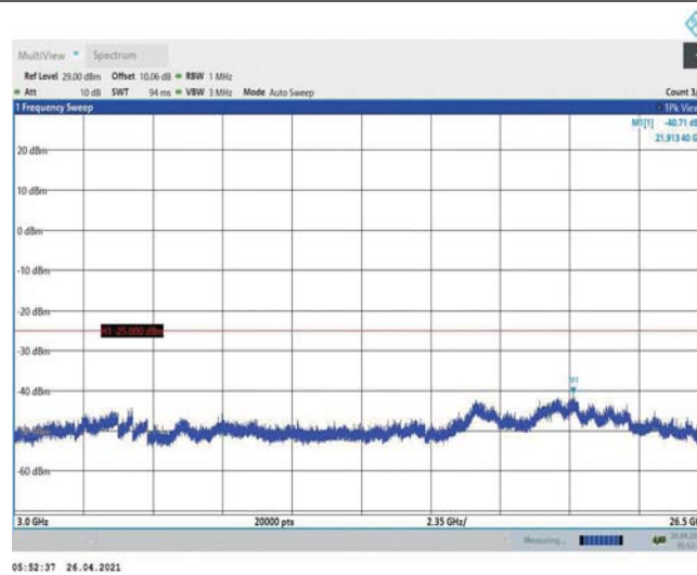
Band7-15MHz-16QAM-21100-1RB#0-Range3:3000~26500MHz
