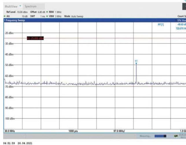
Band7-10MHz-16QAM-21400-1RB#0-Range1:30~1000MHz
