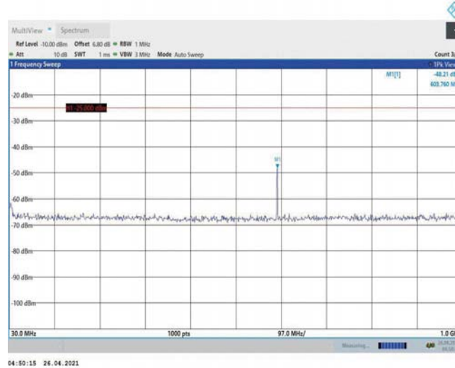
Band7-10MHz-16QAM-20800-1RB#0-Range1:30~1000MHz
