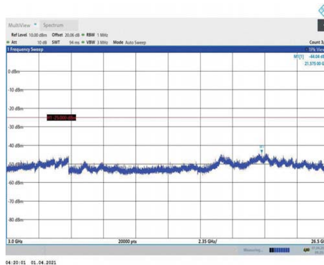
Band7-15MHz-QPSK-21100-1RB#0-Range3:3000~26500MHz
