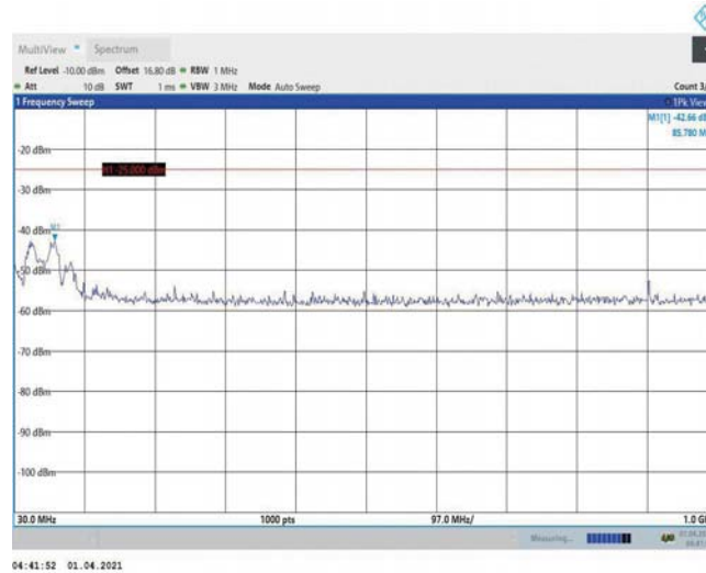
Band7-20MHz-QPSK-20850-1RB#0-Range1:30~1000MHz
