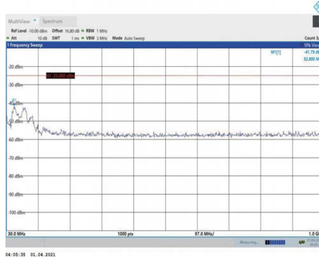
Band7-10MHz-16QAM-21400-1RB#0-Range1:30~1000MHz
