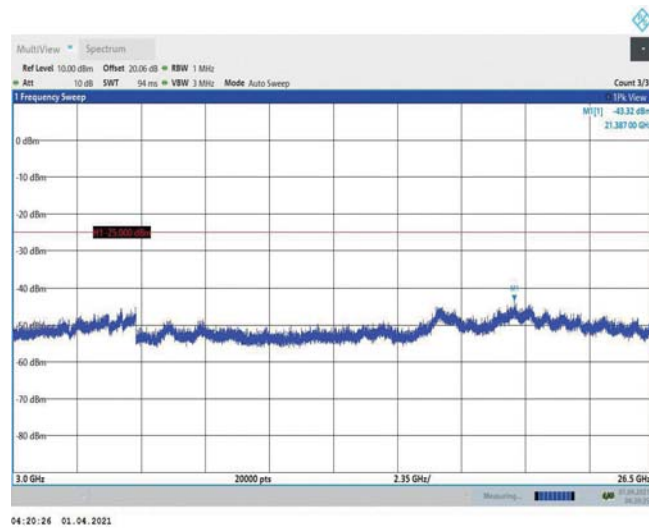
Band7-15MHz-16QAM-21100-1RB#0-Range3:3000~26500MHz
