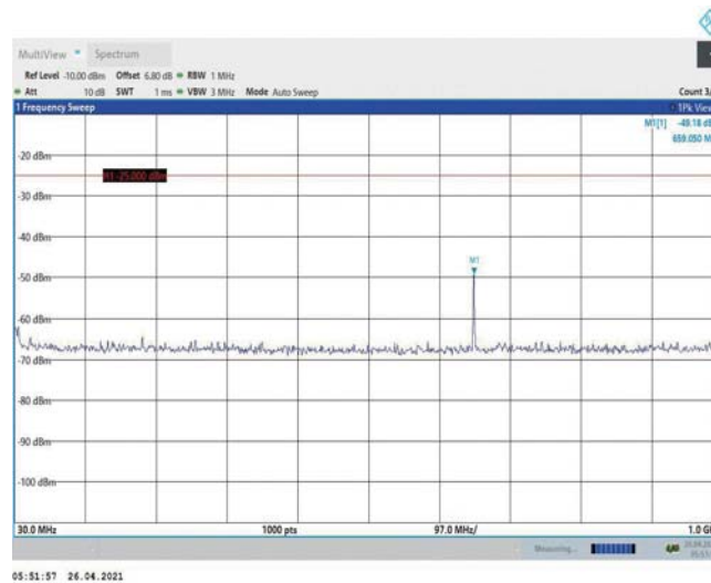
Band7-15MHz-QPSK-21100-1RB#0-Range1:30~1000MHz
