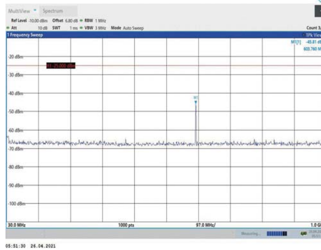
Band7-15MHz-16QAM-20825-1RB#0-Range1:30~1000MHz
