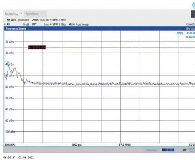
Band7-15MHz-QPSK-21375-1RB#0-Range1:30~1000MHz
