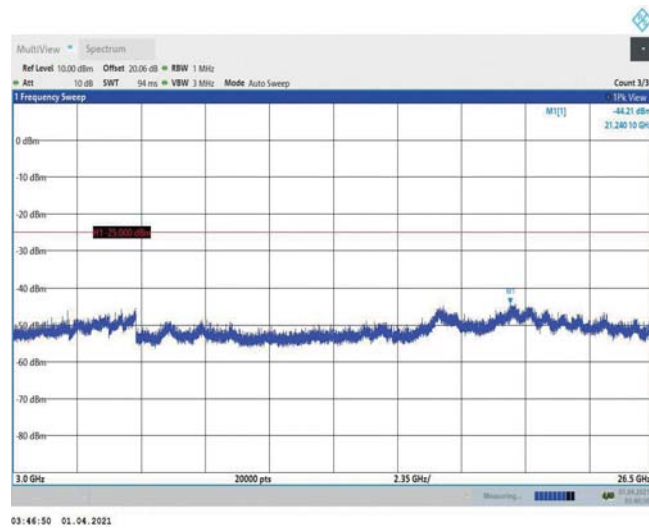
Band7-5MHz-16QAM-20775-1RB#0-Range3:3000~26500MHz
