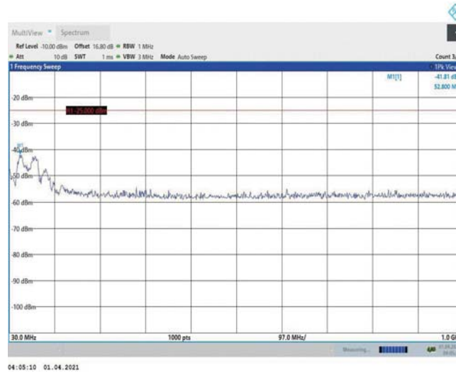
Band7-10MHz-QPSK-21400-1RB#0-Range1:30~1000MHz
