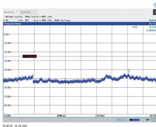
Band7-5MHz-16QAM-21425-1RB#0-Range3:3000~26500MHz
