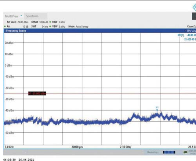
Band7-5MHz-16QAM-21100-1RB#0-Range3:3000~26500MHz
