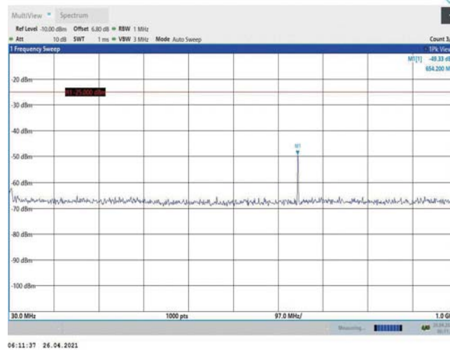
Band7-20MHz-QPSK-21100-1RB#0-Range1:30~1000MHz
