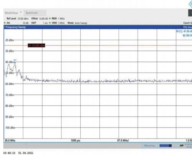
Band7-5MHz-QPSK-20775-1RB#0-Range1:30~1000MHz
