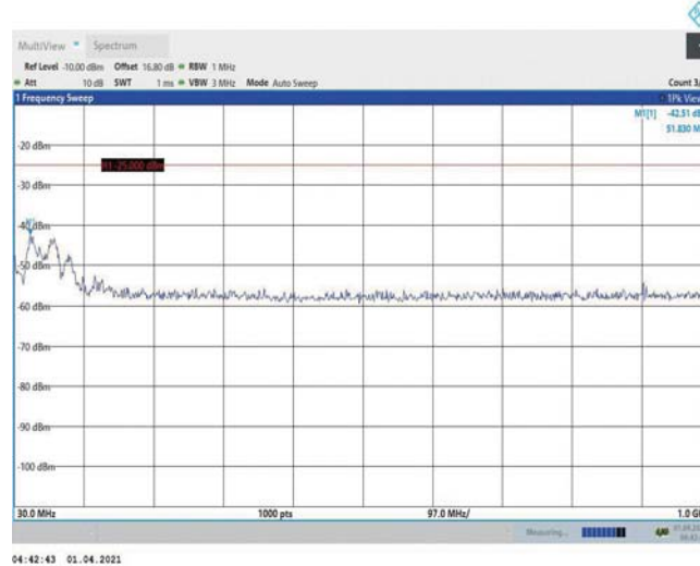
Band7-20MHz-QPSK-21100-1RB#0-Range1:30~1000MHz
