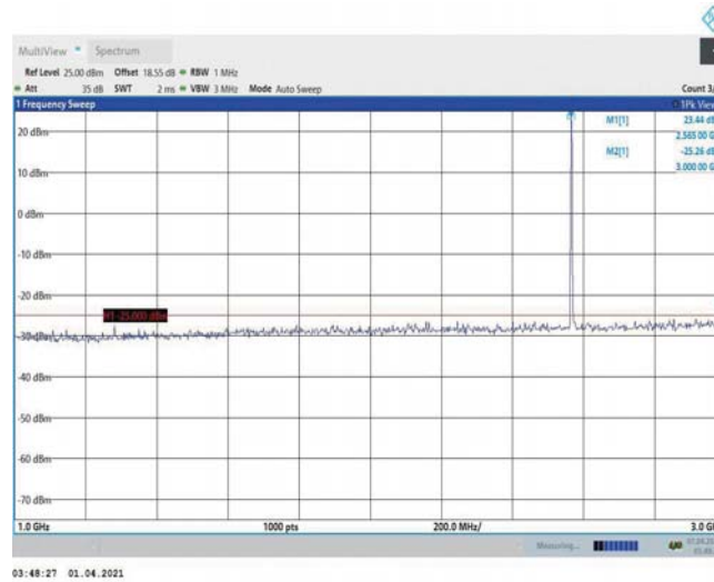
Band7-5MHz-16QAM-21425-1RB#0-Range2:1000~3000MHz
