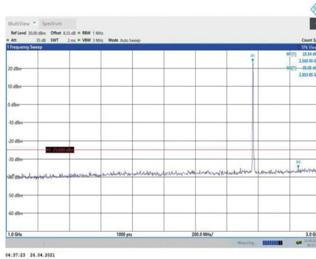
Band7-5MHz-16QAM-21425-1RB#0-Range2:1000~3000MHz
