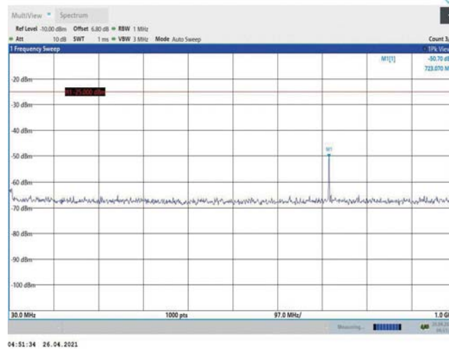
Band7-10MHz-QPSK-21400-1RB#0-Range1:30~1000MHz
