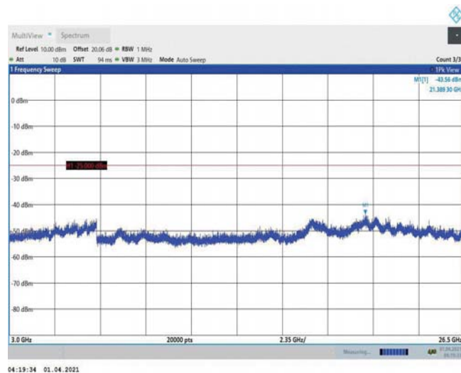
Band7-15MHz-16QAM-20825-1RB#0-Range3:3000~26500MHz
