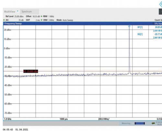
Band7-10MHz-16QAM-21400-1RB#0-Range2:1000~3000MHz
