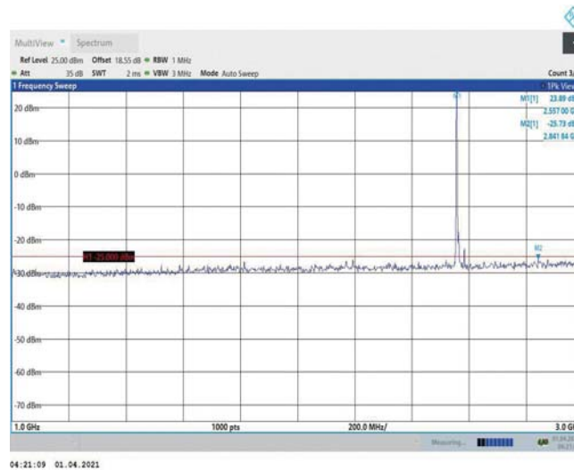
Band7-15MHz-16QAM-21375-1RB#0-Range2:1000~3000MHz
