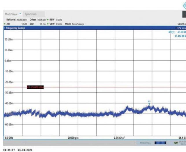
Band7-5MHz-16QAM-20775-1RB#0-Range3:3000~26500MHz
