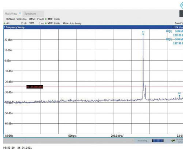
Band7-15MHz-16QAM-21100-1RB#0-Range2:1000~3000MHz
