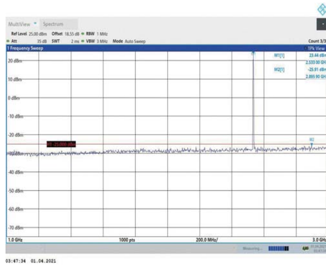
Band7-5MHz-16QAM-21100-1RB#0-Range2:1000~3000MHz
