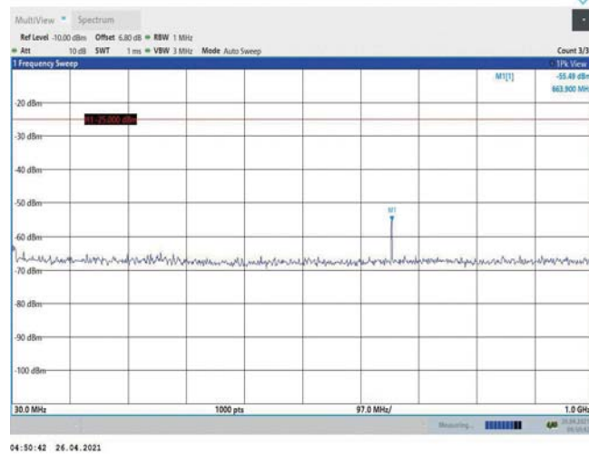
Band7-10MHz-QPSK-21100-1RB#0-Range1:30~1000MHz
