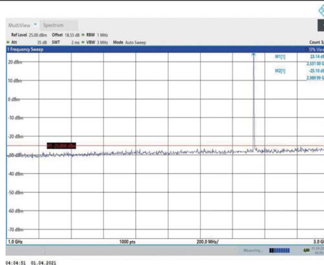
Band7-10MHz-16QAM-21100-1RB#0-Range2:1000~3000MHz
