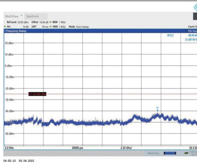
Band7-10MHz-16QAM-21400-1RB#0-Range3:3000~26500MHz
