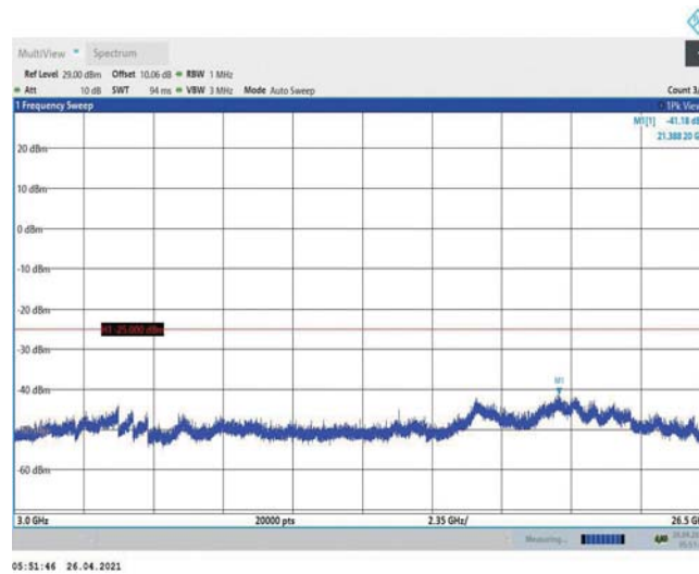
Band7-15MHz-16QAM-20825-1RB#0-Range3:3000~26500MHz
