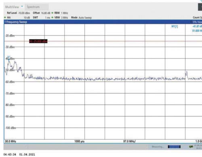
Band7-20MHz-QPSK-21350-1RB#0-Range1:30~1000MHz
