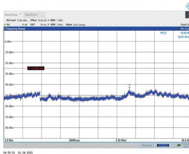
Band7-10MHz-16QAM-21400-1RB#0-Range3:3000~26500MHz
