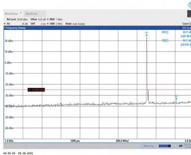
Band7-10MHz-16QAM-20800-1RB#0-Range2:1000~3000MHz
