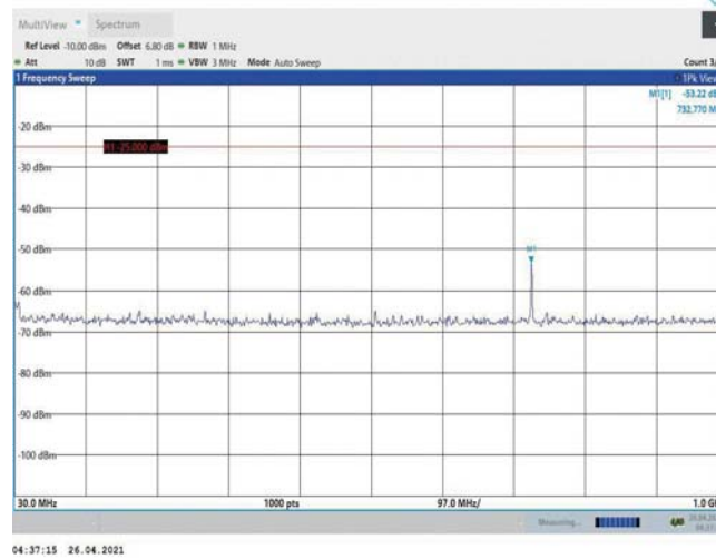
Band7-5MHz-16QAM-21425-1RB#0-Range1:30~1000MHz
