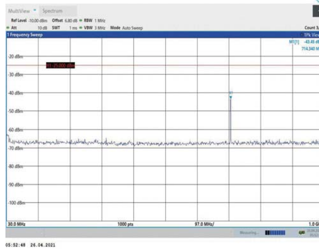
Band7-15MHz-QPSK-21375-1RB#0-Range1:30~1000MHz
