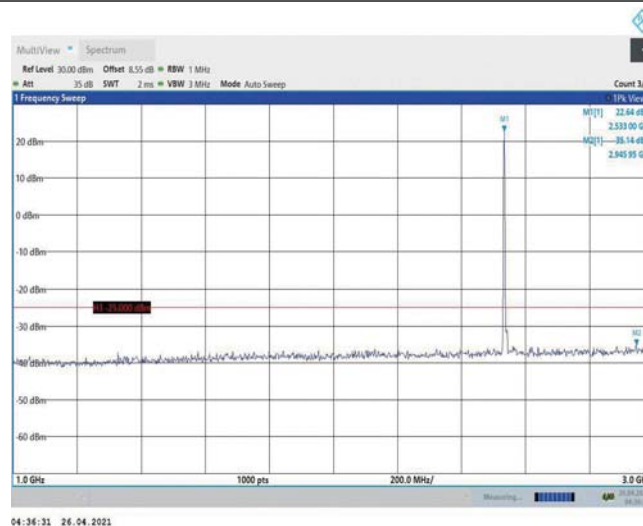
Band7-5MHz-16QAM-21100-1RB#0-Range2:1000~3000MHz
