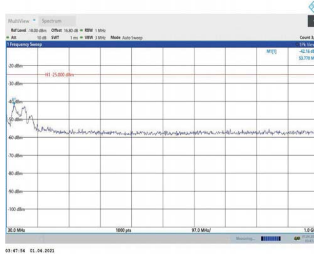
Band7-5MHz-QPSK-21425-1RB#0-Range1:30~1000MHz
