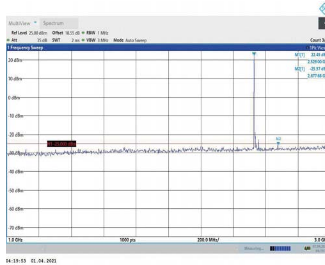
Band7-15MHz-QPSK-21100-1RB#0-Range2:1000~3000MHz
