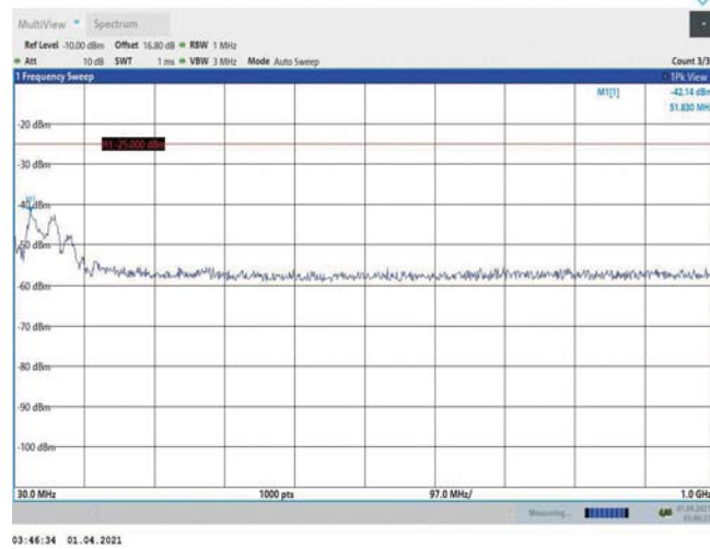
Band7-5MHz-16QAM-20775-1RB#0-Range1:30~1000MHz
