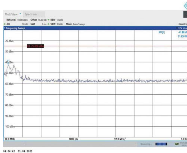
Band7-10MHz-16QAM-21100-1RB#0-Range1:30~1000MHz
