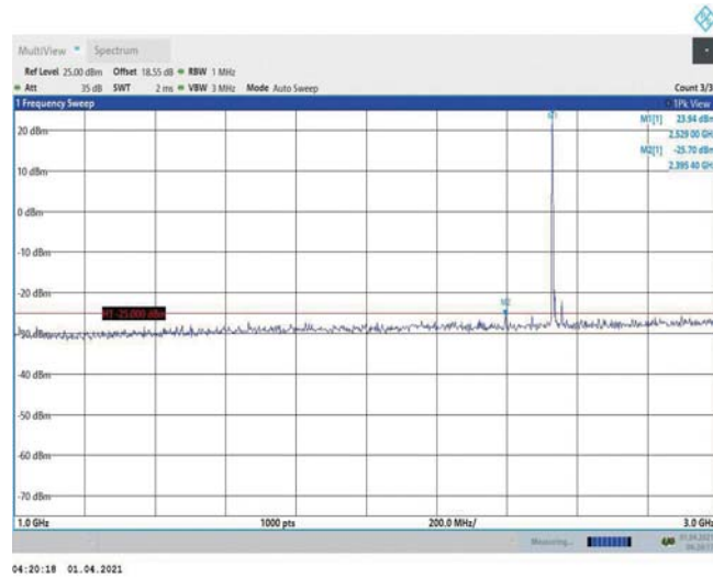
Band7-15MHz-16QAM-21100-1RB#0-Range2:1000~3000MHz
