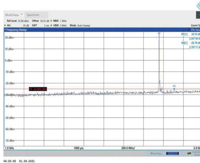
Band7-15MHz-QPSK-21375-1RB#0-Range2:1000~3000MHz
