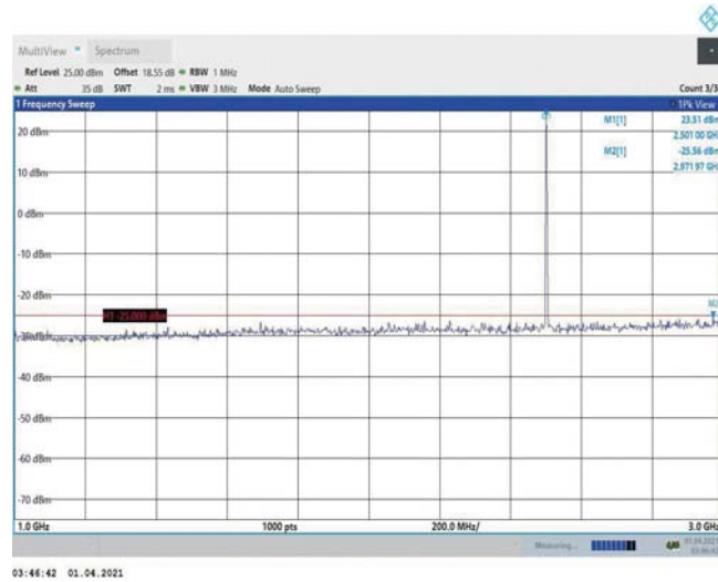
Band7-5MHz-16QAM-20775-1RB#0-Range2:1000~3000MHz
