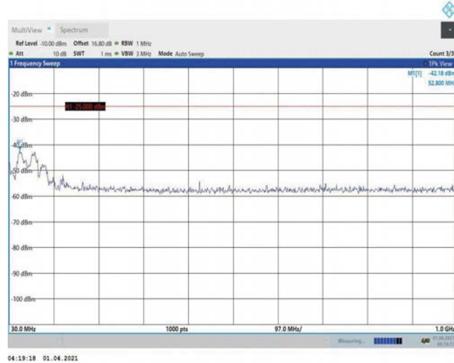
Band7-15MHz-16QAM-20825-1RB#0-Range1:30~1000MHz
