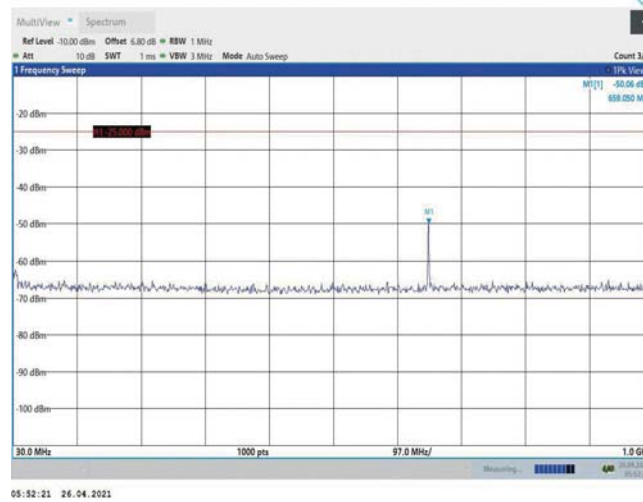
Band7-15MHz-16QAM-21100-1RB#0-Range1:30~1000MHz
