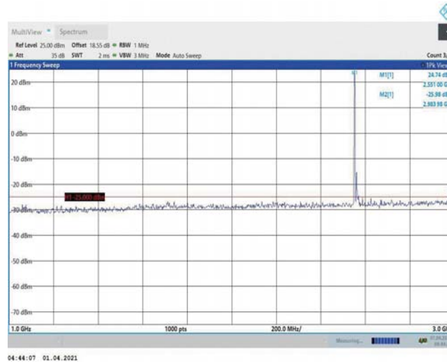
Band7-20MHz-16QAM-21350-1RB#0-Range2:1000~3000MHz
