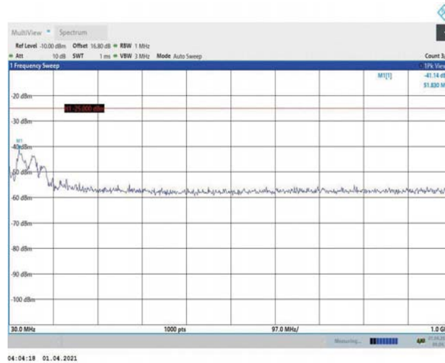
Band7-10MHz-QPSK-21100-1RB#0-Range1:30~1000MHz
