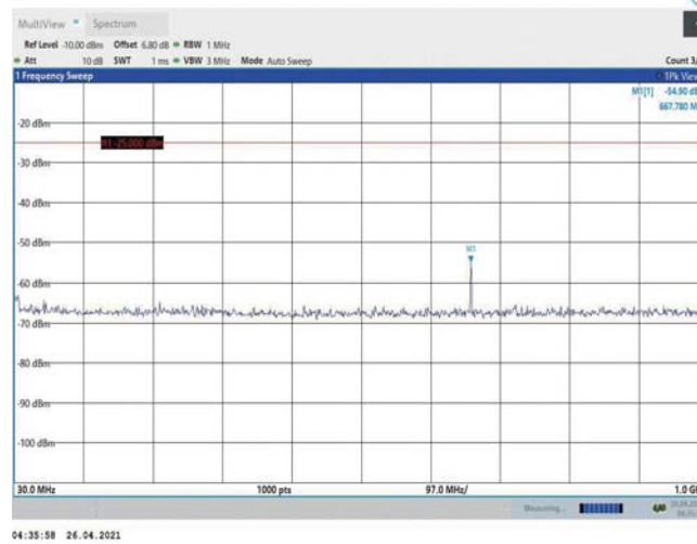
Band7-5MHz-QPSK-21100-1RB#0-Range1:30~1000MHz
