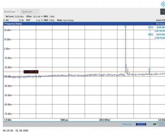
Band7-15MHz-16QAM-20825-1RB#0-Range2:1000~3000MHz
