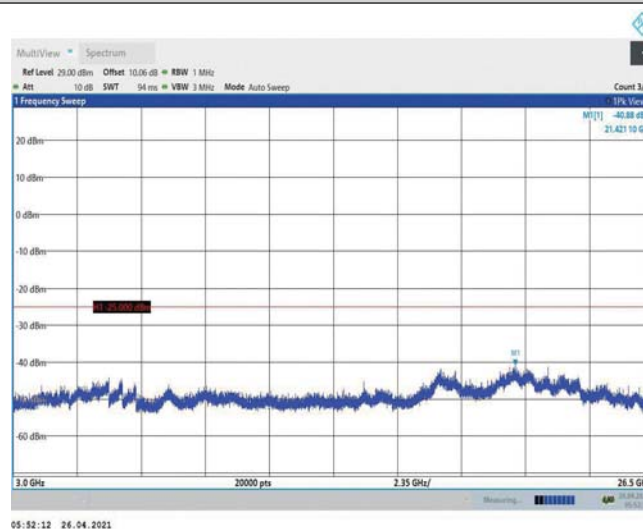
Band7-15MHz-QPSK-21100-1RB#0-Range3:3000~26500MHz
