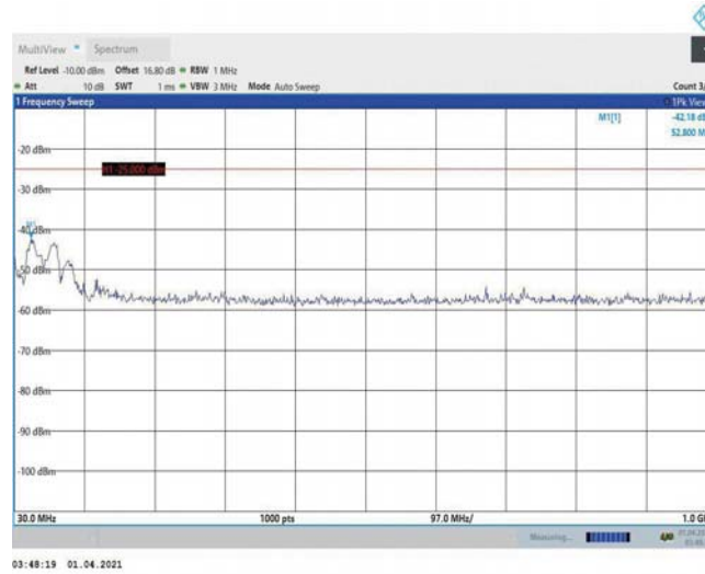
Band7-5MHz-16QAM-21425-1RB#0-Range1:30~1000MHz
