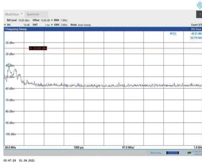
Band7-5MHz-16QAM-21100-1RB#0-Range1:30~1000MHz
