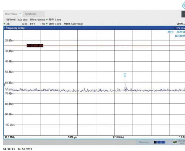
Band7-5MHz-16QAM-21100-1RB#0-Range1:30~1000MHz
