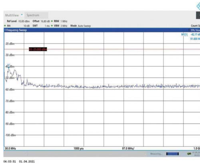
Band7-10MHz-16QAM-20800-1RB#0-Range1:30~1000MHz
