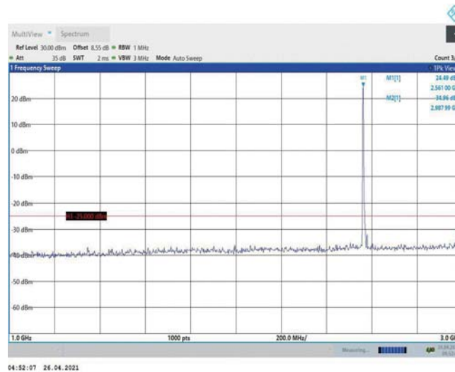
Band7-10MHz-16QAM-21400-1RB#0-Range2:1000~3000MHz
