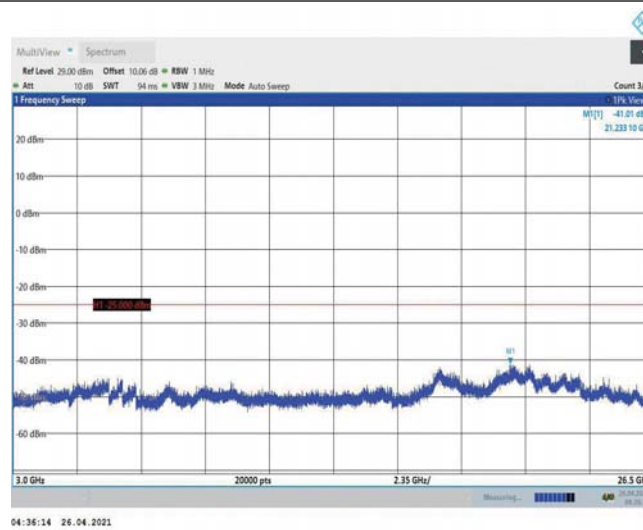
Band7-5MHz-QPSK-21100-1RB#0-Range3:3000~26500MHz
