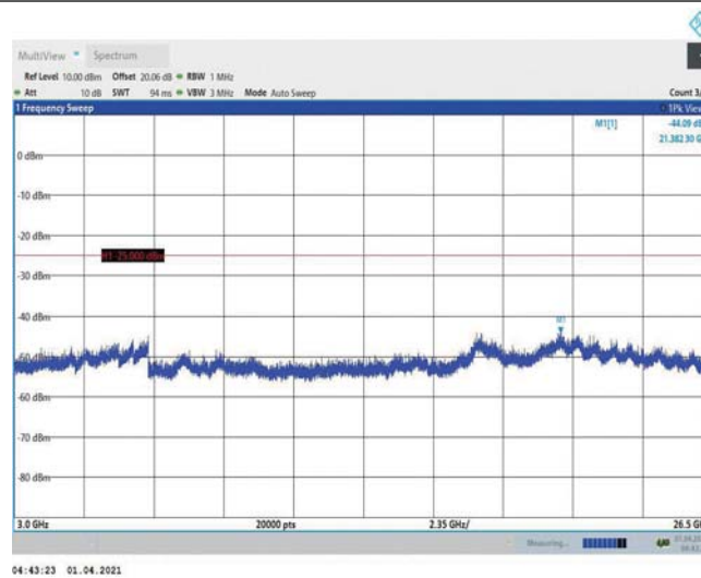
Band7-20MHz-16QAM-21100-1RB#0-Range3:3000~26500MHz
