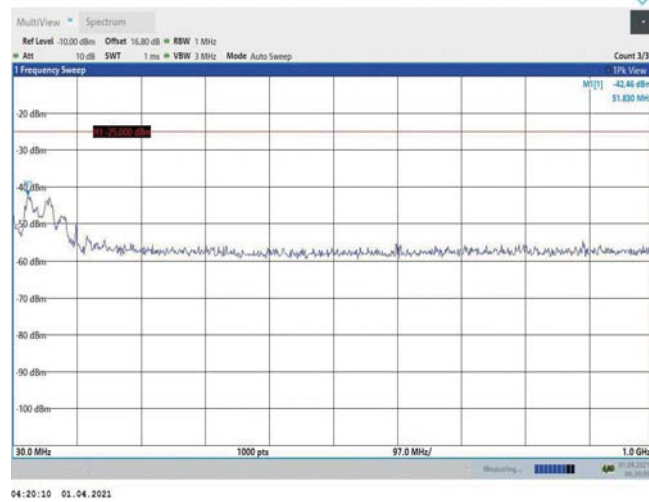
Band7-15MHz-16QAM-21100-1RB#0-Range1:30~1000MHz
