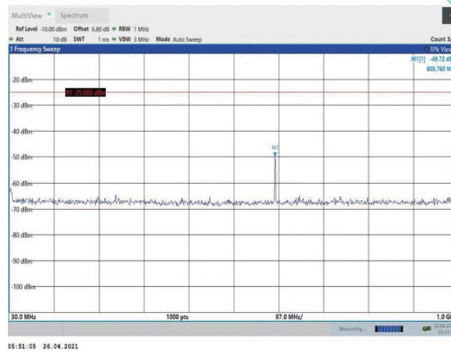
Band7-15MHz-QPSK-20825-1RB#0-Range1:30~1000MHz
