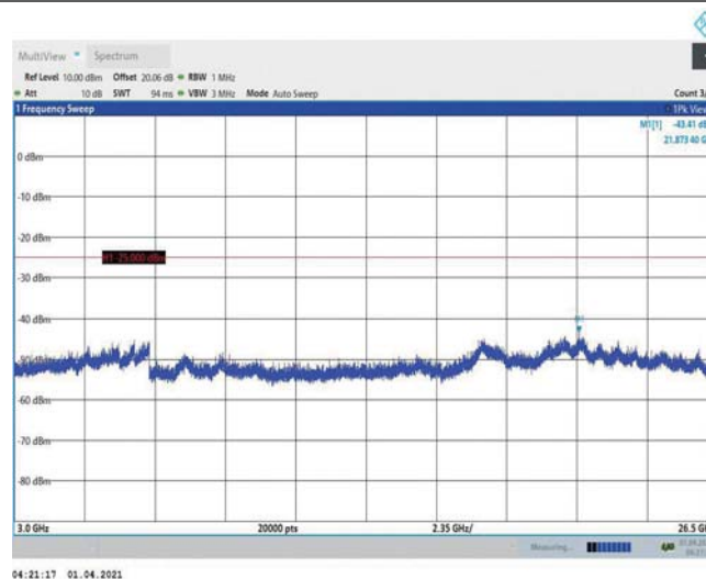
Band7-15MHz-16QAM-21375-1RB#0-Range3:3000~26500MHz
