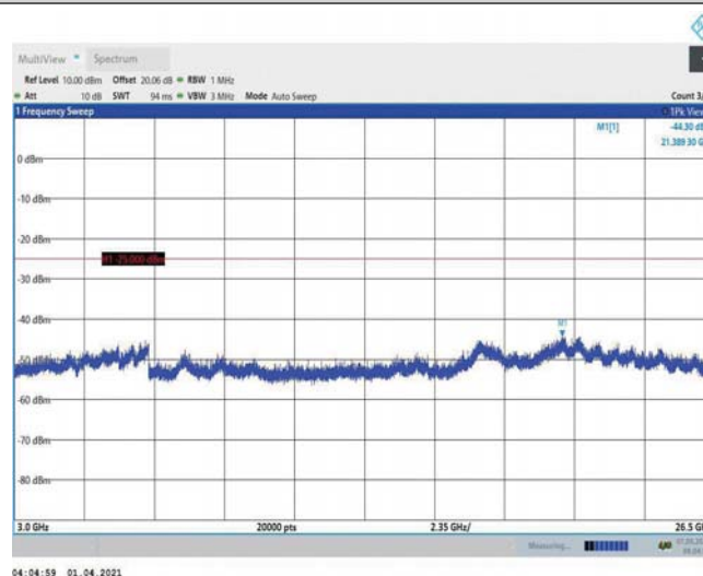
Band7-10MHz-16QAM-21100-1RB#0-Range3:3000~26500MHz
