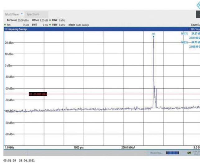
Band7-15MHz-16QAM-20825-1RB#0-Range2:1000~3000MHz
