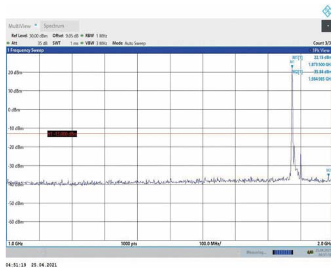
Band2-15MHz-QPSK-18900-1RB#0-Range2:1000~2000MHz
