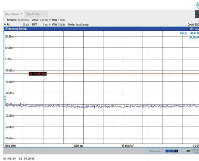
Band2-3MHz-QPSK-19185-1RB#0-Range1:30~1000MHz
