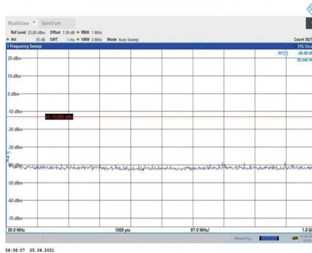
Band2-10MHz-16QAM-18650-1RB#0-Range1:30~1000MHz
