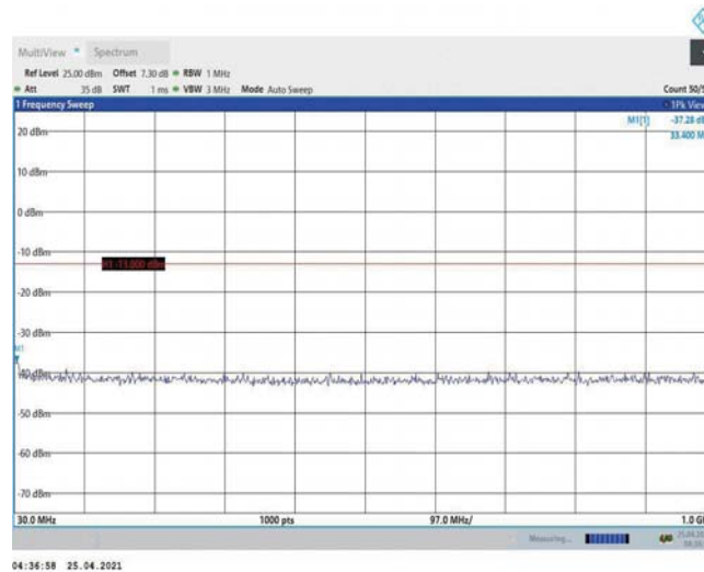
Band2-10MHz-QPSK-18900-1RB#0-Range1:30~1000MHz
